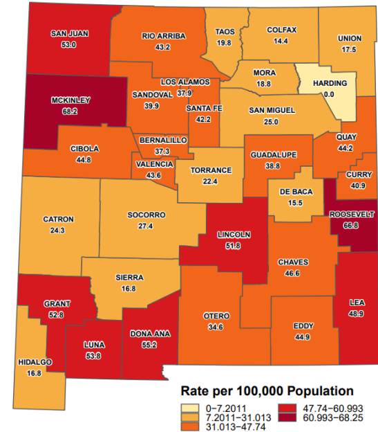
Average daily case rate per 100,000 population in the previous 7 days by New Mexico County (07/25/2022 - 07/31/2022)
