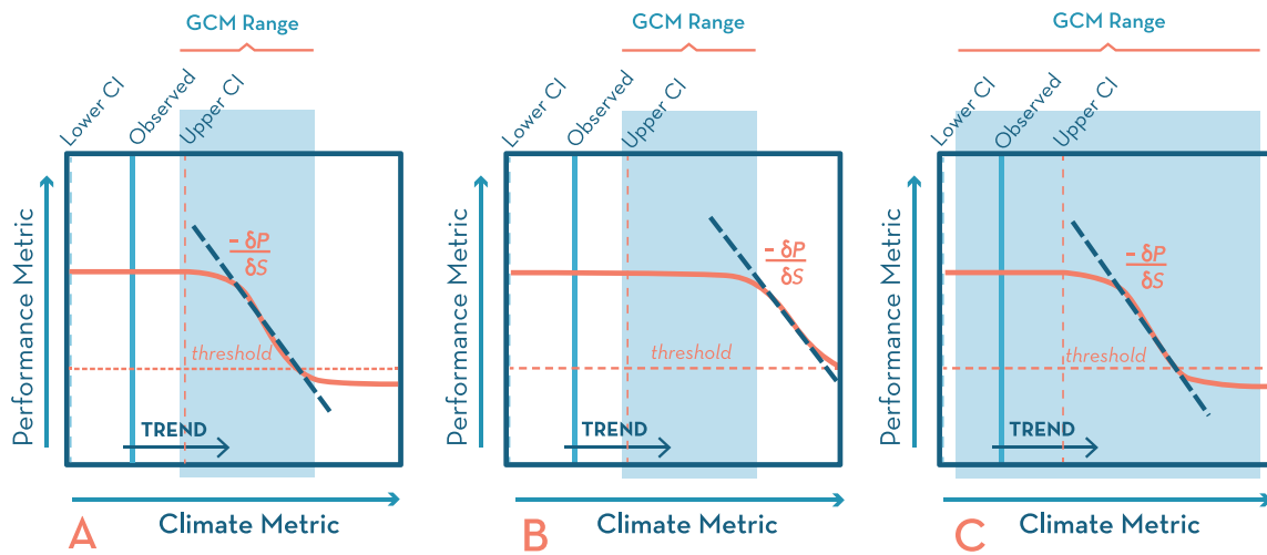
Figure 2.6. Examples of the climate and sensitivity components to assess the plausibility of surpassing a critical threshold.
