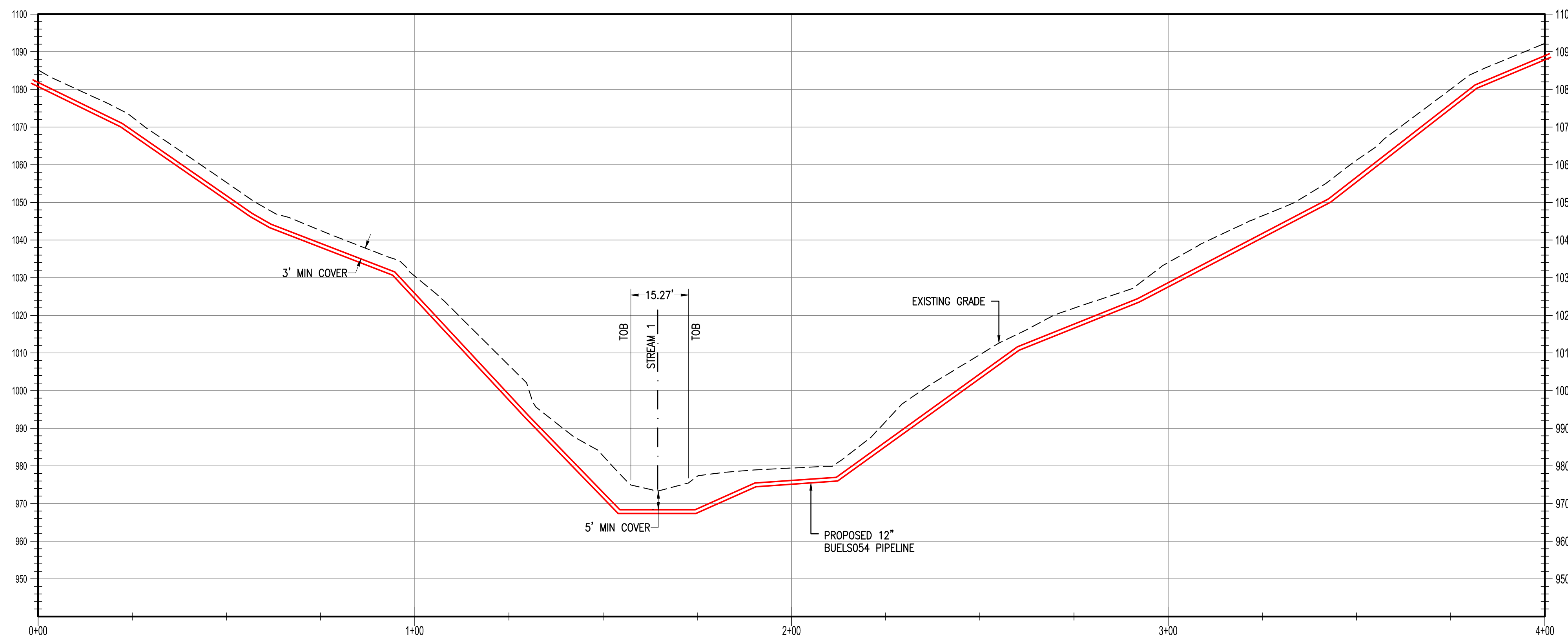
STREAM CROSSING PROFILE SCALE H: 1" = 20' SCALE V: 1" = 20'
