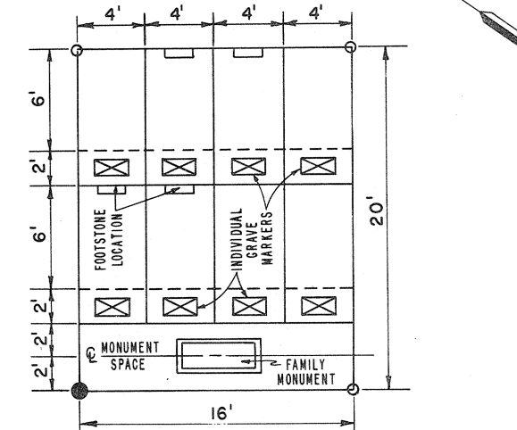
LOT AND GRAVE LAYOUT SCALE: 1" = 5'
