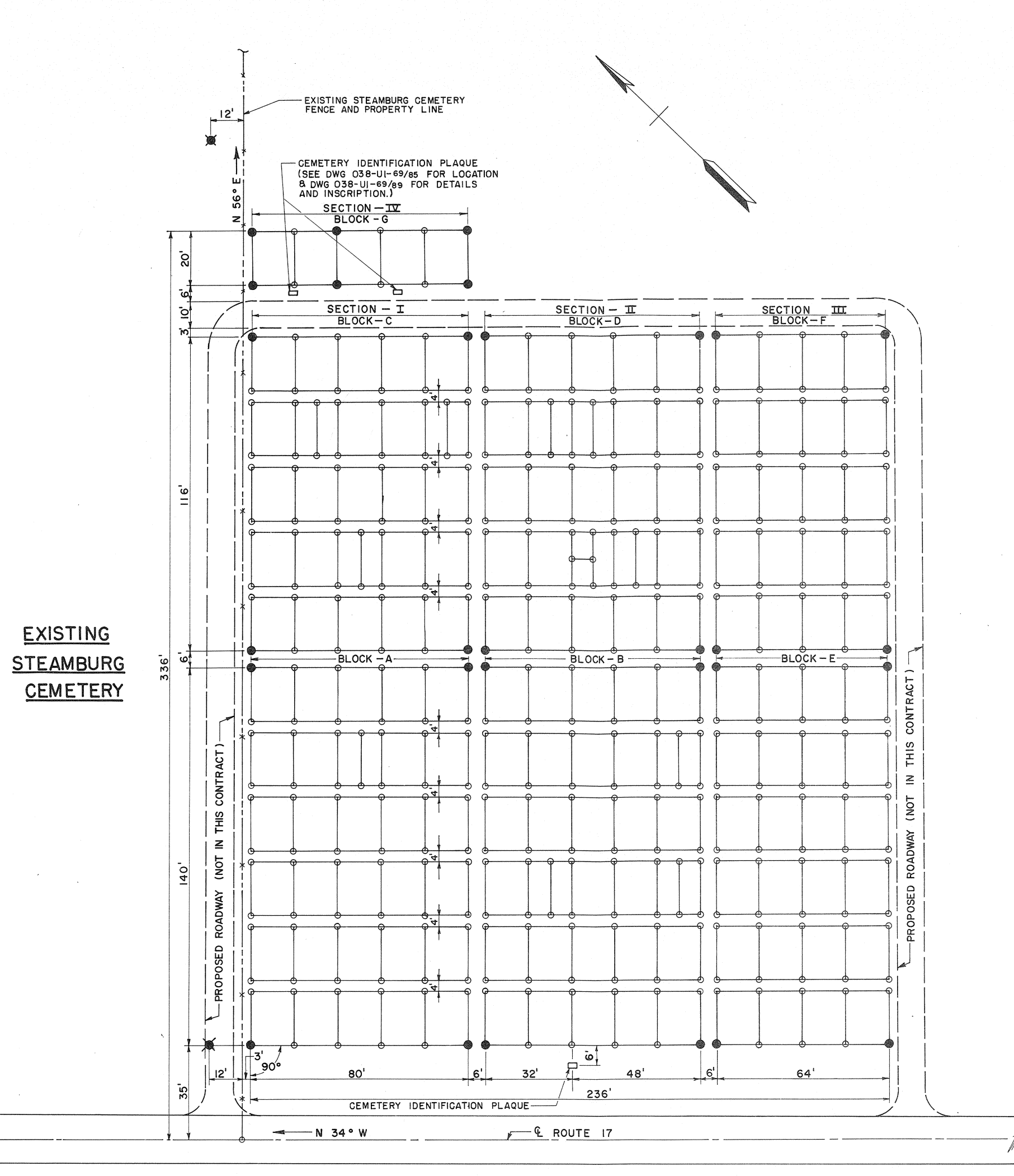
REINTERMENT SITE LAYOUT PLAN SCALE: 1" = 20'
