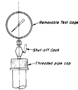
GAGE CONNECTION DETAIL
