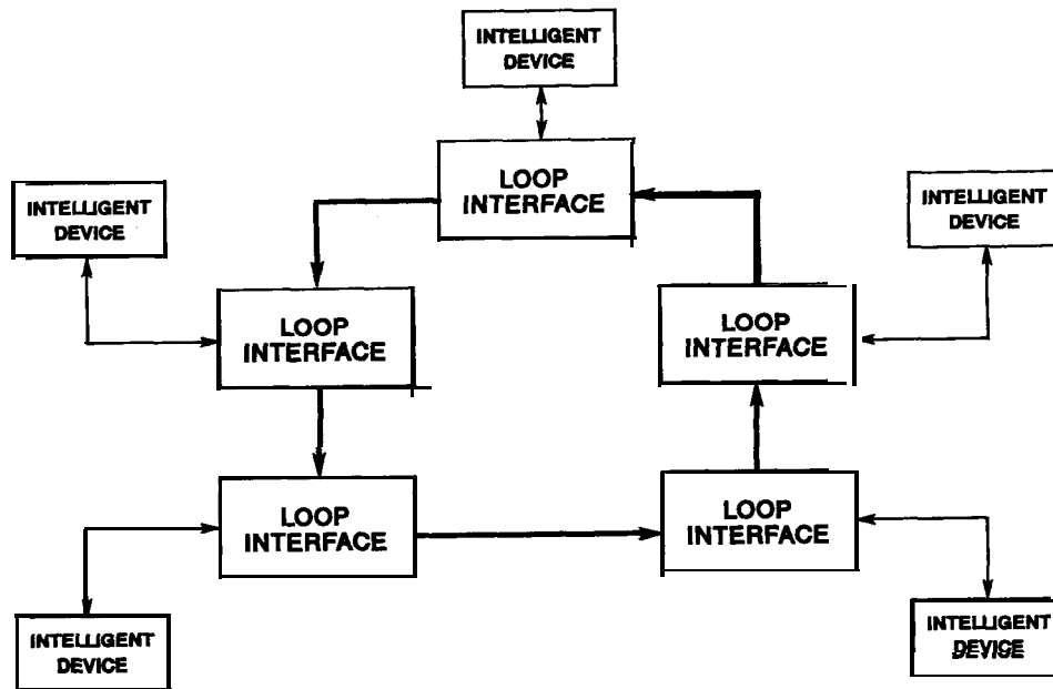
Figure 9-6. Loop Configuration
