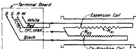
STRAIN METER
