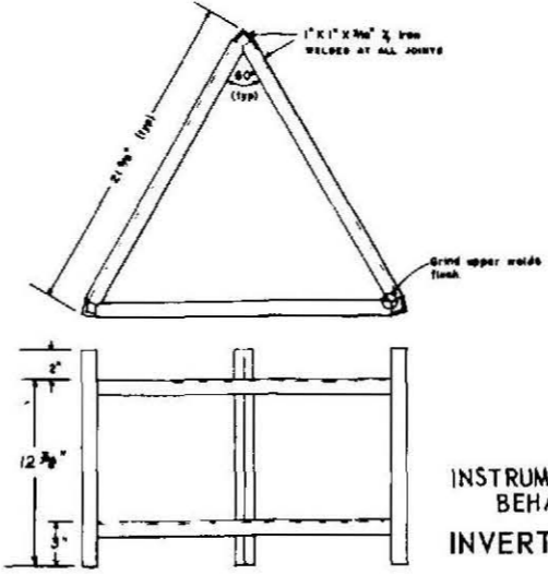
TANK SUPPORT FRAME (3) scale 1/4" = 1"
