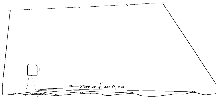
SECTION ALONG MONOLITH C-C
