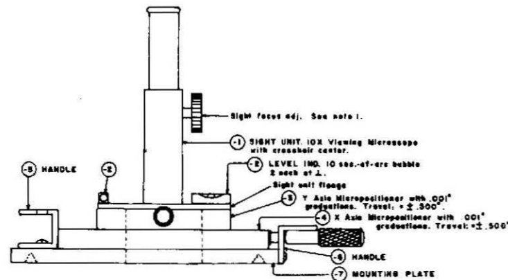
ELEVATION VIEW SIGHT ASSEMBLY 1 Required
