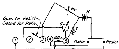
CARLSON BRIDGE
