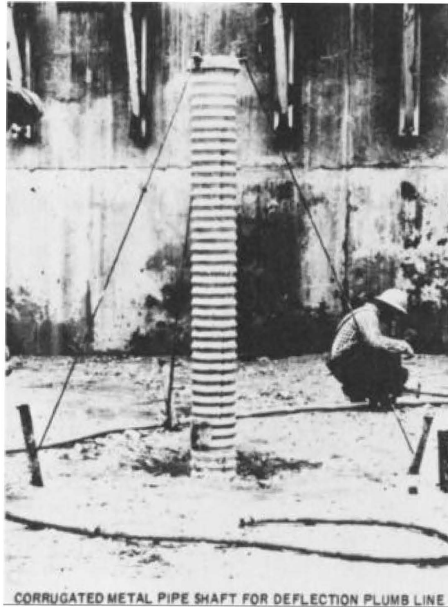
Figure 4-1 Corrugated metal pipe shaft at interface of a lift, and details of suspension plate attached on top of the shaft. (Prepared by CE-WES)
