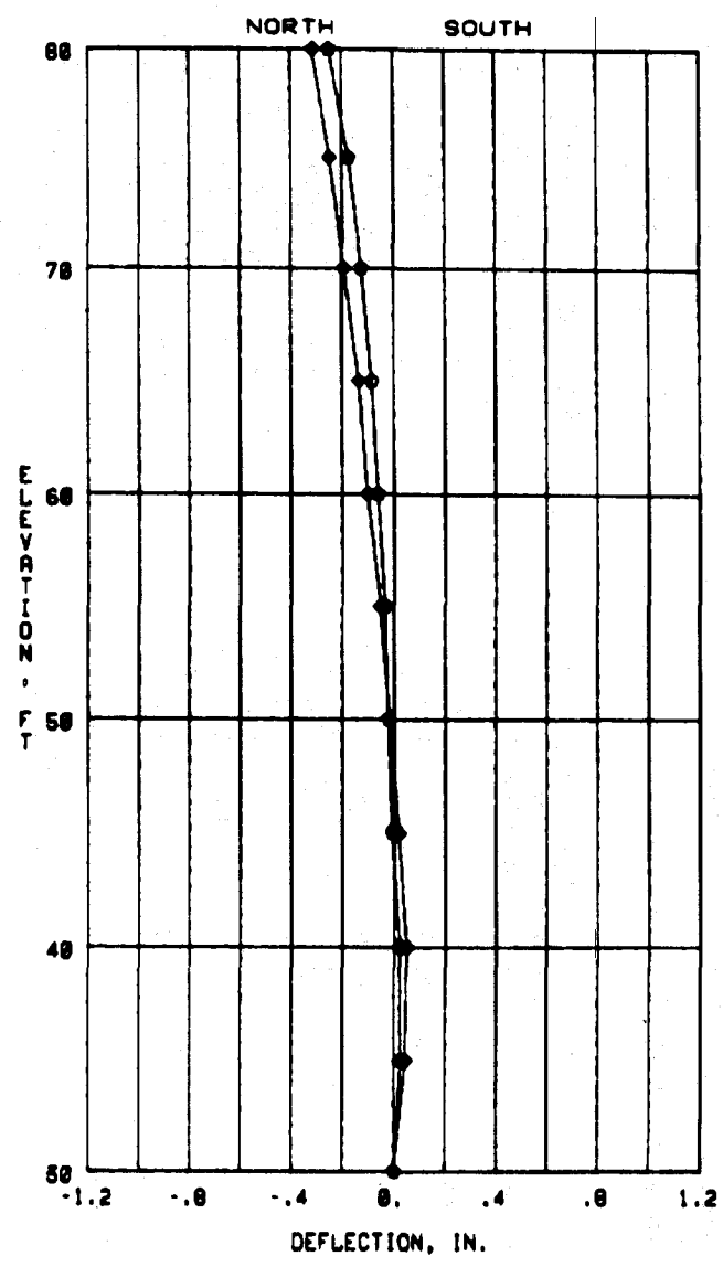
Figure 4-13. Typical Graph of Deflection Versus Elevation
