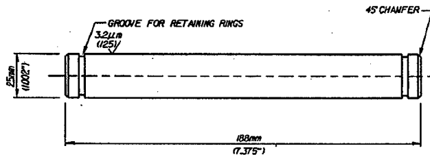
ROLLER PIN
