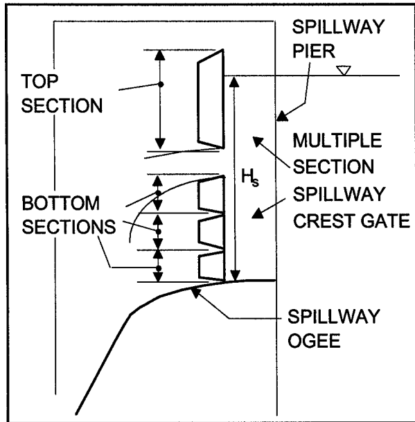
Figure 4-3. Multiple-section spillway crest gate
