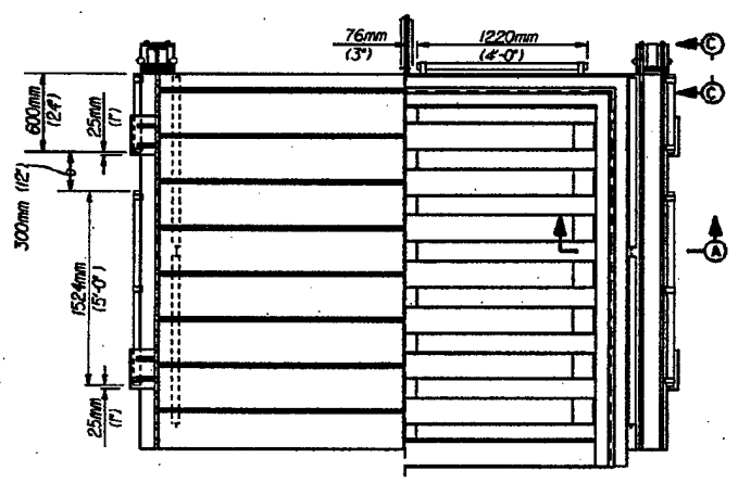
ELEVATION EMERGENCY GATE
