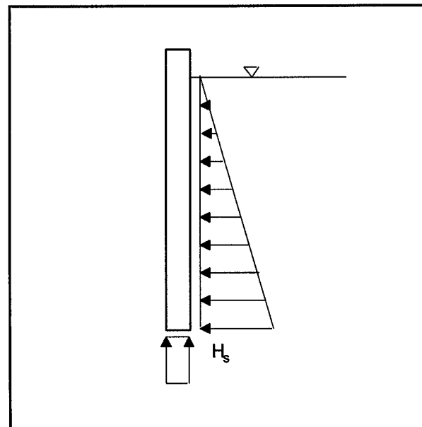
Figure 4-2. Single-section spillway crest gate, hydrostatic loading diagram
