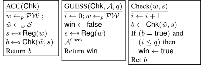
Fig. 4: (Left) Experiment for defining acceptance utility for a checking scheme \text{Reg}, \text{Chk} . (Right) Security game for online guessing attacks against a checking scheme \text{Reg}, \text{Chk} in which \mathcal{A} may make q calls to its oracle \text{Check} . Both experiments are implicitly parameterized by a password and typo setting (p, \tau) .
