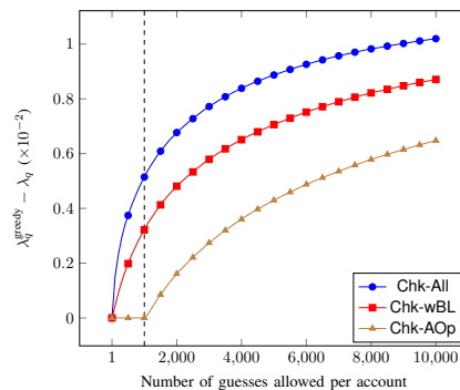
Fig. 6: The security loss as a function of q for challenge distribution RockYou and \mathcal{C}_{\text{top}2} .
