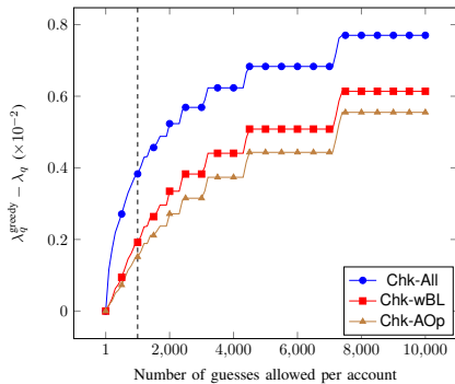
Fig. 7: Difference in exact-knowledge adversary success against typo-tolerant schemes and exact checking, as a function of q for challenge distribution phpBB and \mathcal{C}_{\text{top}2} .
