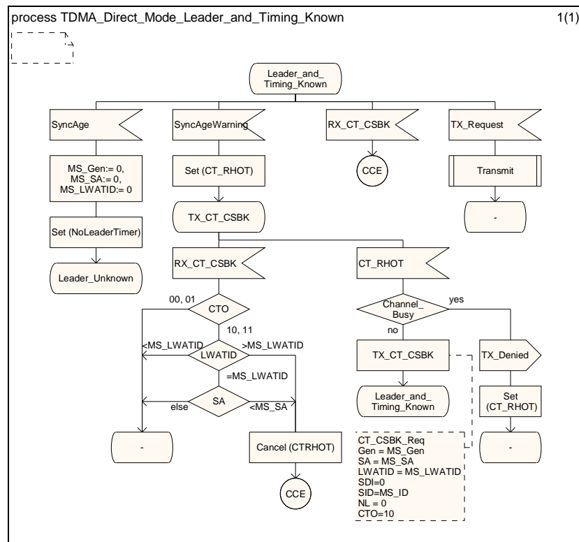
Figure 6.5: Leader and timing known SDL
