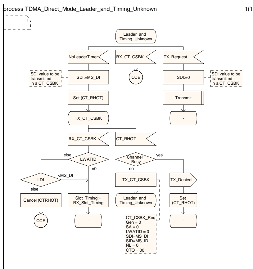
Figure 6.3: Leader and timing unknown SDL
