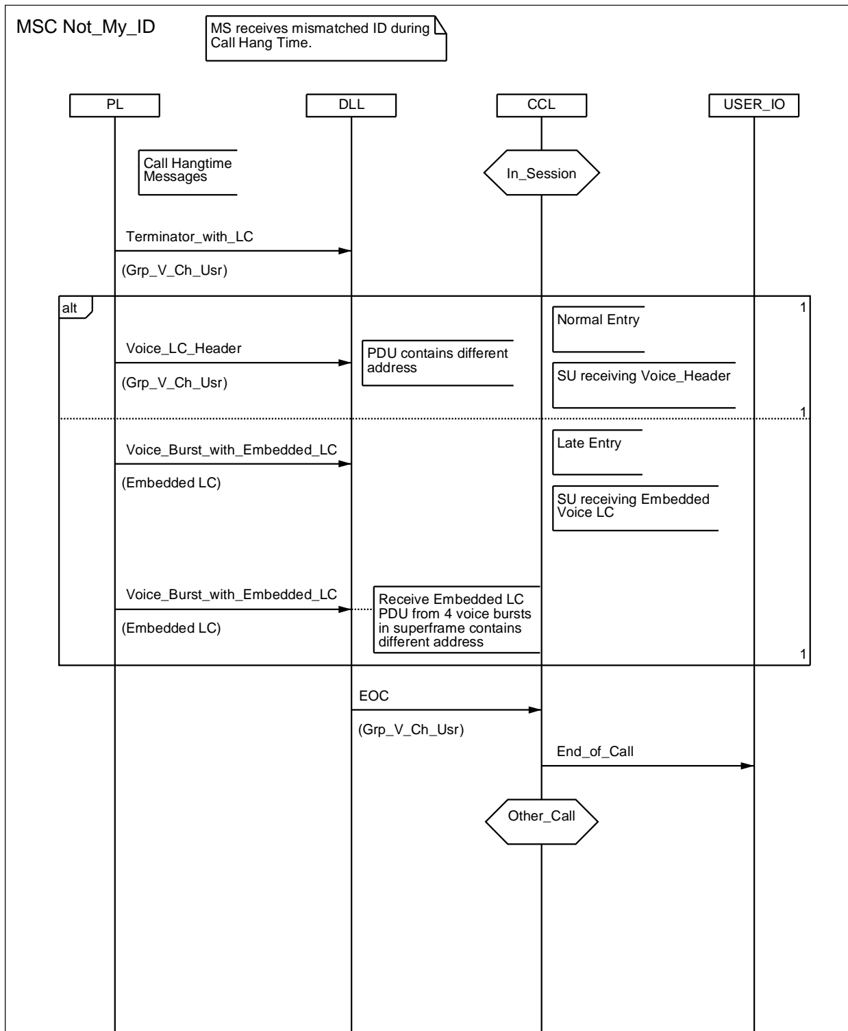
Figure 5.20: MSC Not_My_ID
