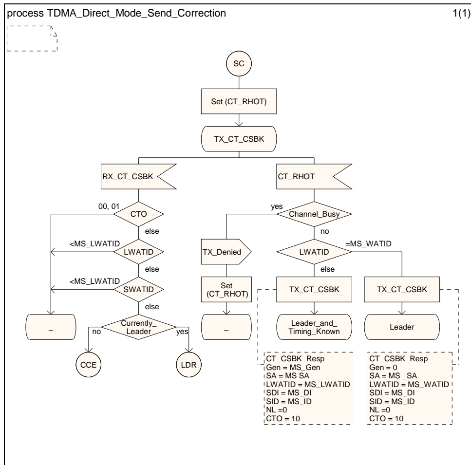
Figure 6.9: Send correction SDL
