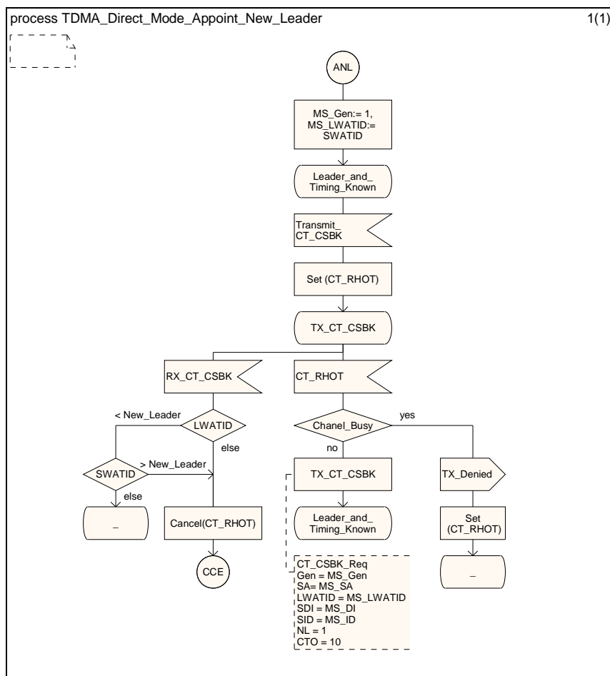
Figure 6.11: Appoint new leader SDL
