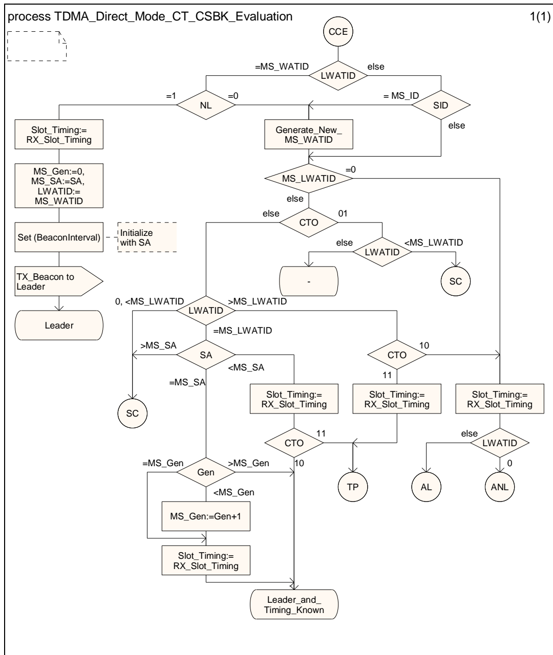
Figure 6.8: CT_CSBK evaluation SDL
