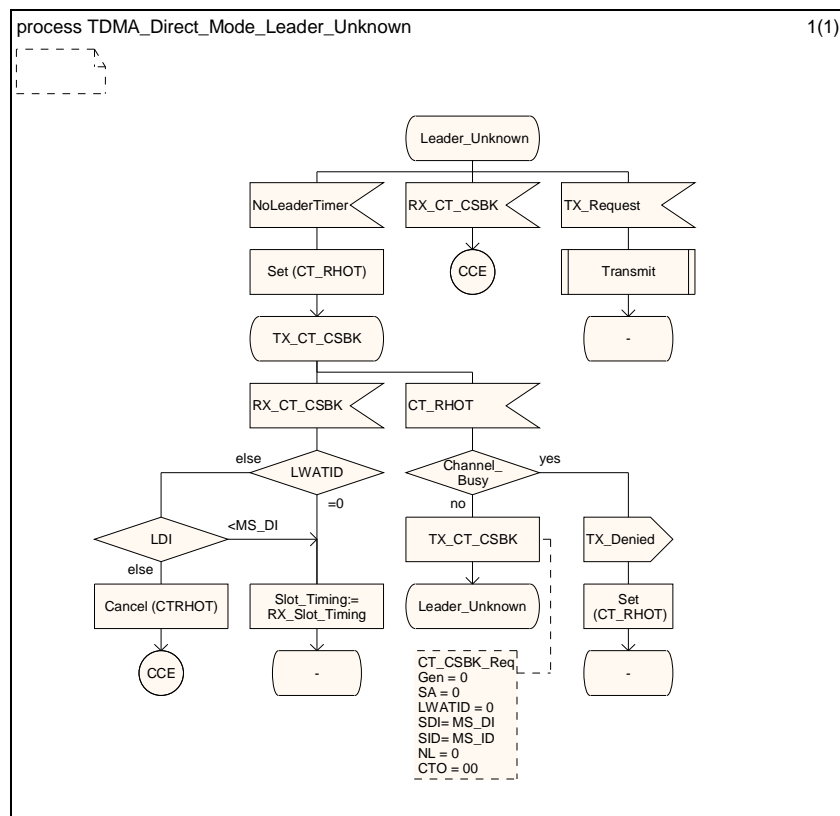
Figure 6.4: Leader unknown SDL
