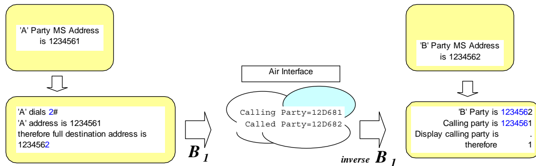
Figure C.6: Example of abbreviated dialling
