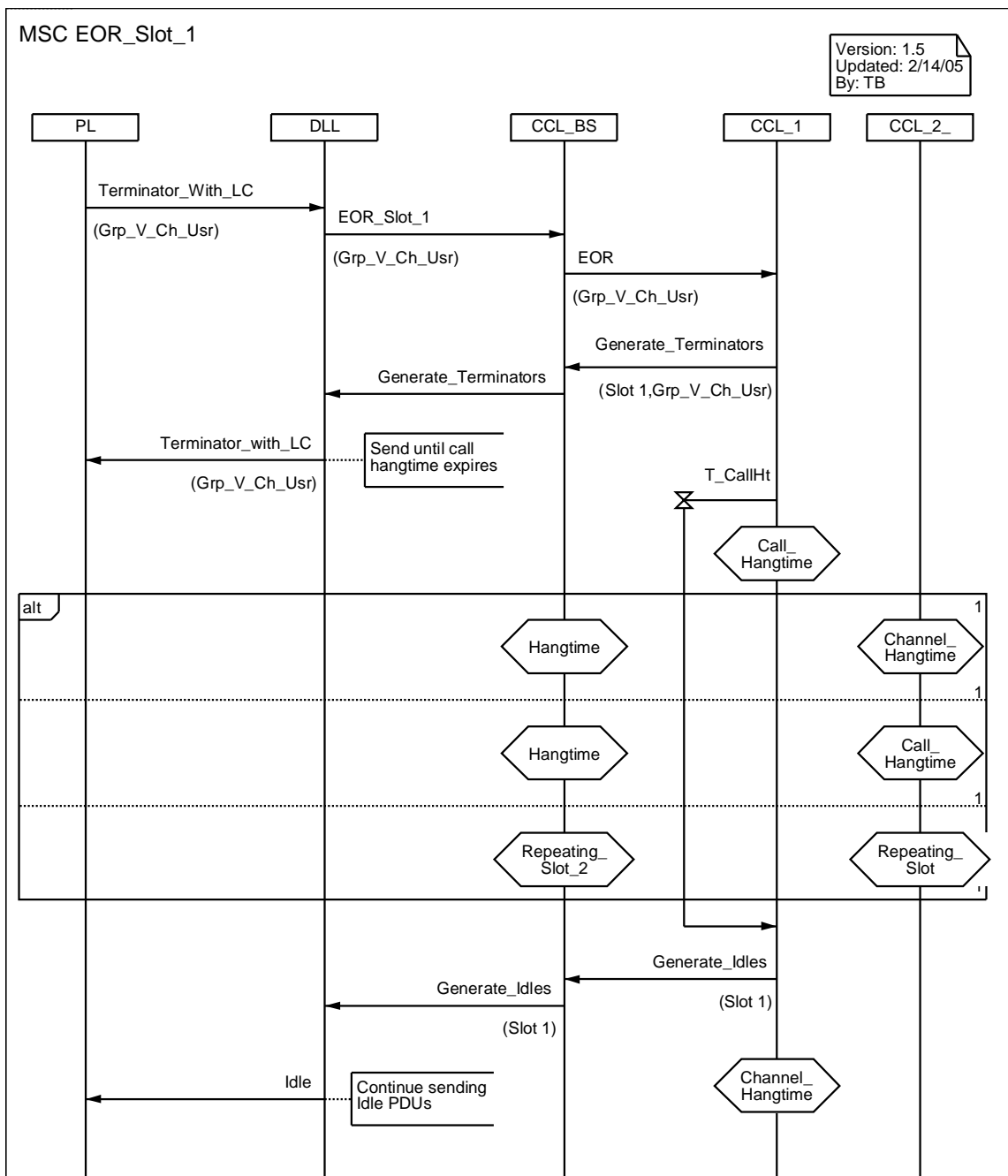
Figure 5.6: BS EOR_Slot_1
