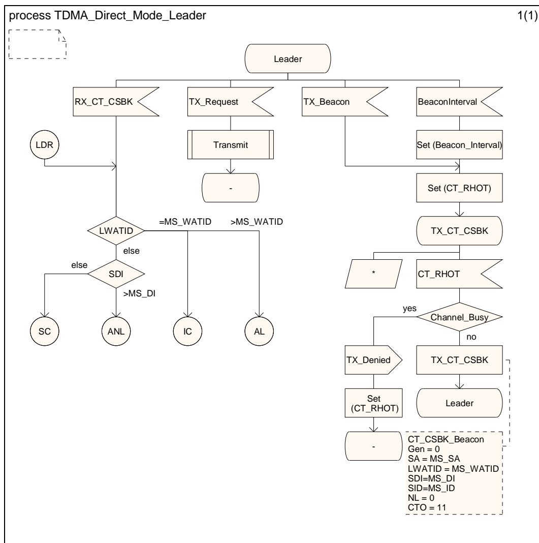
Figure 6.6: Leader SDL
