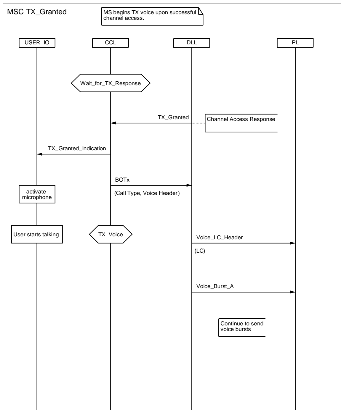
Figure 5.14: MSC TX_Granted
