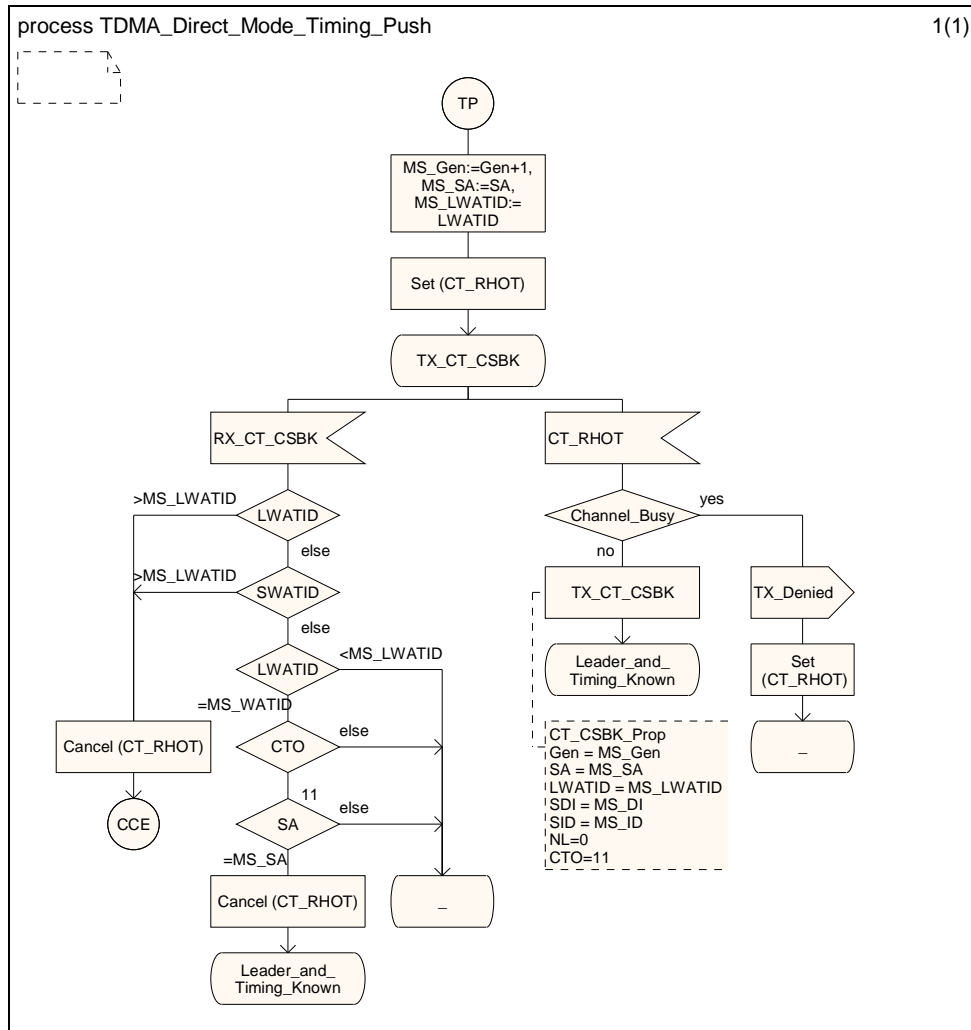
Figure 6.12: Timing push SDL
