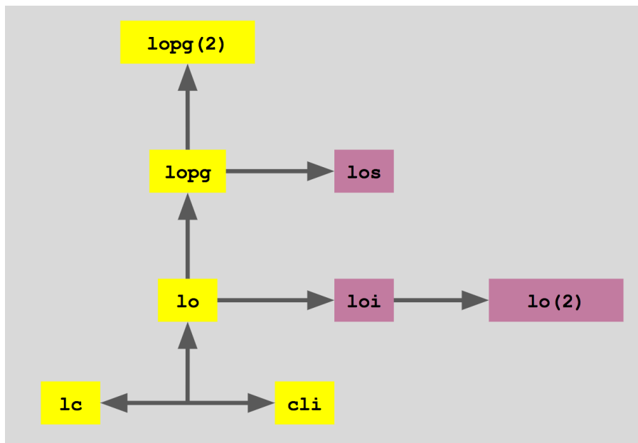
The development tree of LOKI2 in the Moonlight Maze samples from 1997–1999.
