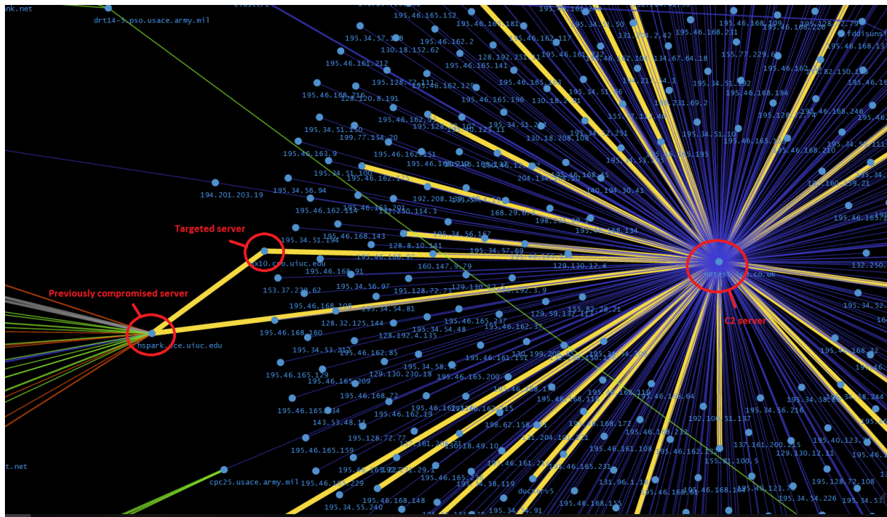
Search results for eee.tar.z highlighted in yellow. The connection between two non-relay nodes was unexpected.
