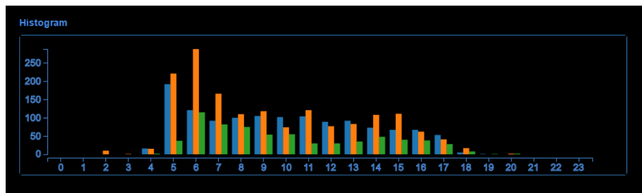
Time-of-day histogram (GMT) for file transfers with HRTest. Blue denotes operator connections, orange is retrieval by targeted hosts, and green is file exfiltration. April 2016.
