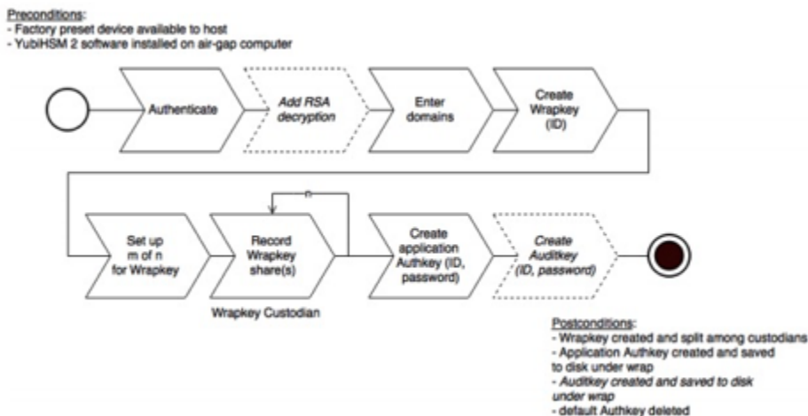
Figure: Pre- and Post-Conditions
