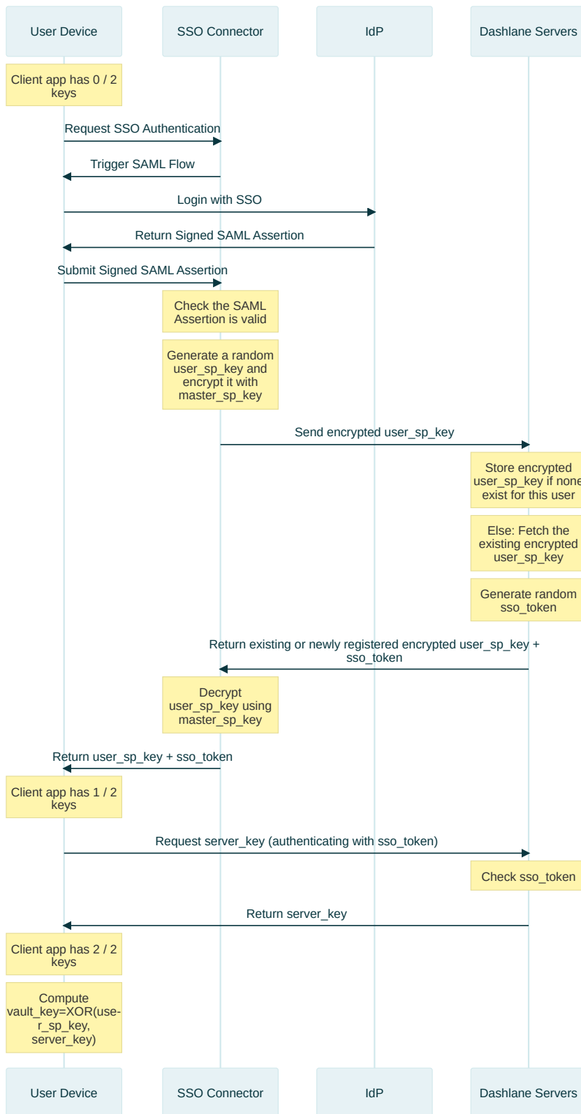
Figure 5: SSO Workflow
