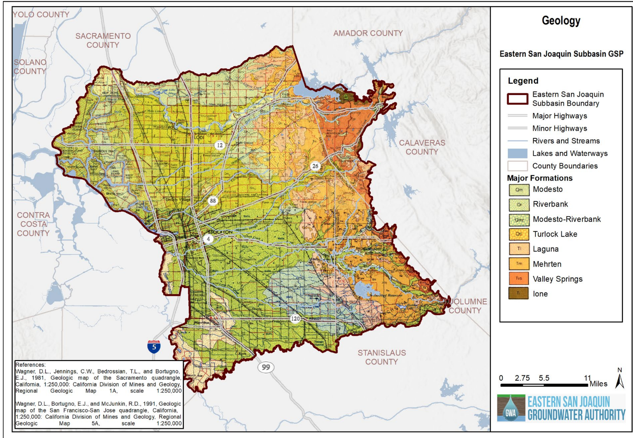
Figure 2-16: Geologic Map
