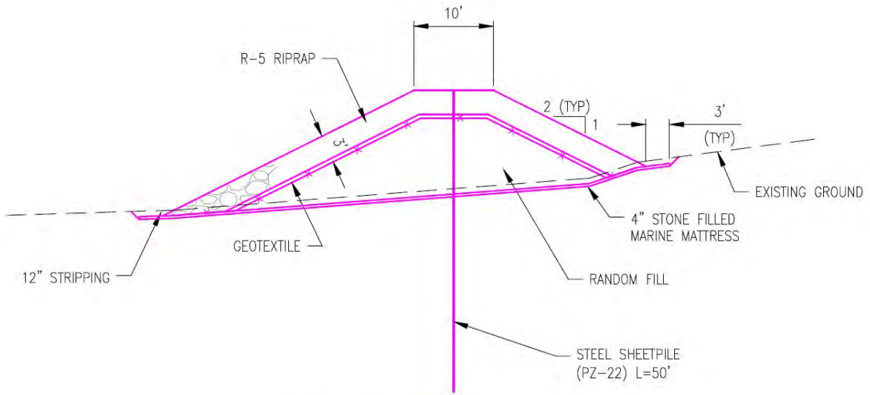
TYPICAL SECTION – LEVEE – TYPE A NTS
