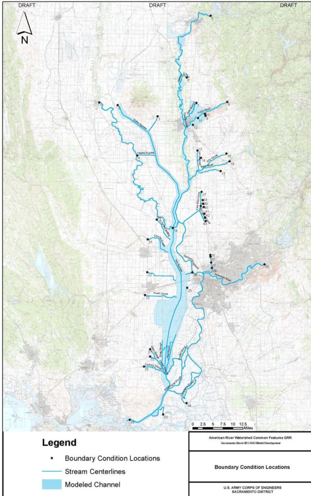
Figure 1. USACE Sacramento River 1-D HEC-RAS Model Extents (Source: USACE)
