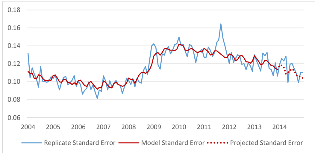
Figure 6: Replicate, model, and projected standard errors (in thousands) for unemployment rate . Not seasonally adjusted.
