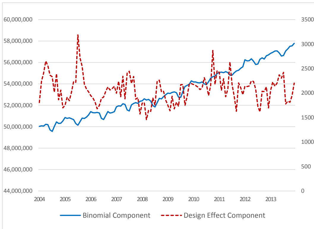
Figure 3: Decomposition of civilian labor force replicate variance into "binomial" [Np(1-p)] and "design effect" [N\delta/n] components. The design effect component is on the secondary (right-hand) scale.
