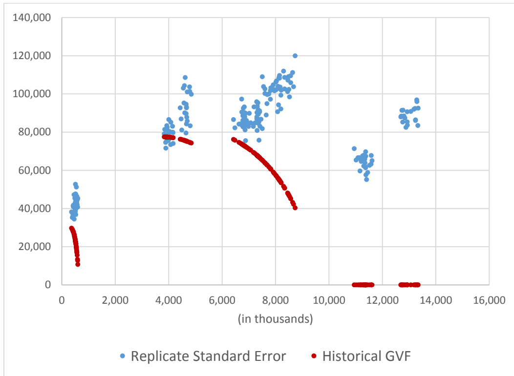
Figure 1: Replicate and GVF standard errors (vertical axis) plotted against associated survey estimates of employed, unemployed, and not in labor force for Asian, 20 and older and Asian, 16 and older .
