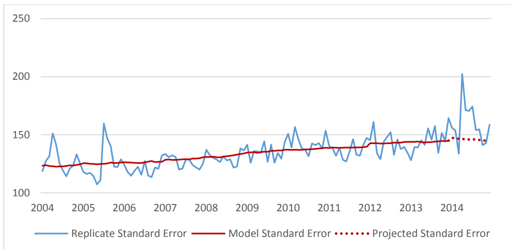
Figure 5: Replicate, model, and projected standard errors (in thousands) for Hispanic or Latino employment . Not seasonally adjusted.
