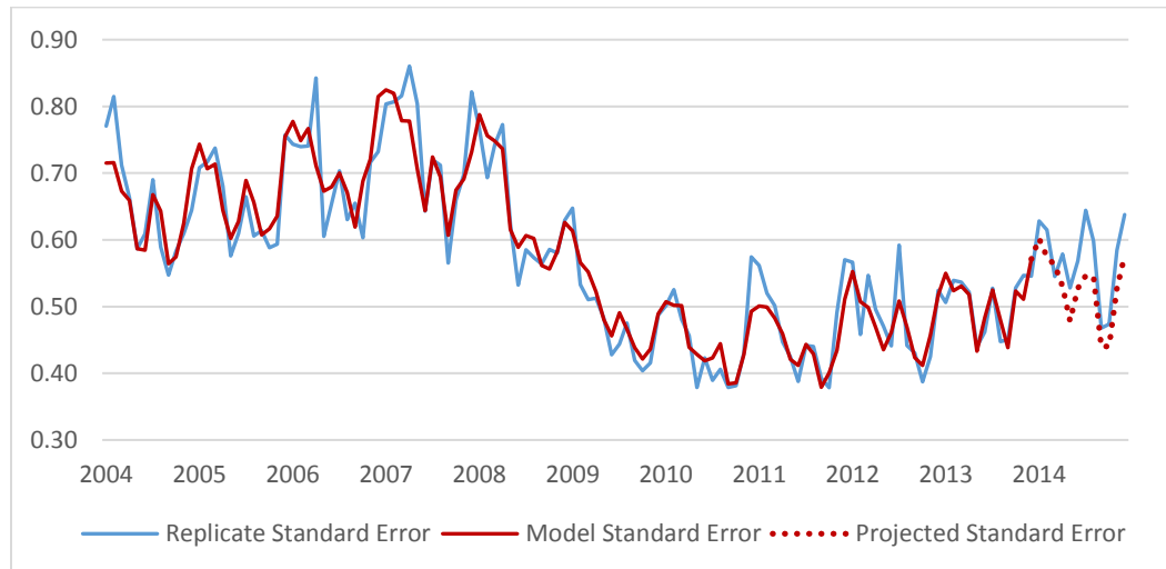
Figure 8: Replicate, model, and projected standard errors (in percent) for job losers on layoff, as a percent of total unemployed .
