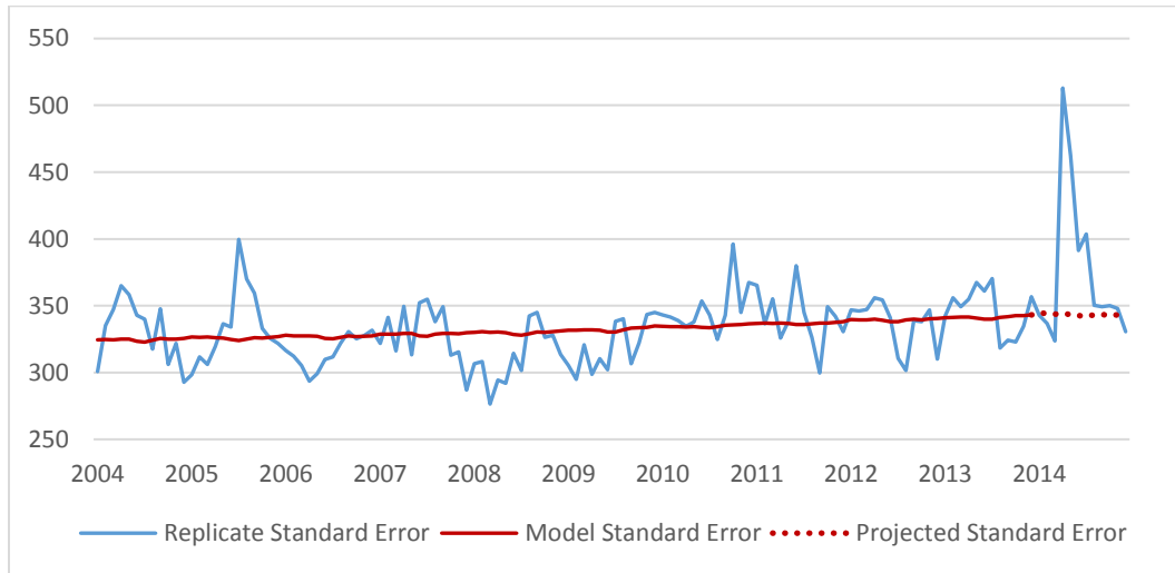
Figure 4: Replicate, model, and projected standard errors (in thousands) for civilian labor force . Not seasonally adjusted.
