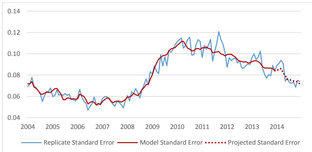
Figure 7: Replicate, model, and projected standard errors (in percent) for unemployed 15 weeks and over, as a percent of civilian labor force . Not seasonally adjusted.
