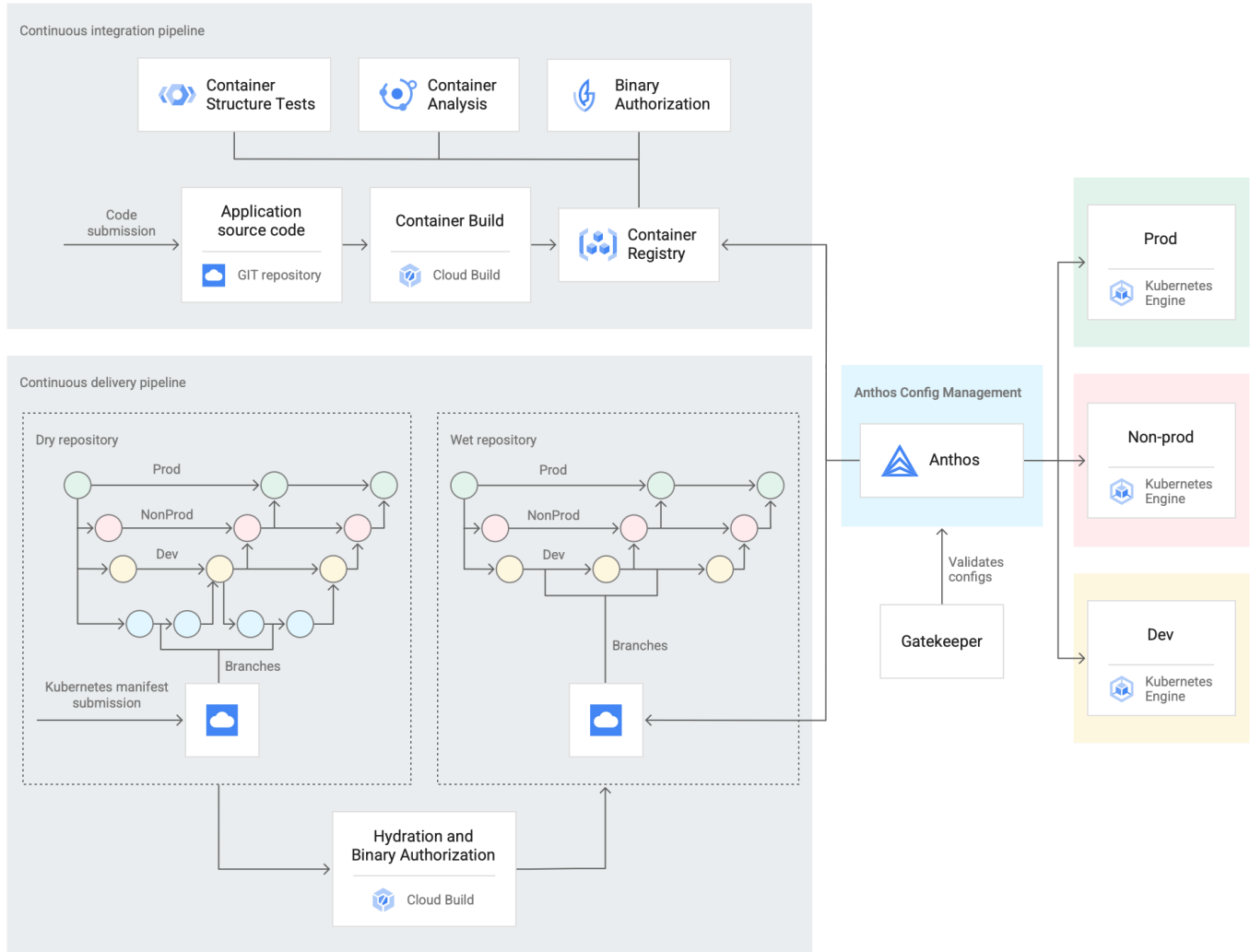
Figure 2.5.5 Application deployment pipeline
