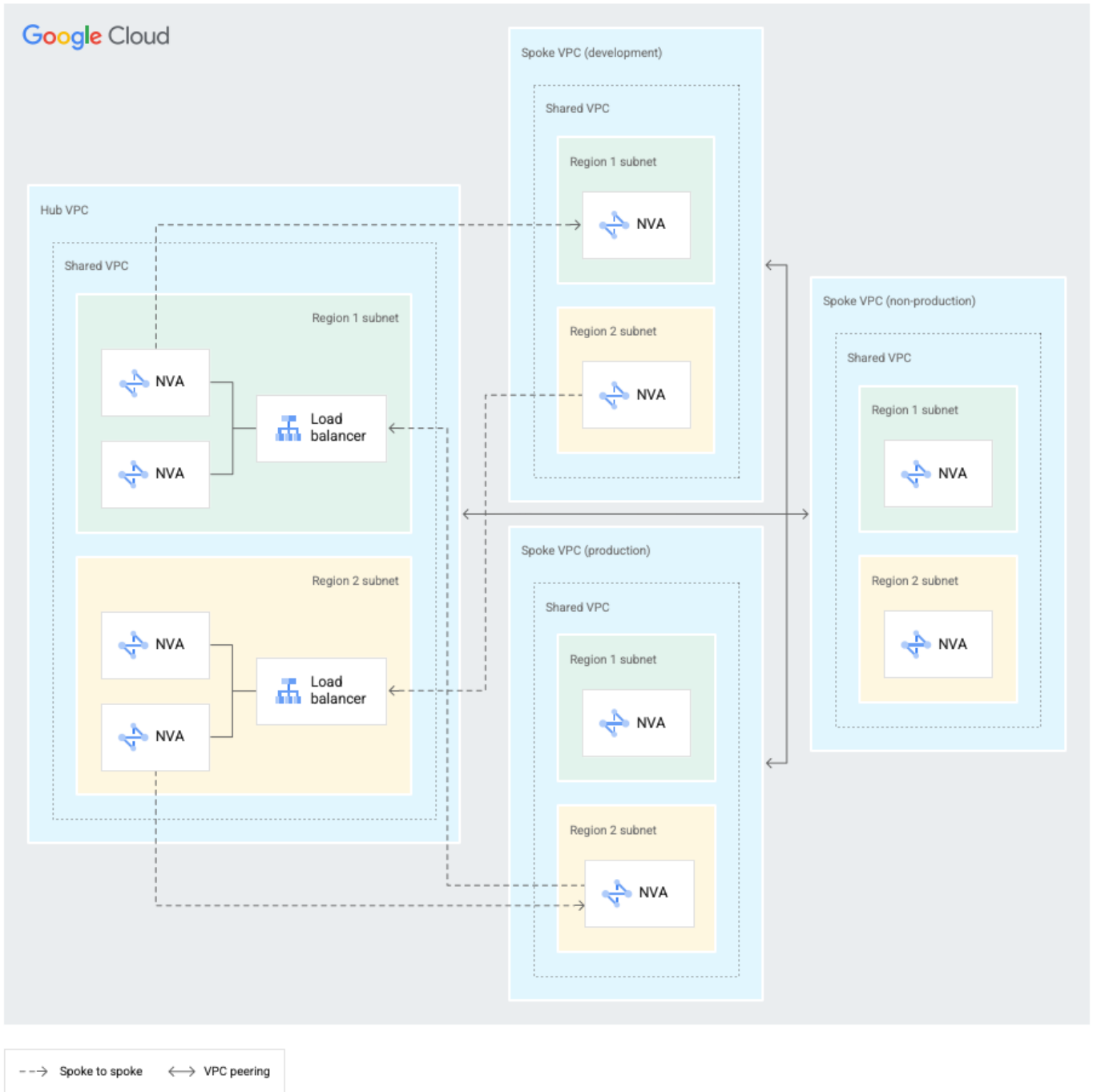
Figure 2.7.3 Spoke-to-spoke connectivity using network virtual appliances (NVAs)
