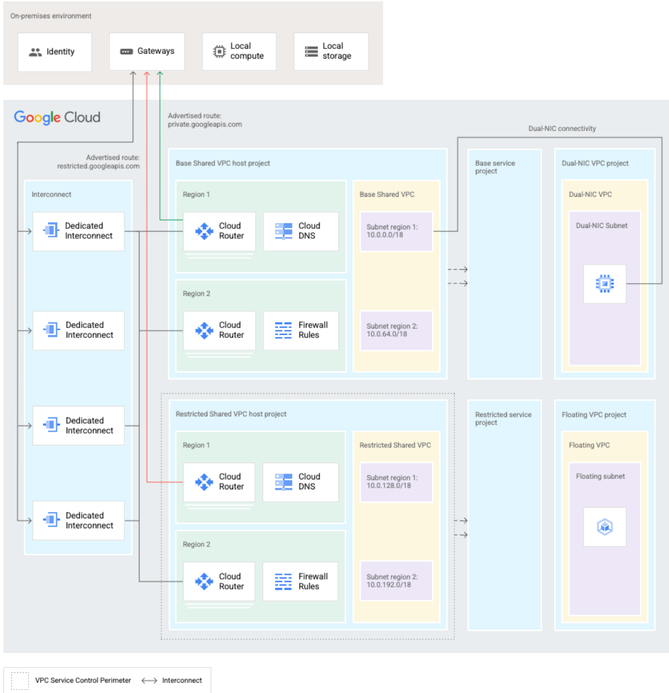
Figure 2.7.1 The example.com VPC network structure
