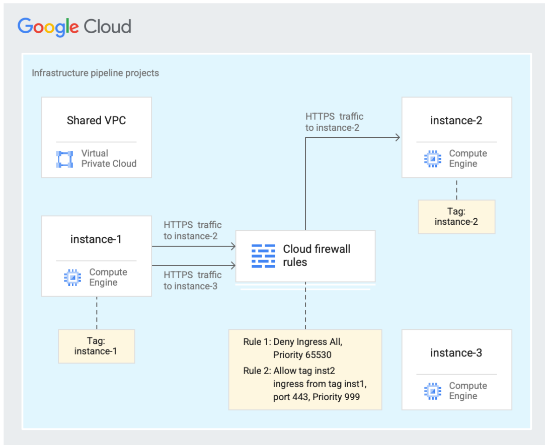
Figure 2.7.6 Firewall rules in example.com
