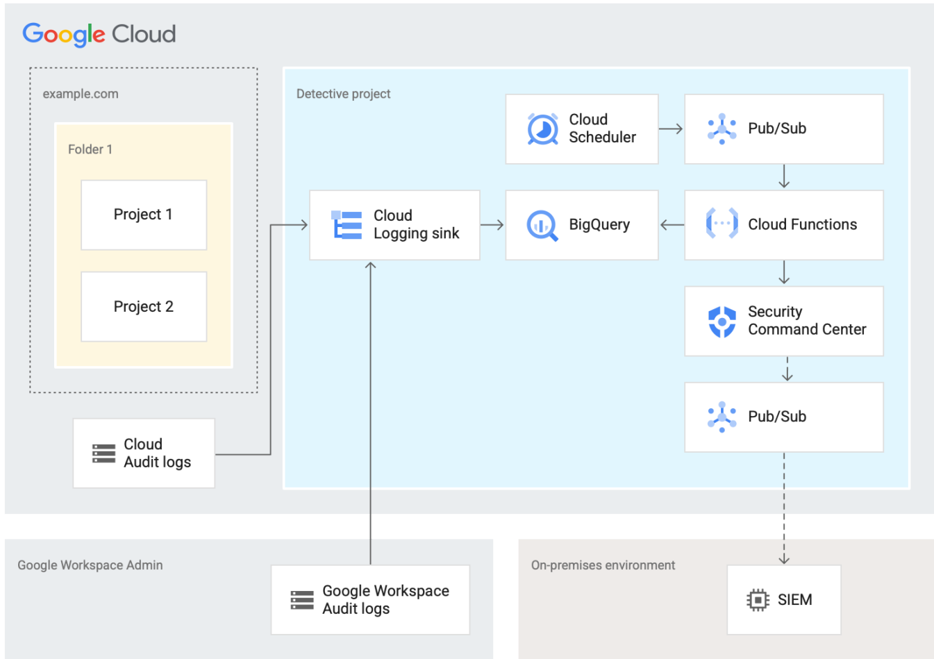
Figure 2.10.8 BigQuery-based analysis architecture
