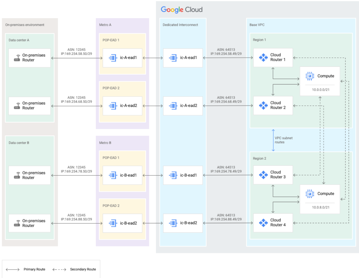
Figure 2.7.4 The example.com Dedicated Interconnect connection structure
