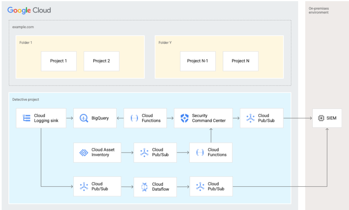
Figure 2.10.1 Detective control architecture in example.com
