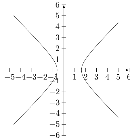
FIGURE 23.2: Le graphique de x^2 - x - y^2 - 1 = 0 . LabelFigProjPoly
