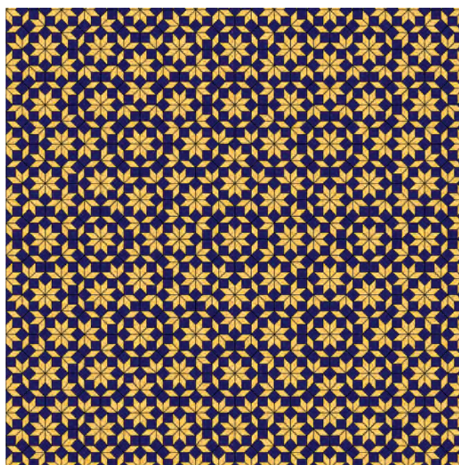
Figure 19. Ammann-Beenker (or “octagonal”) tiling.
