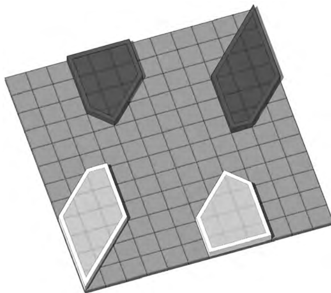
Figure 5. A general construction for the Peaceable Queens problem found by Benoît Jubin, showing that for large n , a(n) \geq \lceil 7n^2/48 \rceil , a formula which might be exact for all n > 9 .
