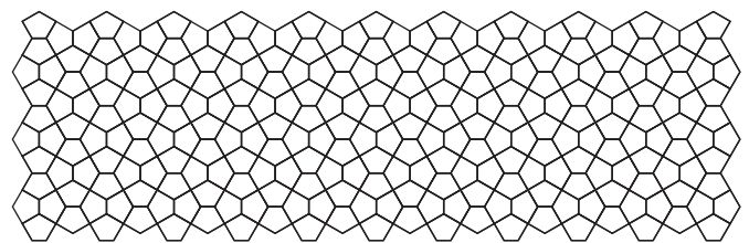
Figure 17. A portion of the Cairo tiling.
