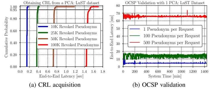
Fig. 8. End-to-end latency for revocation update (LuST dataset).
