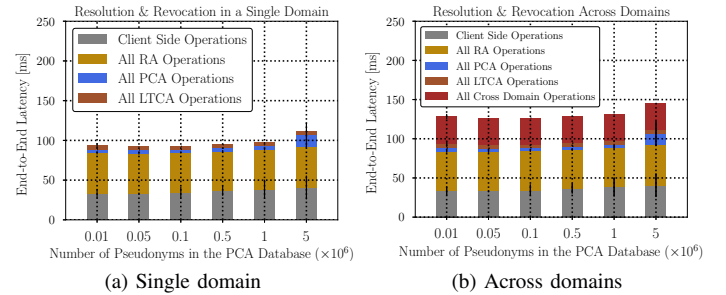
Fig. 9. End-to-end latency to resolve and revoke a pseudonym.
