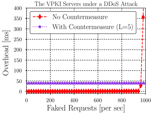
Fig. 7. The VPKI servers are under a DDoS attack: overhead to obtain pseudonyms for LuST dataset with P1 (difficulty level: L=5 , \tau_P = 5 min).
