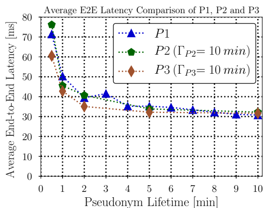
Fig. 5. End-to-end latency comparison for different policies (Tapas dataset).
