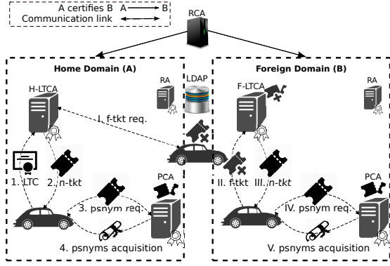
Fig. 1. Pseudonym acquisition overview in the home and foreign domains.
