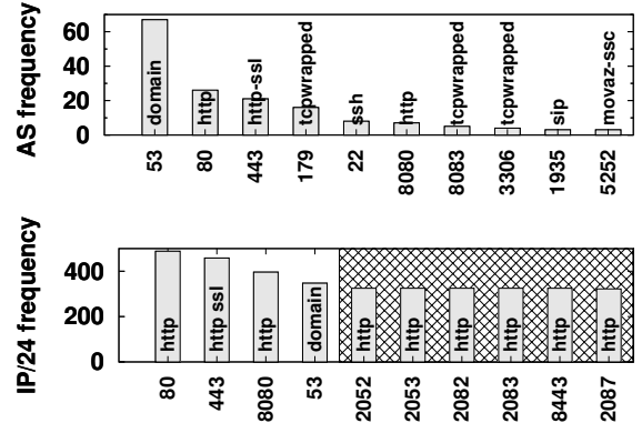
Figure 14: Overall nmap portscan statistics and Top-10 open TCP ports (per AS and per /24).
