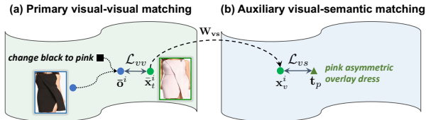
Figure 3. Feature matching in a two-level hierarchical space.
