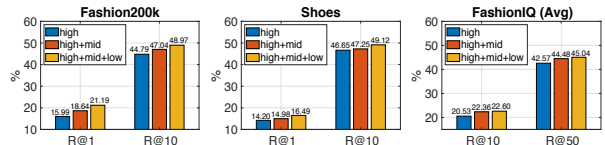
Figure 8. Effect of composition at multi-level.
