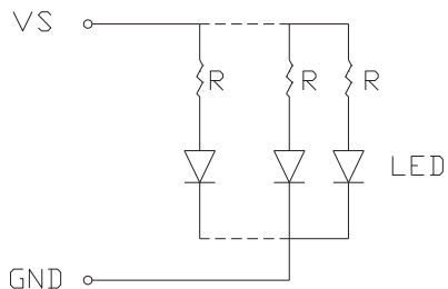
Recommended Set-up
