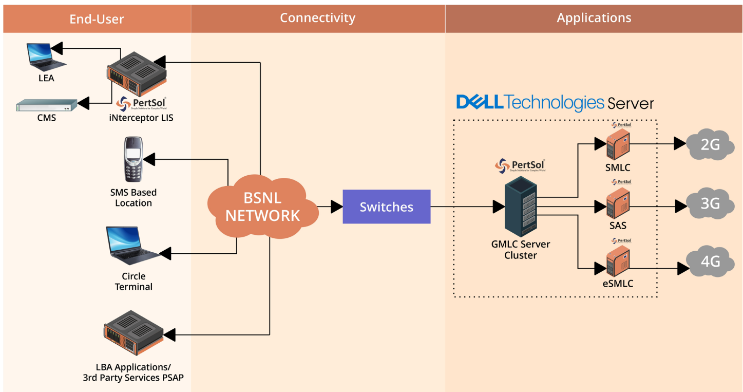
Location-Based System Architecture
