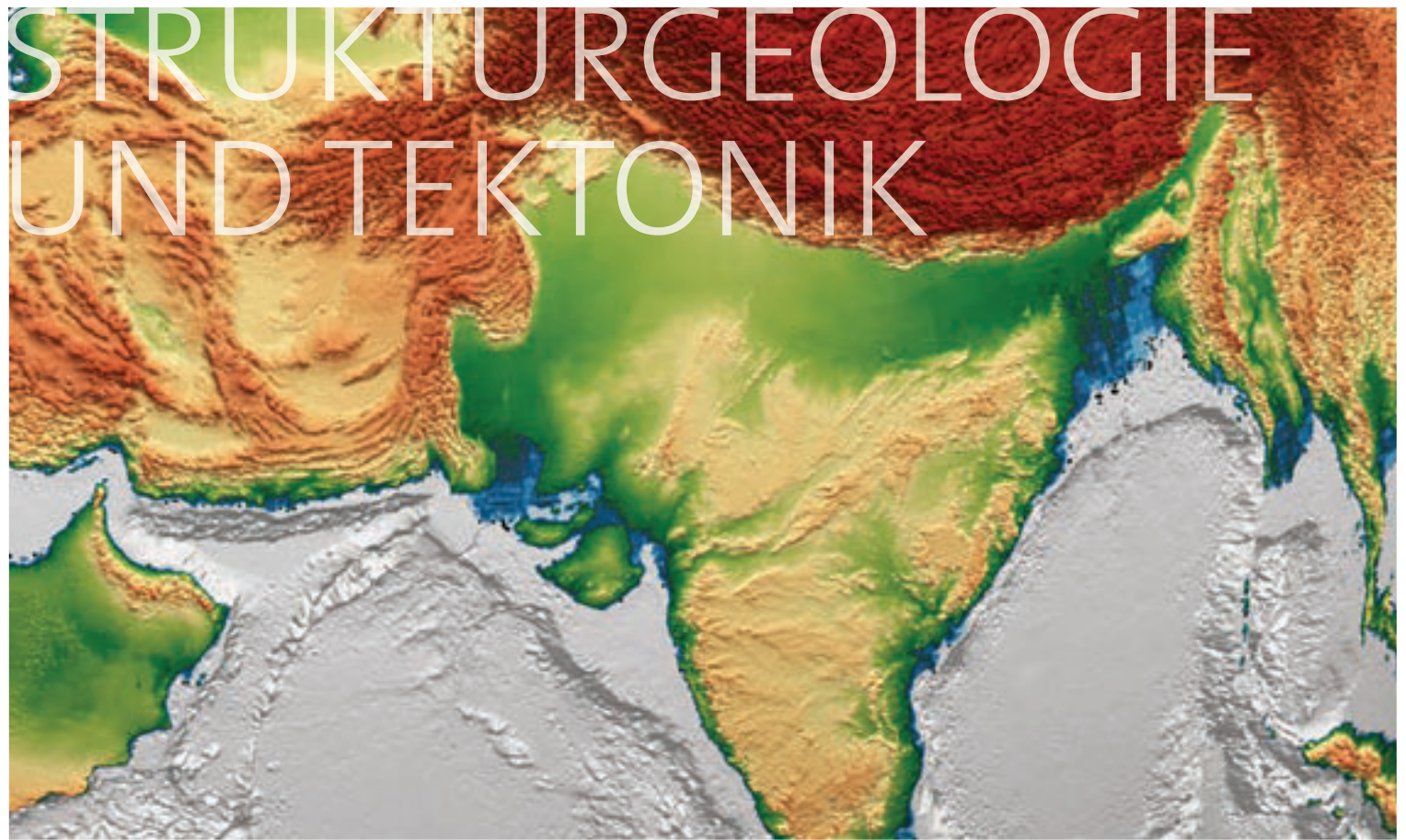
Alpine Himalayan mountain belt colored by topographic relief
