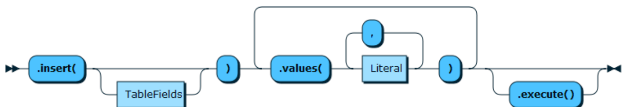
Figure 11.16 TableInsertFunction
