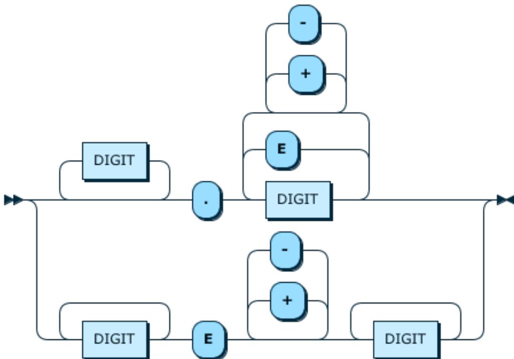
Figure 12.33 FLOAT
