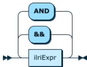
Figure 12.29 andExpr
