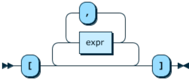
Figure 12.18 jsonarray
