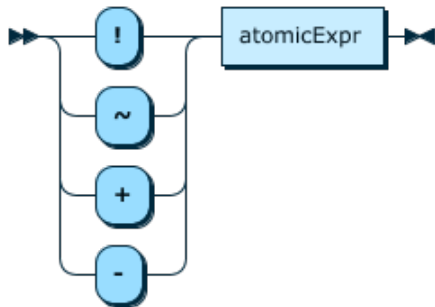
Figure 12.14 unaryOp
