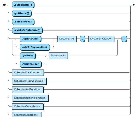
Figure 11.7 Collection
