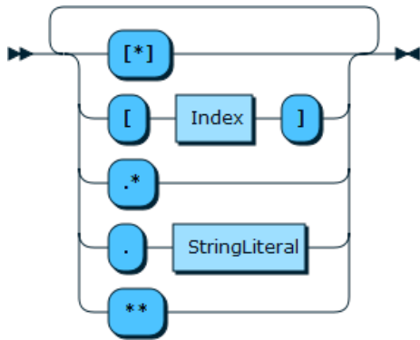
Figure 11.36 DocPath
