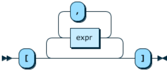
Figure 12.18 jsonarray
