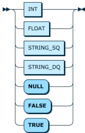
Figure 11.37 Literal
