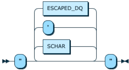
Figure 12.39 STRING_DQ
