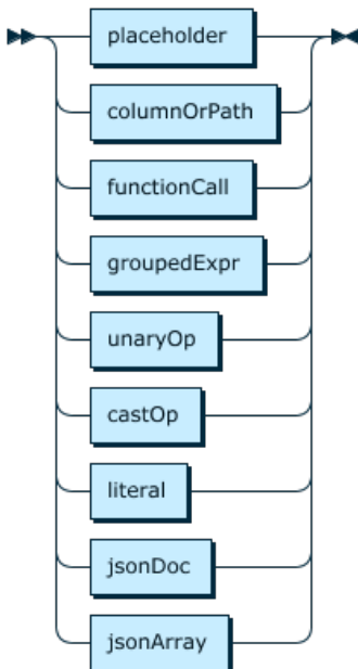
Figure 12.19 atomicExpr
