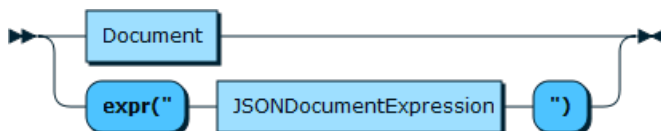
Figure 11.43 DocumentOrJSON
