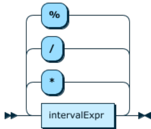
Figure 12.23 mulDivExpr
