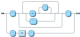
Figure 12.35 QUOTED_ID
