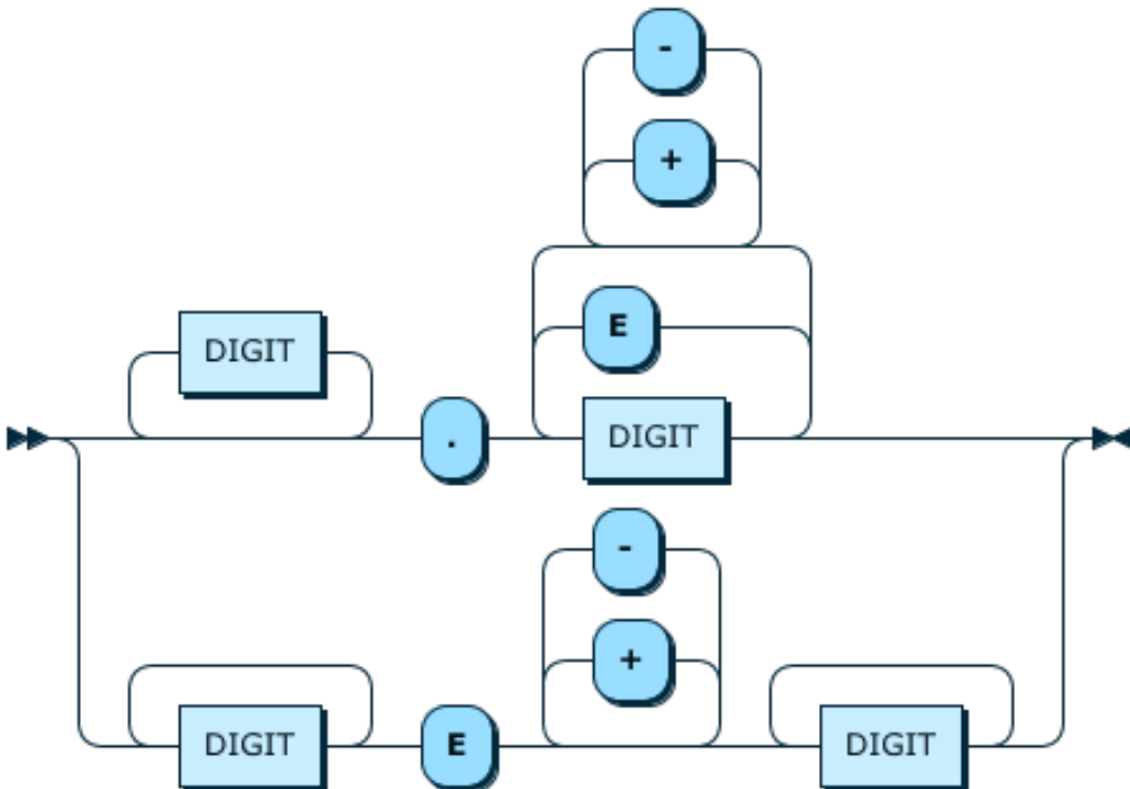
Figure 12.33 FLOAT
