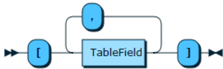
Figure 11.45 TableFields
