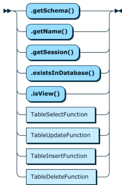
Figure 11.8 Table
