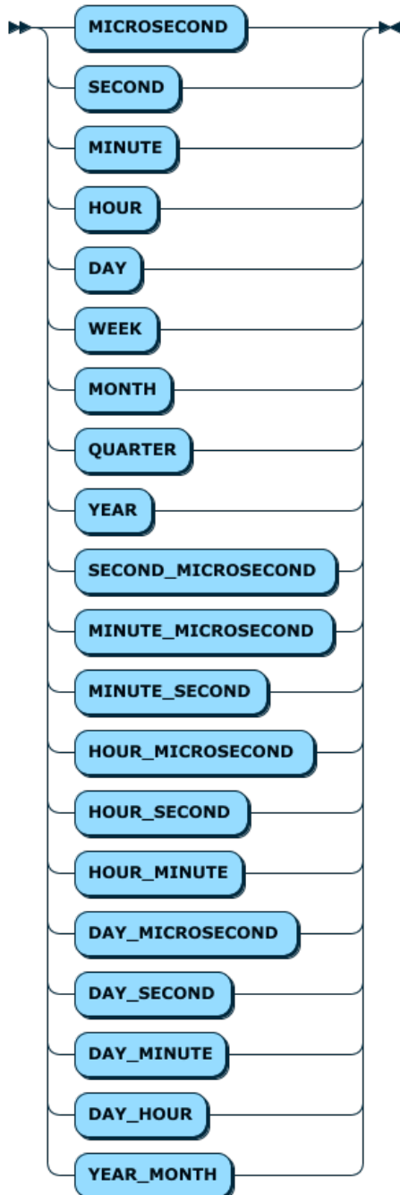
Figure 12.20 INTERVAL_UNIT
