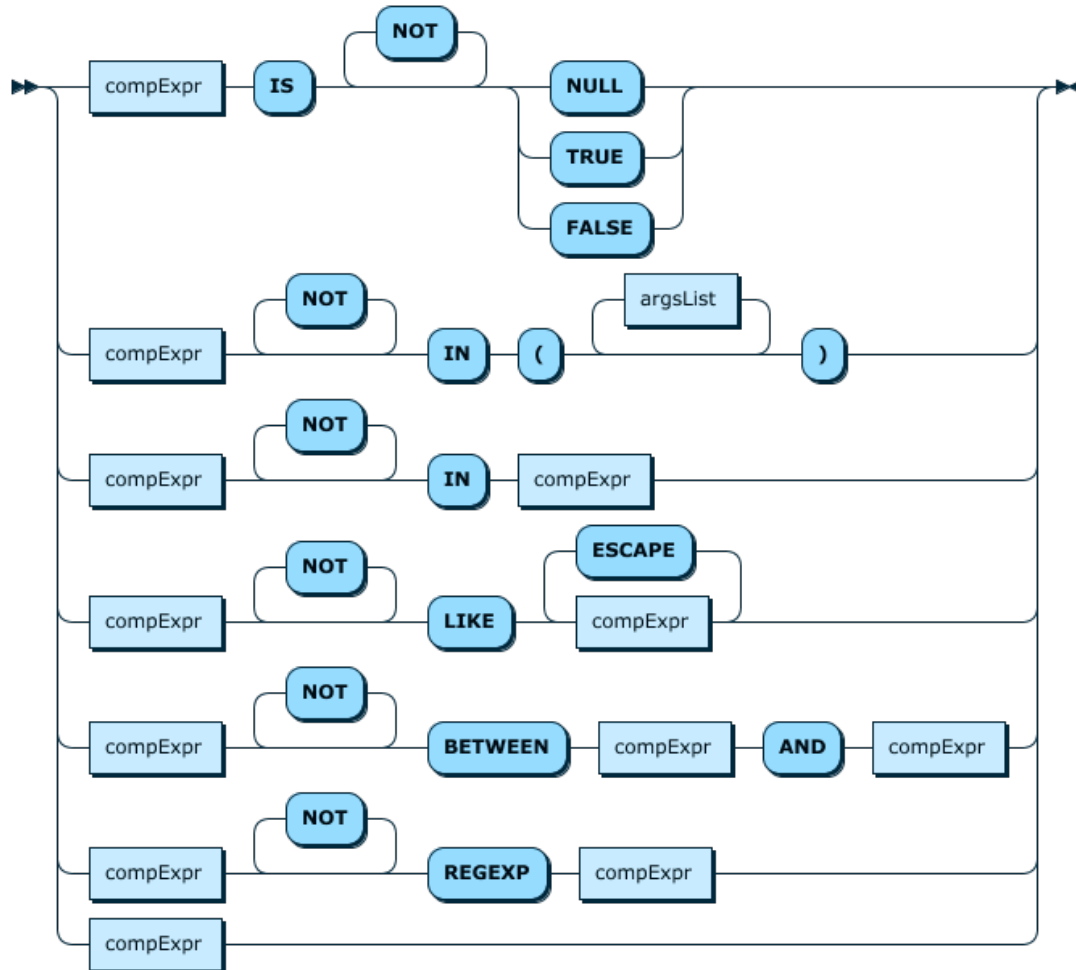
Figure 12.28 ilriExpr
