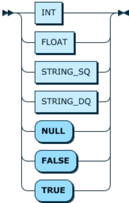
Figure 12.15 literal
