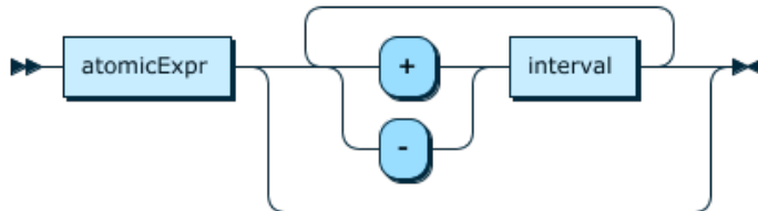
Figure 12.22 intervalExpr
