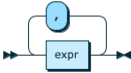
Figure 12.8 argsList
