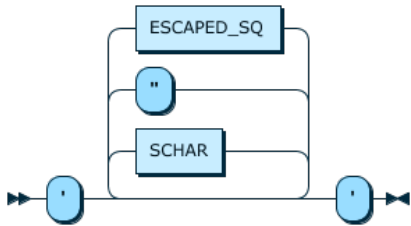
Figure 12.40 STRING_SQ
