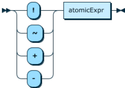
Figure 12.14 unaryOp
