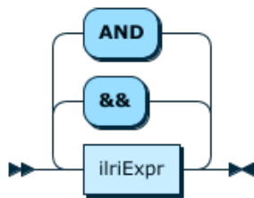
Figure 12.29 andExpr
