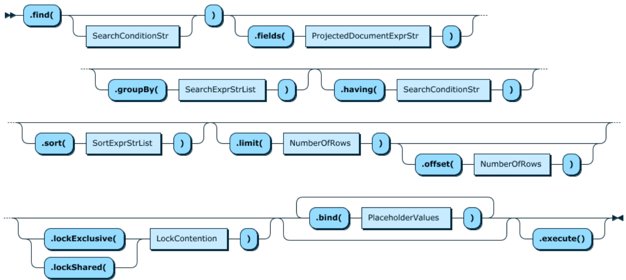
Figure 11.9 CollectionFindFunction
