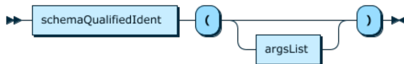
Figure 12.11 functionCall
