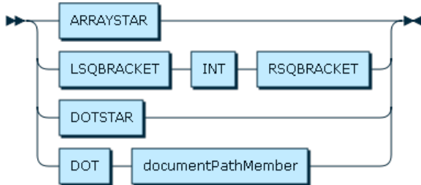
Figure 12.4 documentPathLastItem
