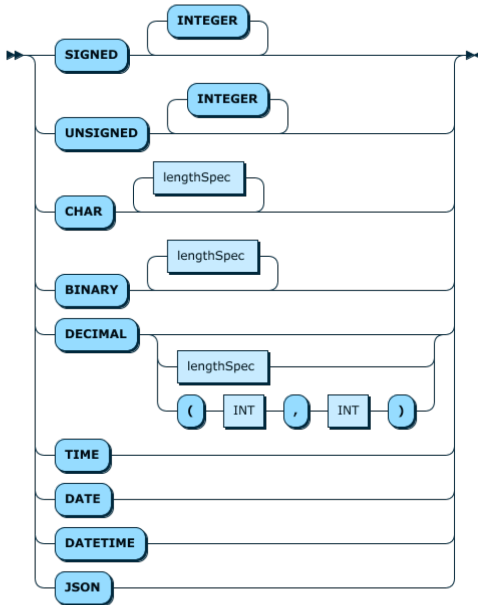
Figure 12.10 castType
