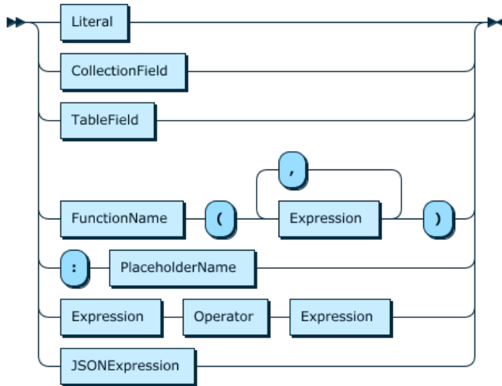
Figure 11.38 Expression
