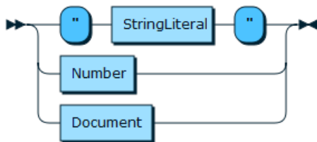
Figure 11.5 SQLLiteral
