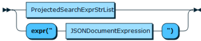
Figure 11.26 ProjectedDocumentExprStr
