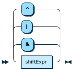
Figure 12.26 bitExpr
