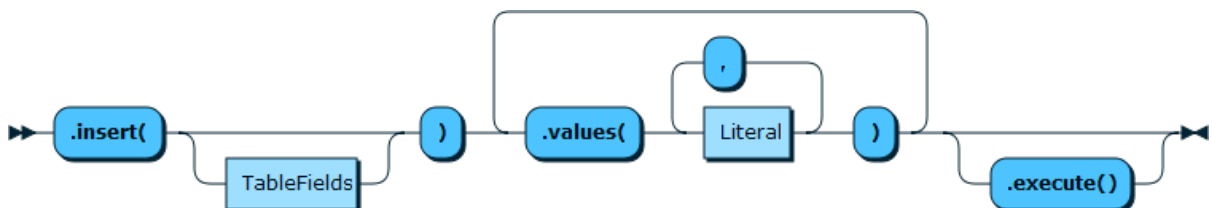
Figure 11.16 TableInsertFunction
