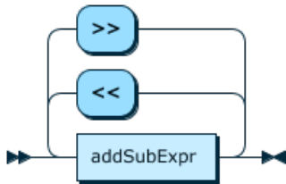
Figure 12.25 shiftExpr
