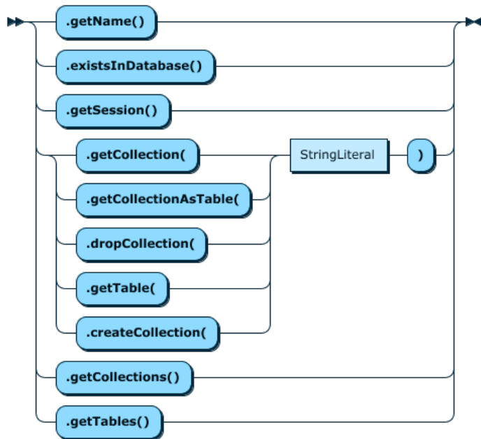
Figure 11.6 Schema
