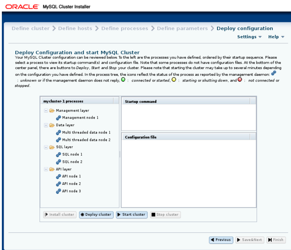
Figure 3.29 NDB Cluster Auto-Installer Deploy Configuration screen
