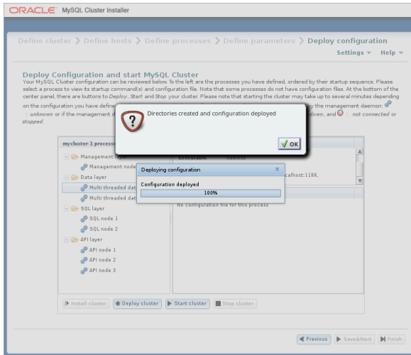
Figure 3.30 Cluster Deployment Process
