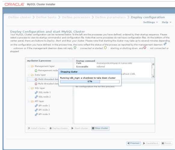
Figure 3.33 Cluster Shutdown Process, with Progress Bar
