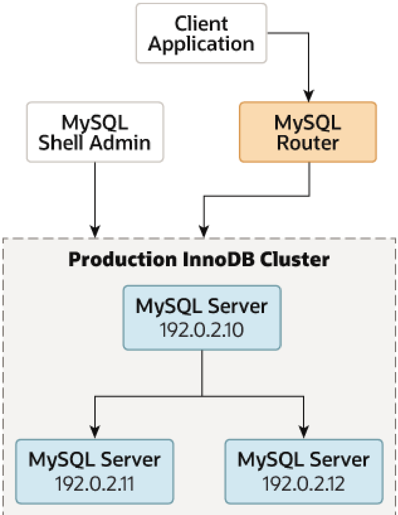
Figure 7.2 Production Deployment
