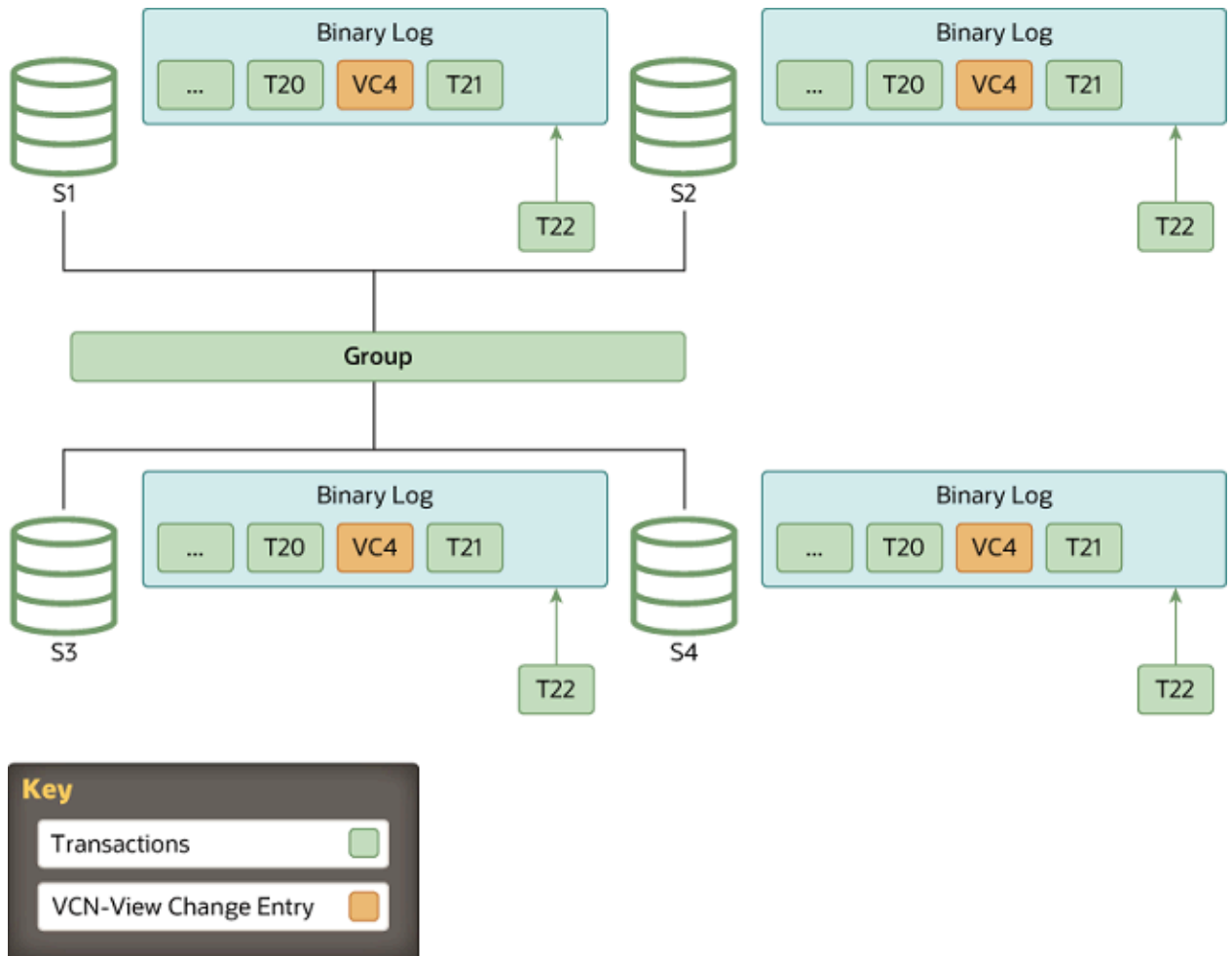
Figure 18.12 Instance Online
