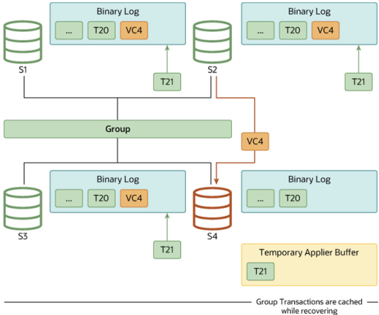
Figure 18.11 Queued Transactions
