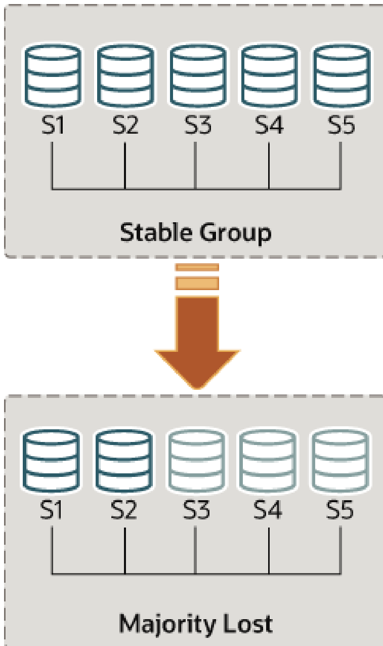
Figure 18.13 Losing Quorum
