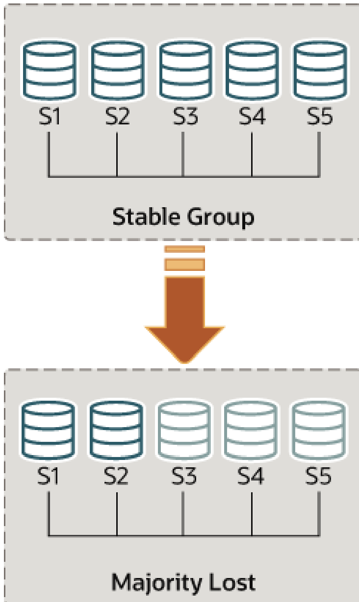
Figure 17.7 Losing Quorum
