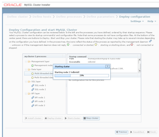
Figure 21.34 Cluster Startup Process with Progress Bar
