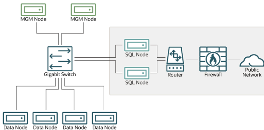
Figure 21.40 NDB Cluster with Hardware Firewall
