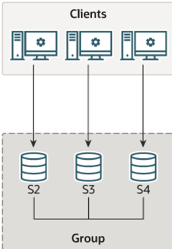
Figure 17.4 Group Architecture
