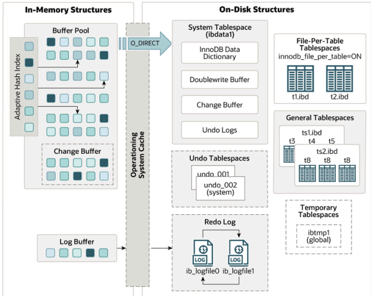
Figure 14.1 InnoDB Architecture
