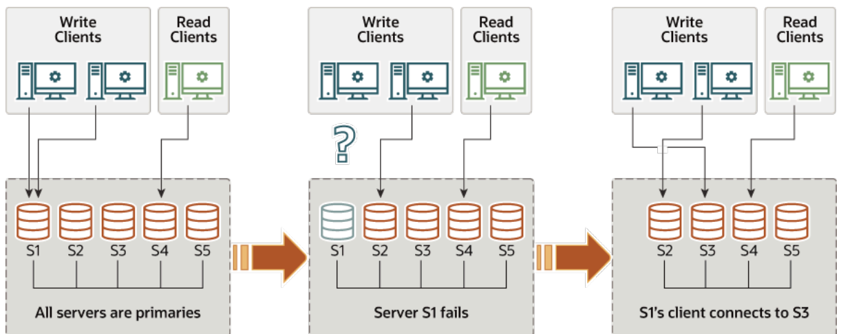
Figure 17.6 Client Failover
