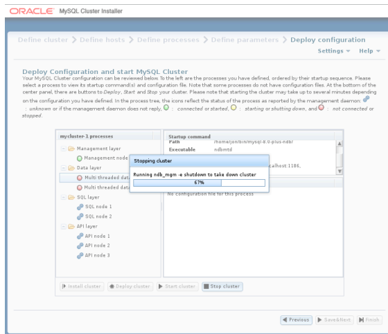
Figure 21.36 Cluster Shutdown Process, with Progress Bar
