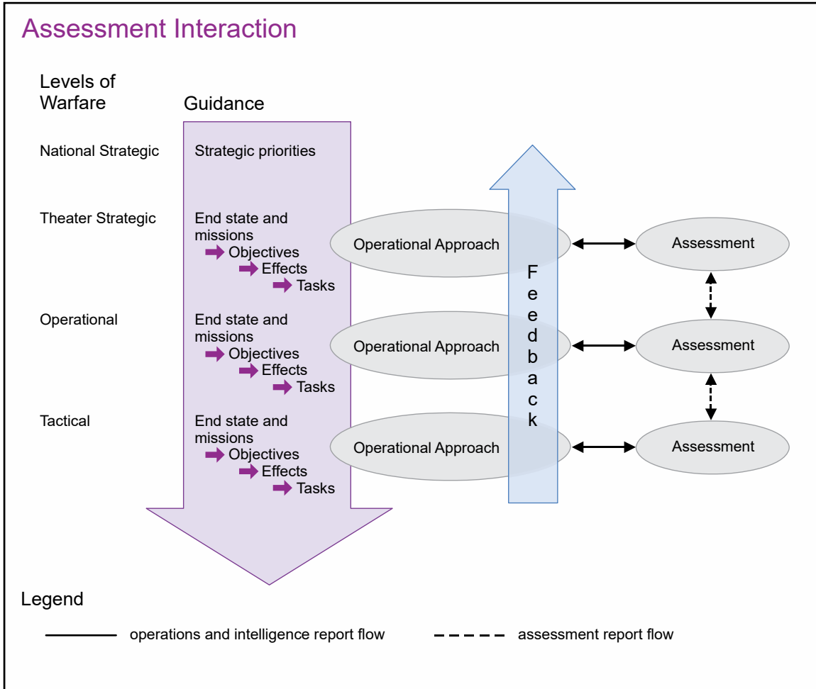
Figure II-2. Assessment Interaction
