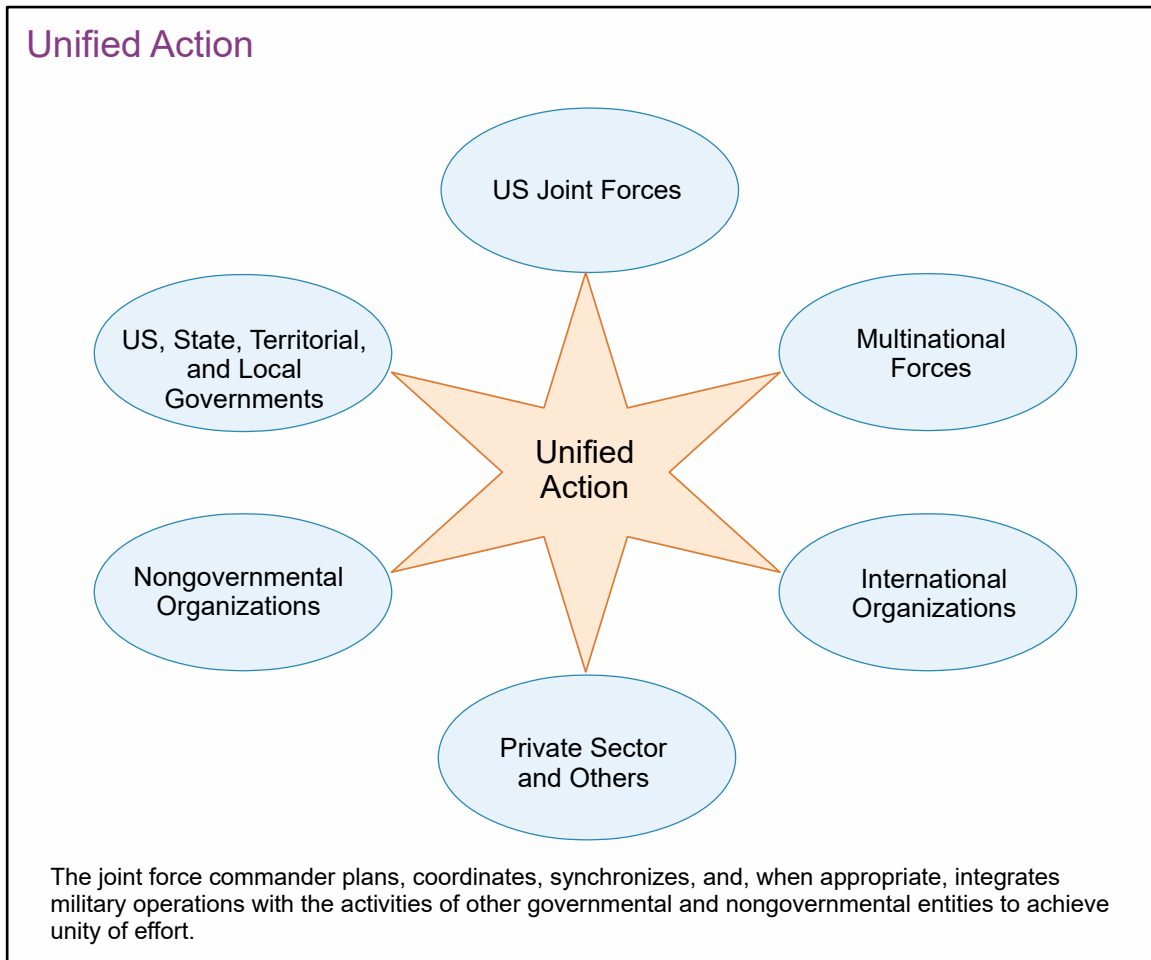
Figure I-3. Unified Action
