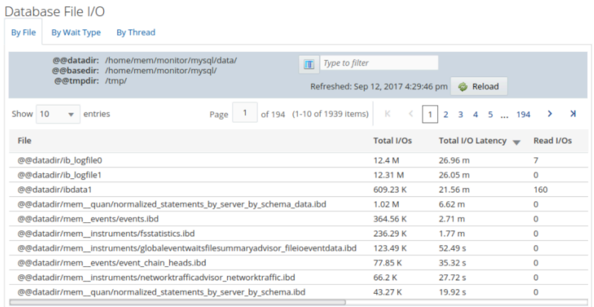
Figure 28.2 Database File I/O By File
