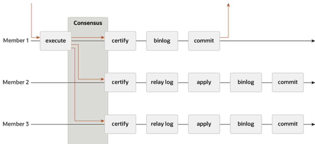
Figure 18.3 MySQL Group Replication Protocol
