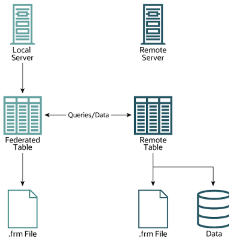
Figure 16.2 FEDERATED Table Structure
