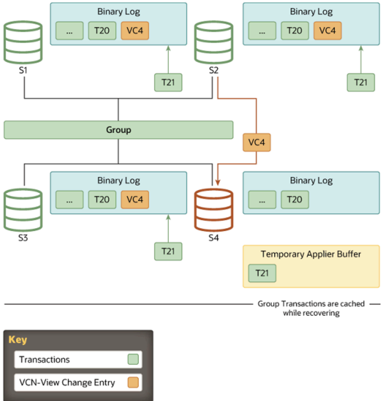
Figure 18.11 Queued Transactions
