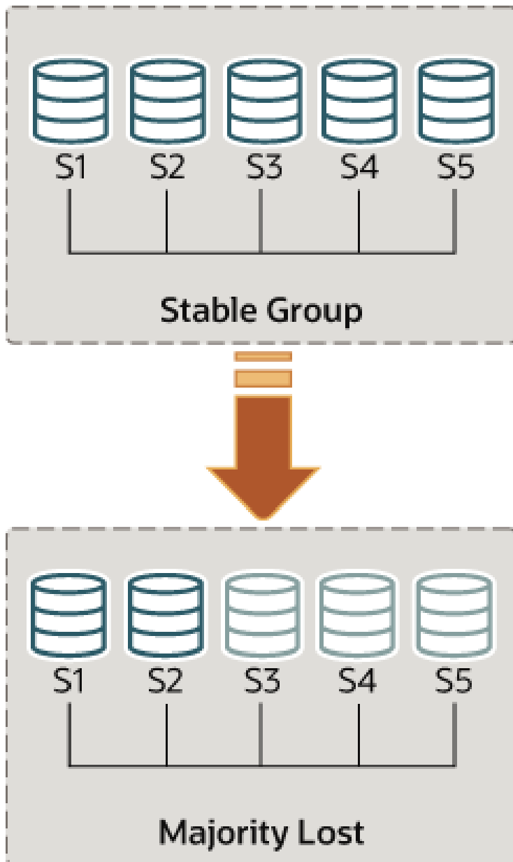
Figure 18.13 Losing Quorum
