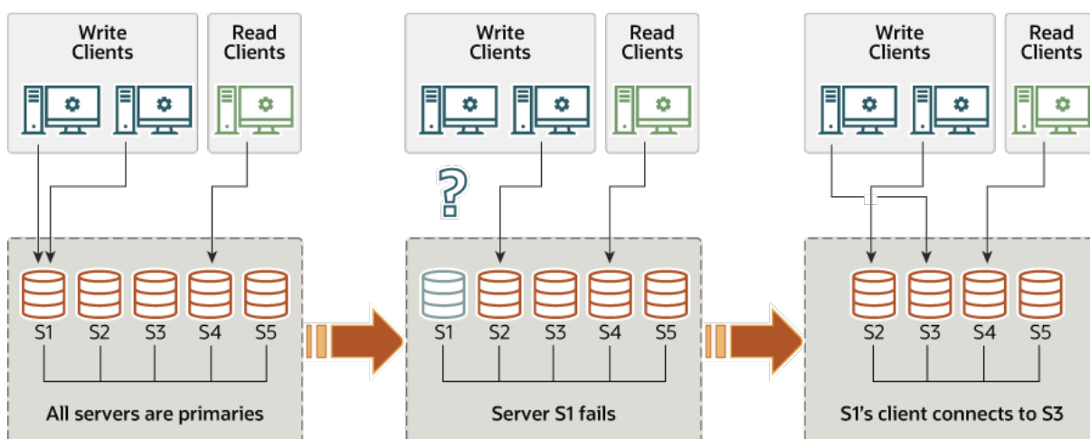
Figure 18.5 Client Failover
