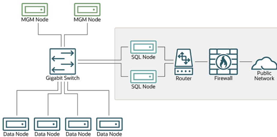
Figure 23.28 NDB Cluster with Hardware Firewall
