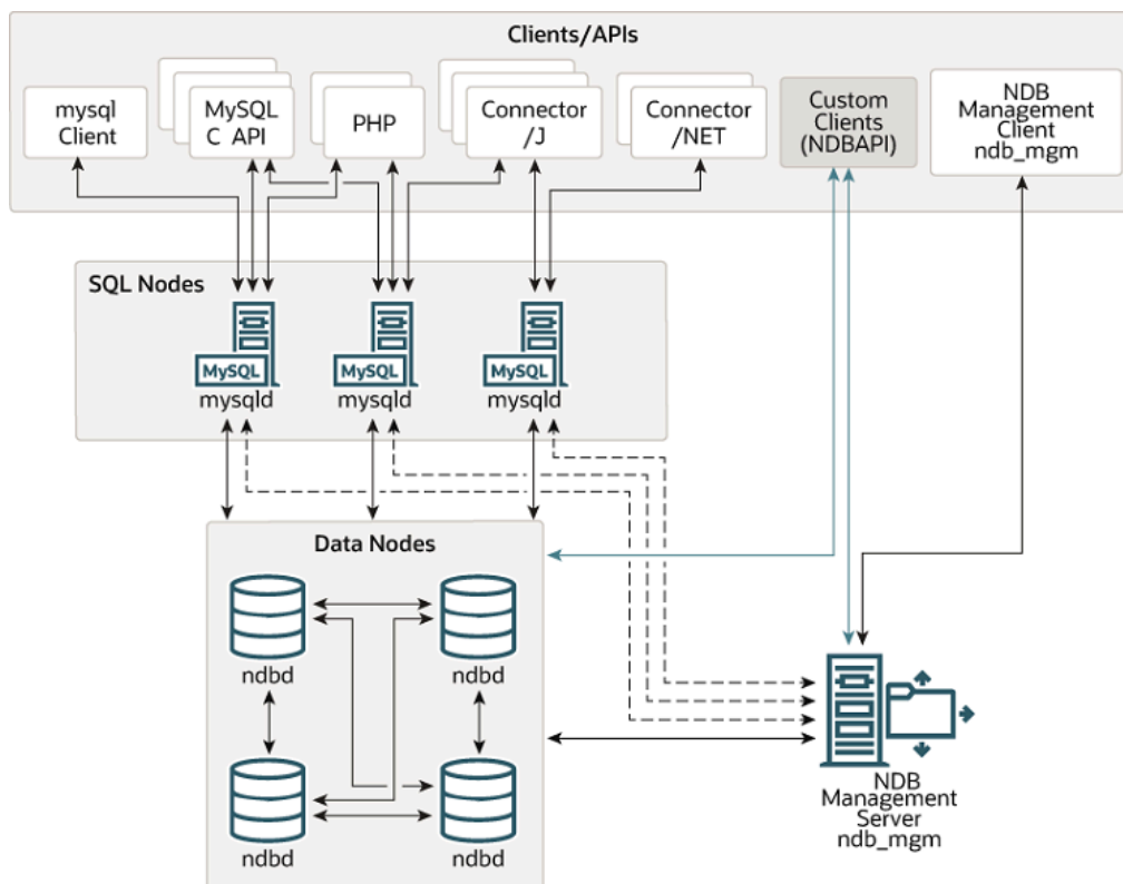
Figure 23.1 NDB Cluster Components
