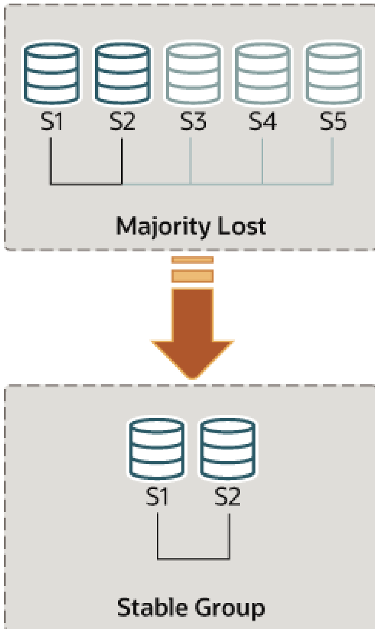
Figure 18.14 Forcing a New Membership
