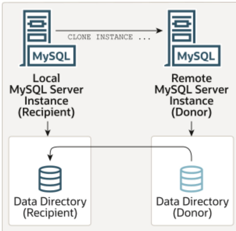
Figure 5.2 Remote Cloning Operation
