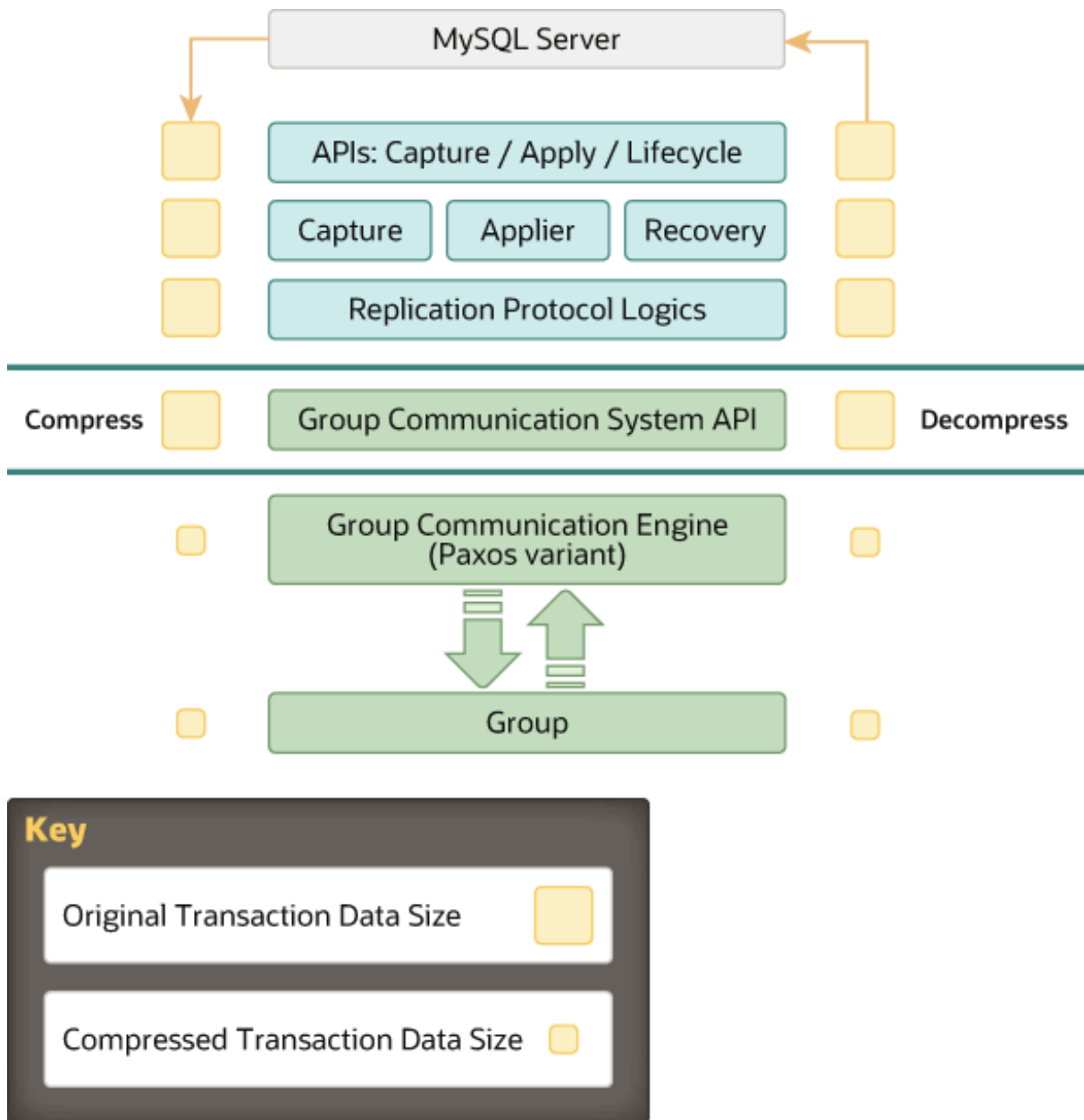
Figure 18.15 Compression Support
