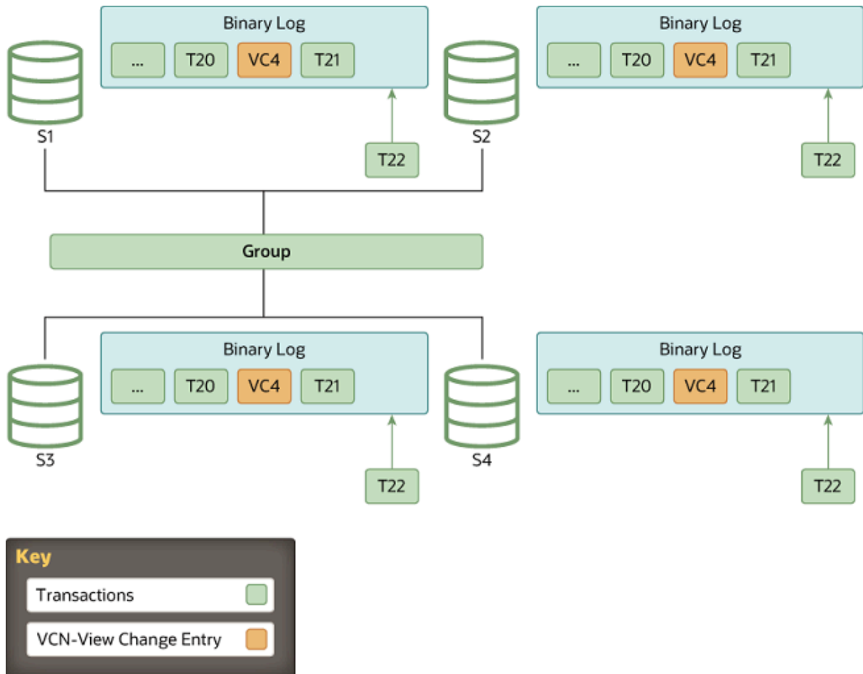
Figure 18.12 Instance Online
