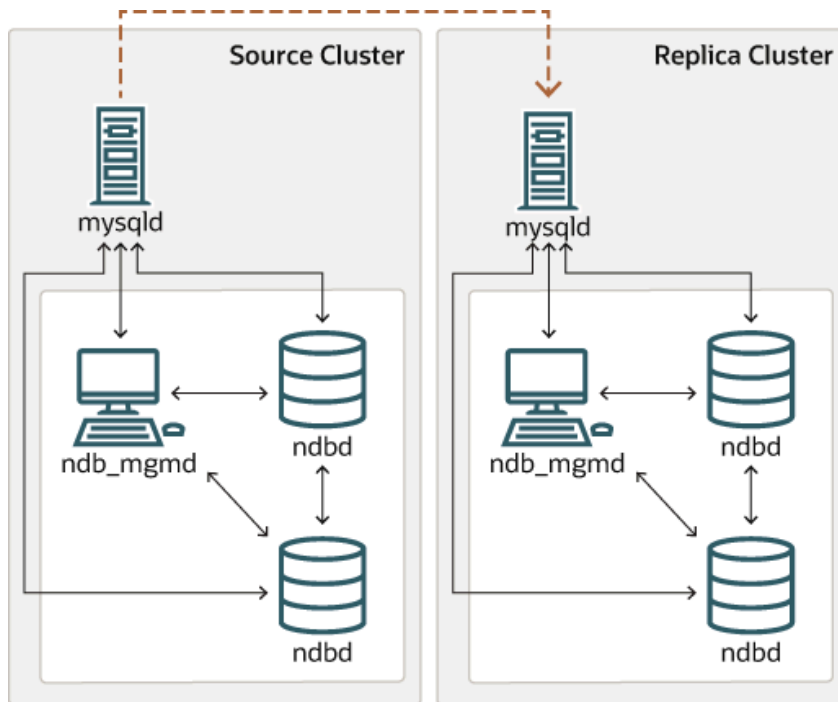
Figure 23.34 Replication Between SQL Nodes Connected Using IPv6
