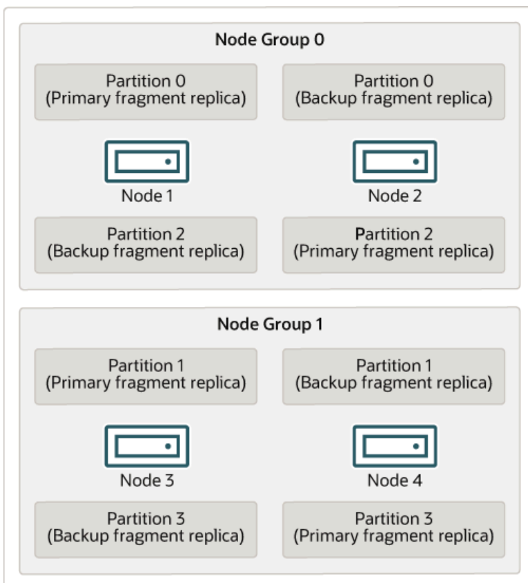
Figure 23.2 NDB Cluster with Two Node Groups
