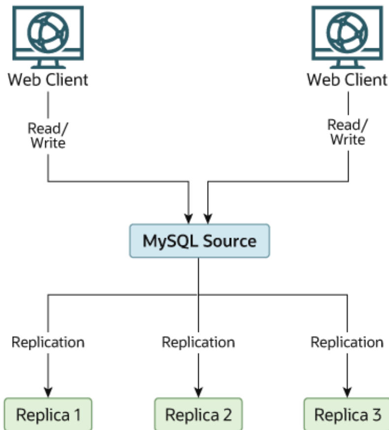
Figure 16.4 Redundancy Using Replication, Initial Structure
