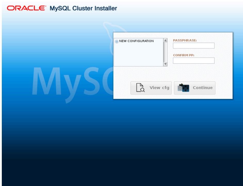
Figure 21.20 The NDB Cluster Auto-Installer Welcome screen, first run
