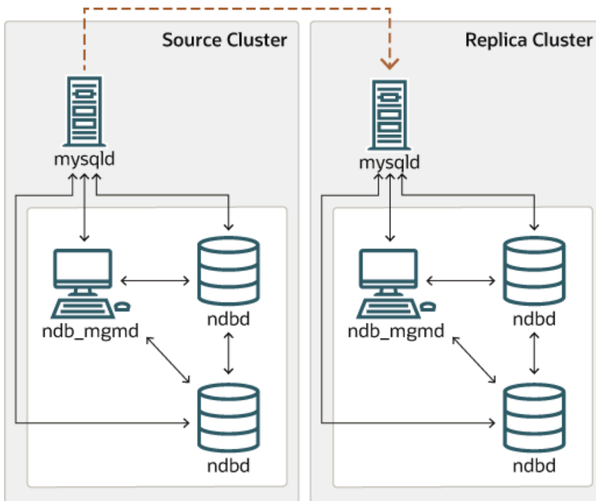
Figure 21.46 Replication Between SQL Nodes Connected Using IPv6
