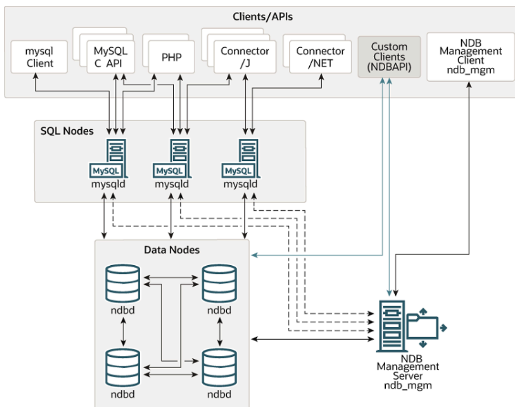
Figure 21.1 NDB Cluster Components
