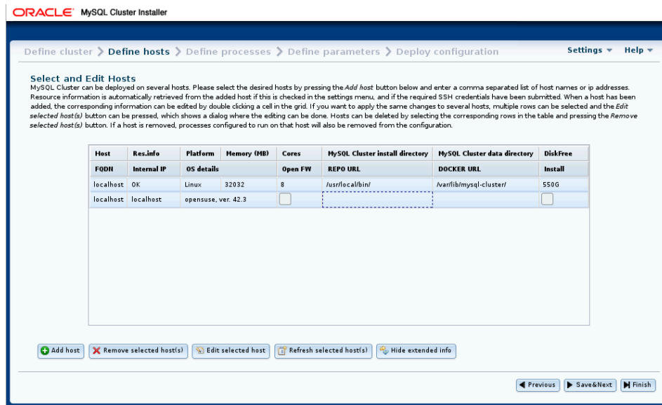
Figure 21.25 NDB Cluster Define Hosts screen, extended host info view
