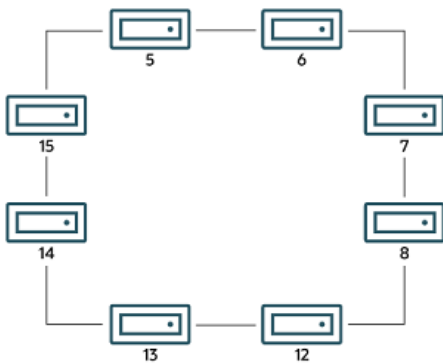
Figure 21.39 Circular Arrangement of NDB Cluster Nodes
