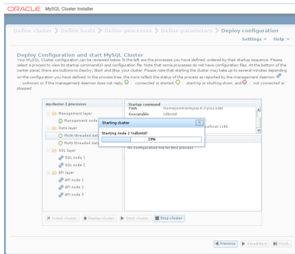
Figure 21.34 Cluster Startup Process with Progress Bar
