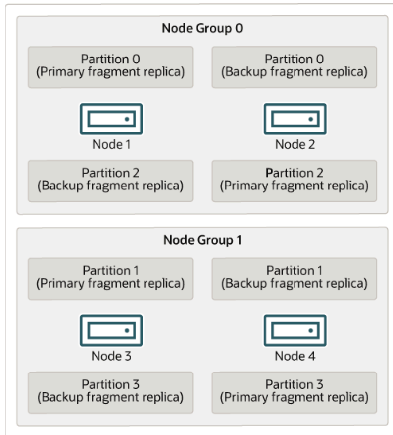
Figure 21.2 NDB Cluster with Two Node Groups
