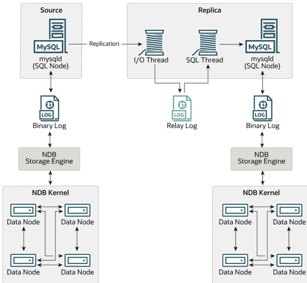
Figure 21.43 NDB Cluster-to-Cluster Replication Layout
