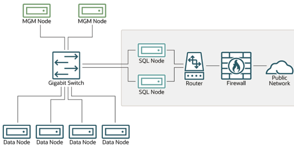
Figure 21.40 NDB Cluster with Hardware Firewall
