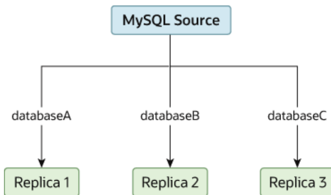
Figure 16.2 Replicating Databases to Separate Replicas
