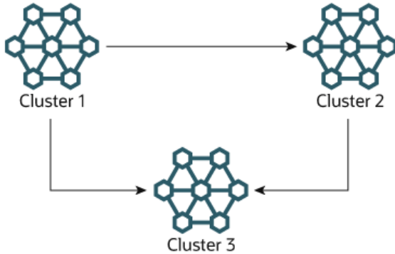
Figure 21.50 NDB Cluster Multi-Master Replication With 3 Sources
