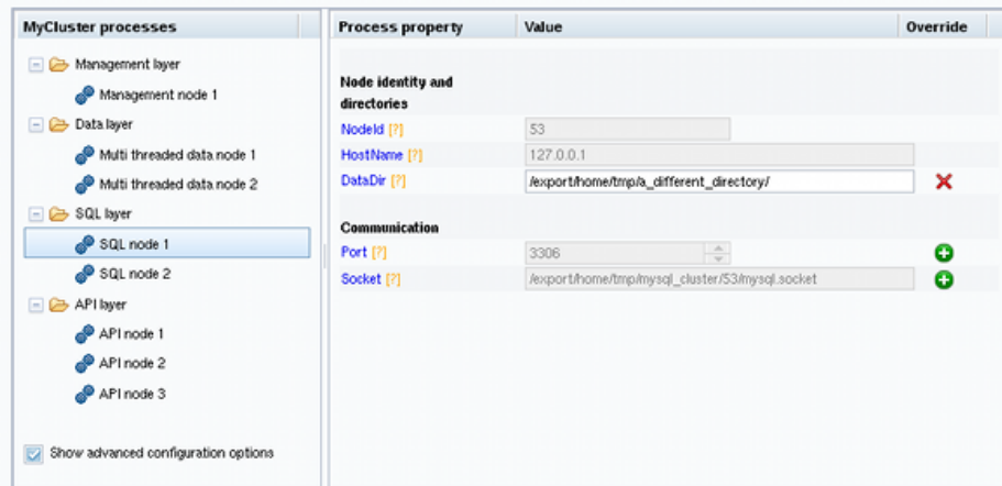
Figure 21.15 Define Attributes Detail, Overriding Attribute Default Value
