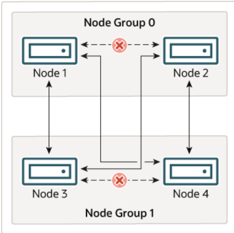
Figure 21.3 Nodes Required for a 2x2 NDB Cluster
