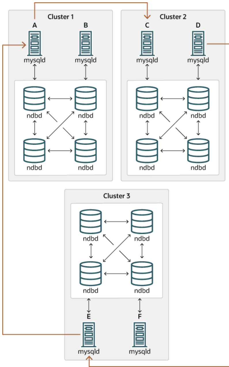
Figure 21.48 NDB Cluster Circular Replication with All Sources As Replicas
