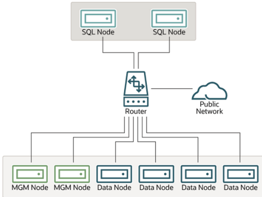
Figure 21.41 NDB Cluster with Software Firewalls
