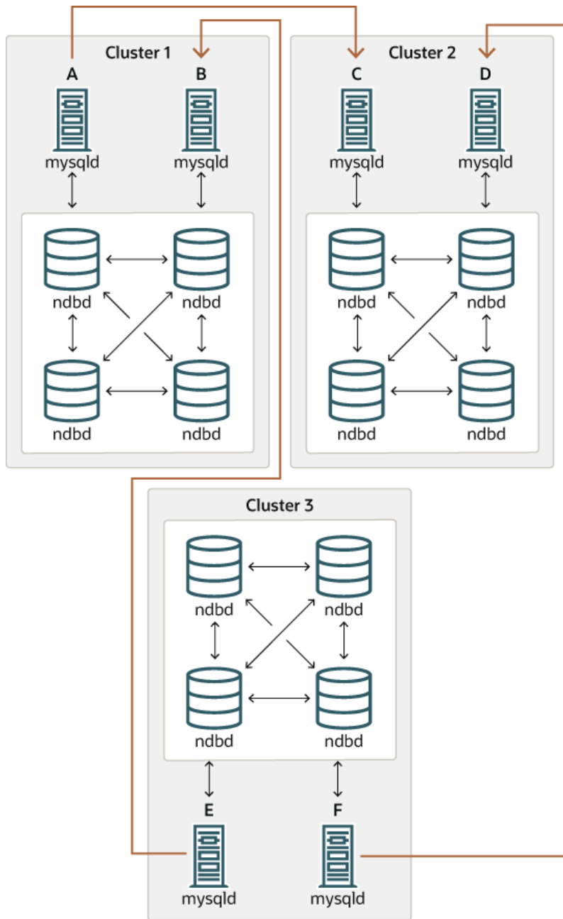
Figure 21.49 NDB Cluster Circular Replication Where Not All Sources Are Replicas
