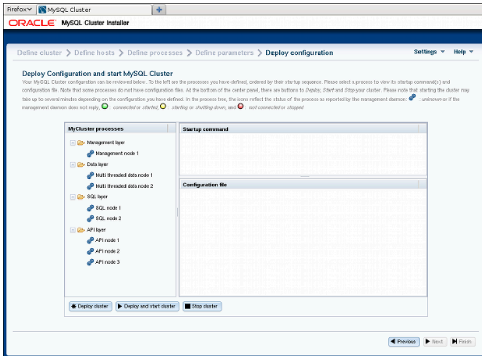
Figure 21.16 NDB Cluster Auto-Installer Deploy Cluster Configuration screen
