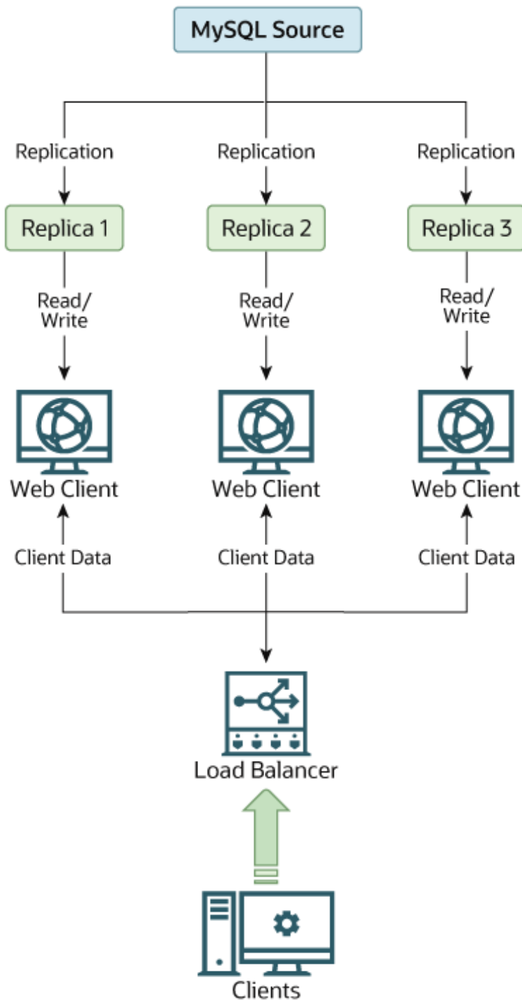
Figure 16.1 Using Replication to Improve Performance During Scale-Out
