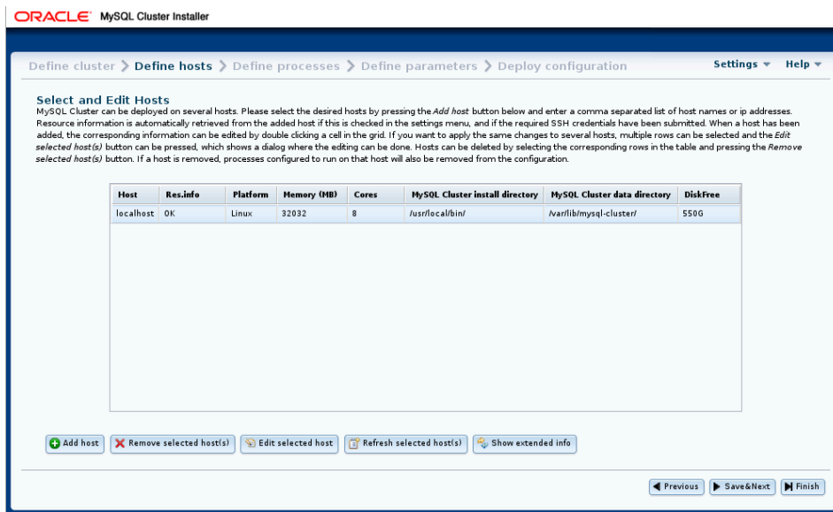
Figure 21.24 NDB Cluster Define Hosts screen, start
