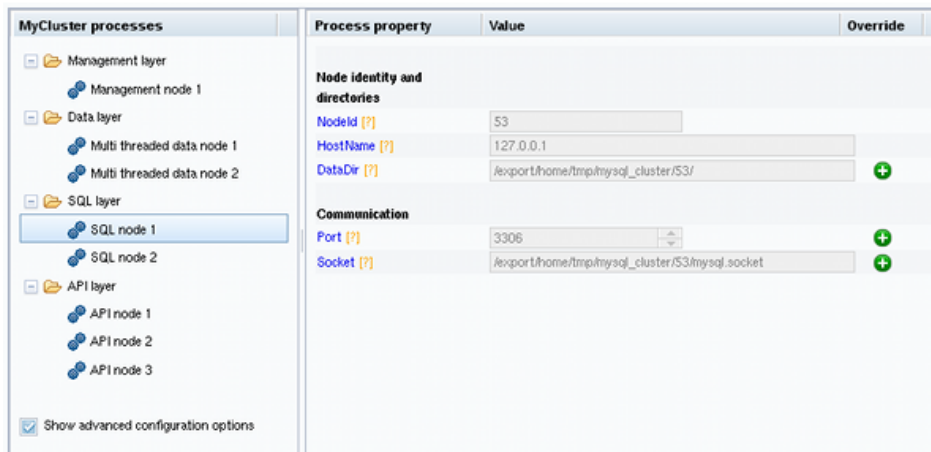
Figure 21.14 Define Attributes Detail With SQL Process Attributes
