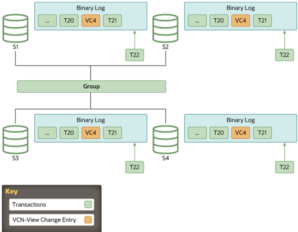
Figure 17.14 Instance Online
