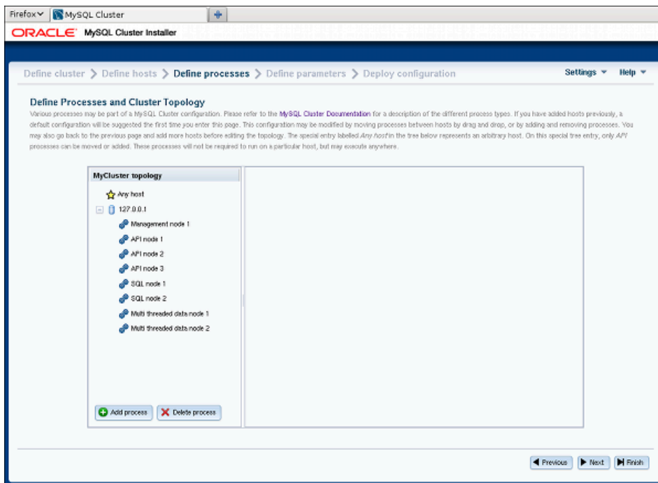
Figure 21.11 NDB Cluster Auto-Installer Define Processes dialog
