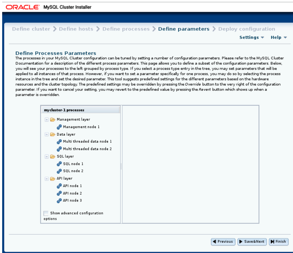
Figure 21.30 NDB Cluster Auto-Installer Define Parameters screen
