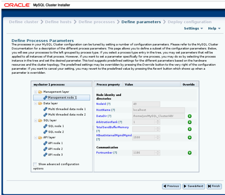
Figure 21.31 Define Parameters—Process Attributes
