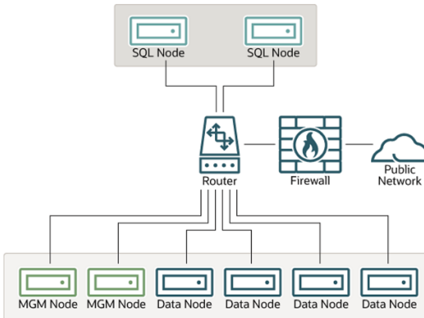
Figure 21.42 NDB Cluster with a Combination of Hardware and Software Firewalls
