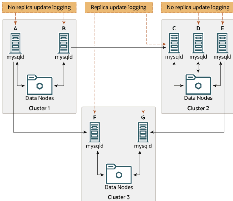
Figure 21.51 NDB Cluster Multi-Source Replication, With MySQL Servers
