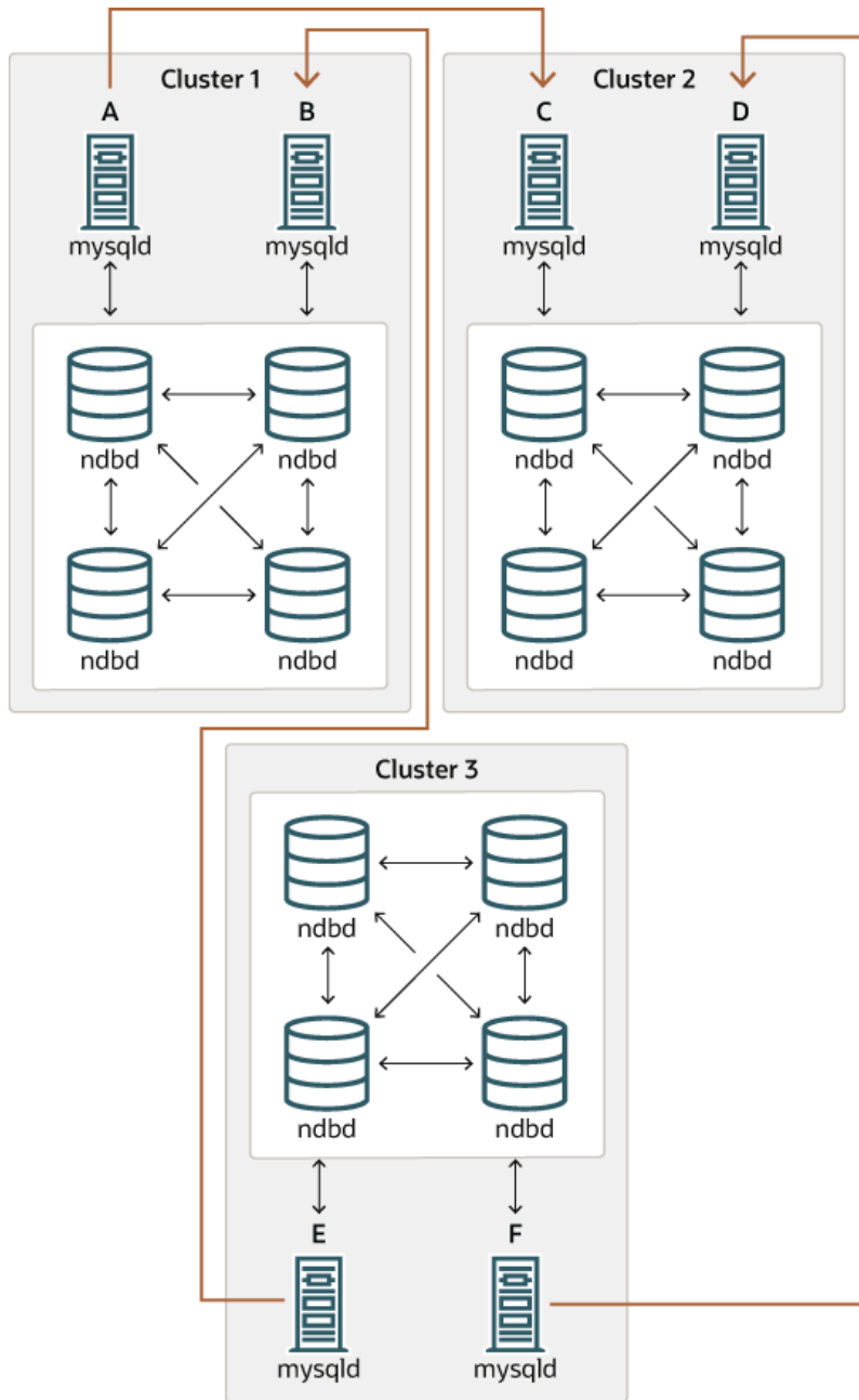
Figure 21.45 NDB Cluster Circular Replication Where Not All Sources Are Replicas
