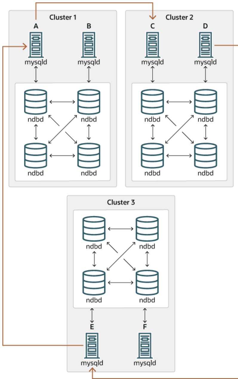
Figure 21.44 NDB Cluster Circular Replication With All Sources As Replicas
