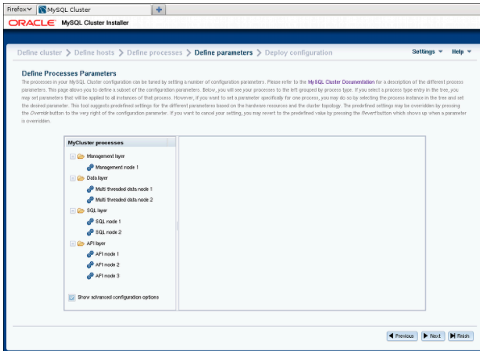
Figure 21.13 NDB Cluster Auto-Installer Define Attributes screen
