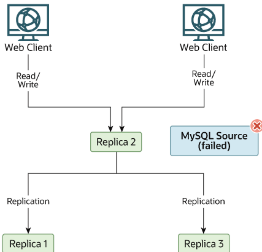
Figure 16.5 Redundancy Using Replication, After Source Failure
