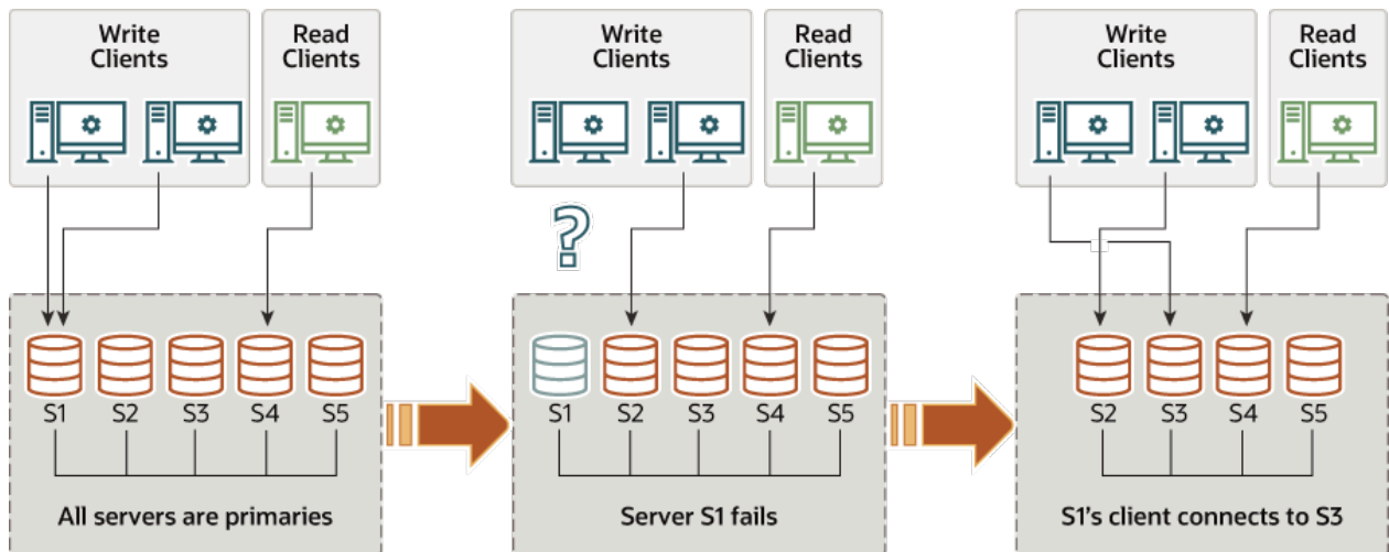
Figure 17.6 Client Failover
