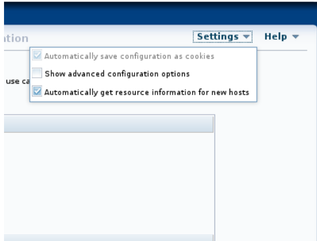
Figure 21.18 NDB Cluster Auto-Installer Settings menu
