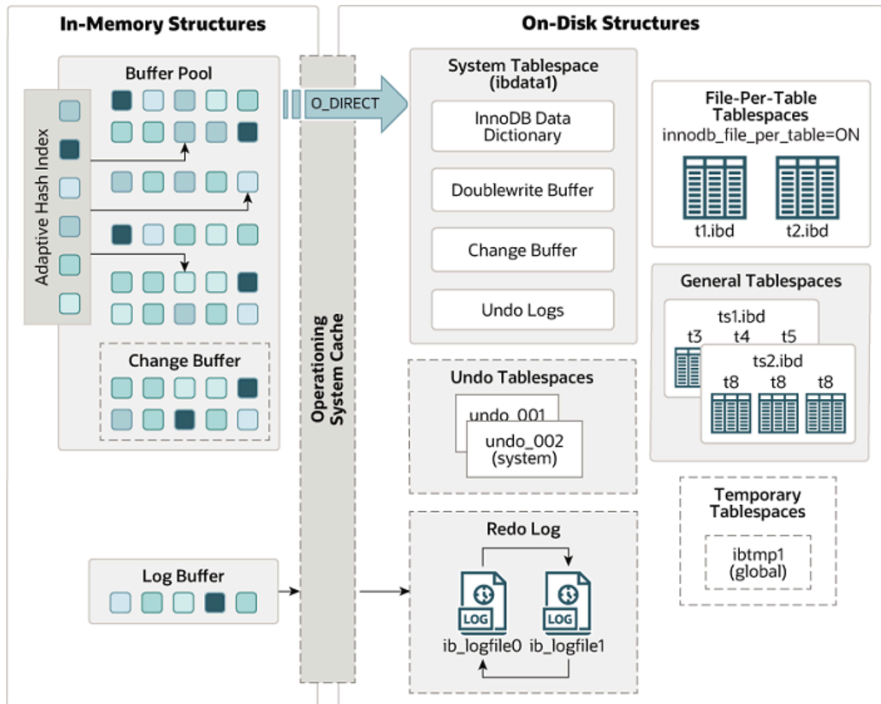
Figure 14.1 InnoDB Architecture
