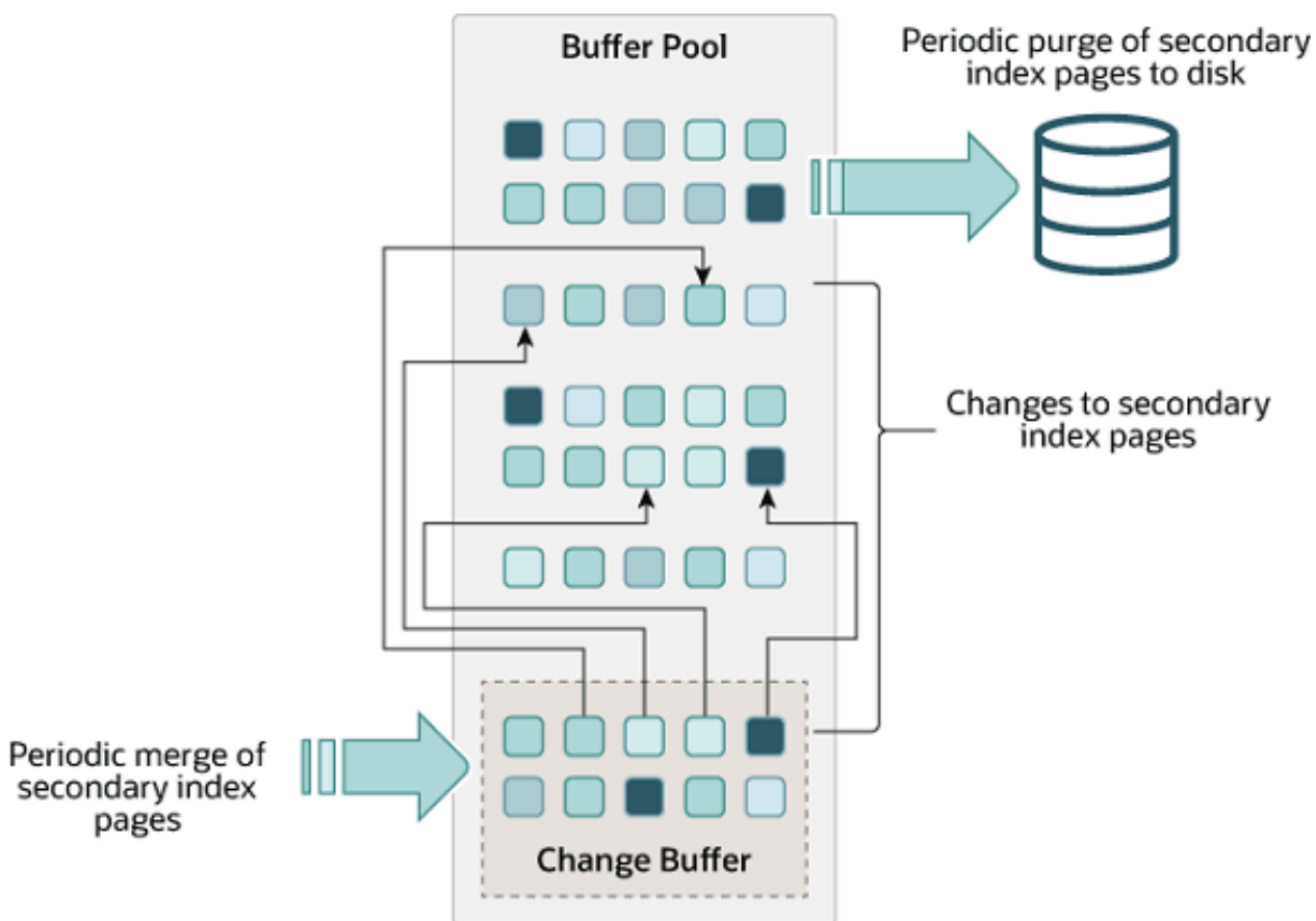
Figure 14.3 Change Buffer
