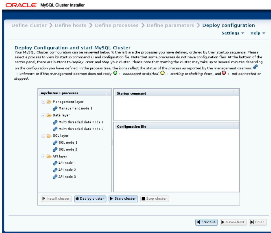
Figure 21.32 NDB Cluster Auto-Installer Deploy Configuration screen
