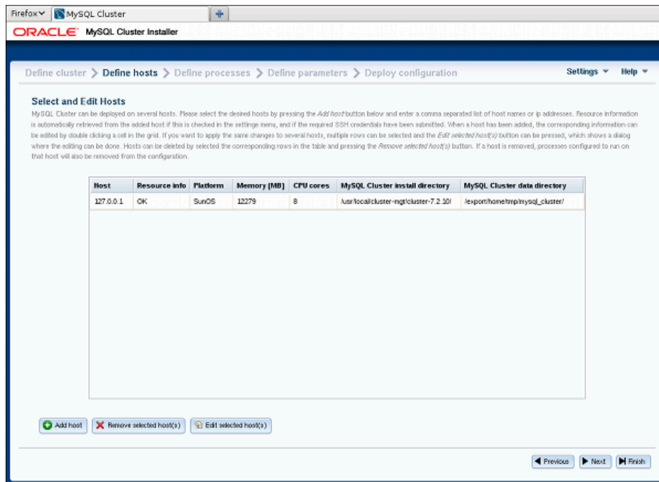
Figure 21.9 NDB Cluster Define Hosts screen
