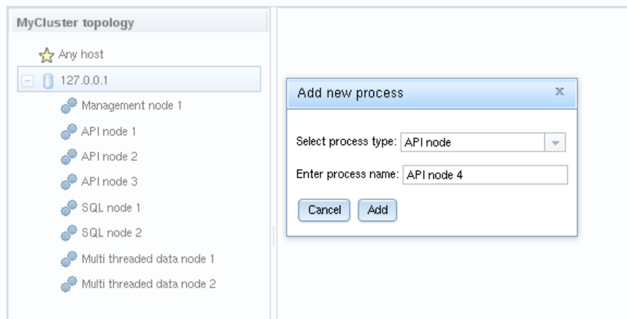
Figure 21.12 NDB Cluster Auto-Installer Add Process Dialog
