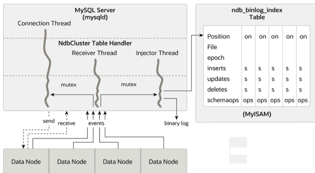
Figure 21.47 The Replication Source Cluster
