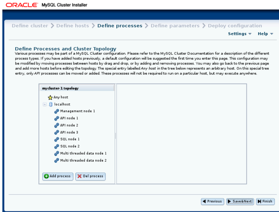
Figure 21.28 NDB Cluster Auto-Installer Define Processes dialog
