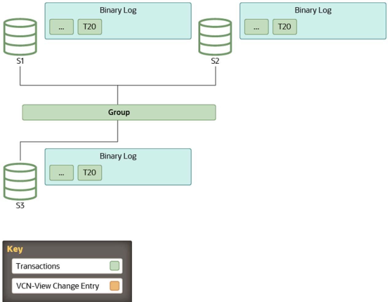
Figure 17.10 Stable Group
