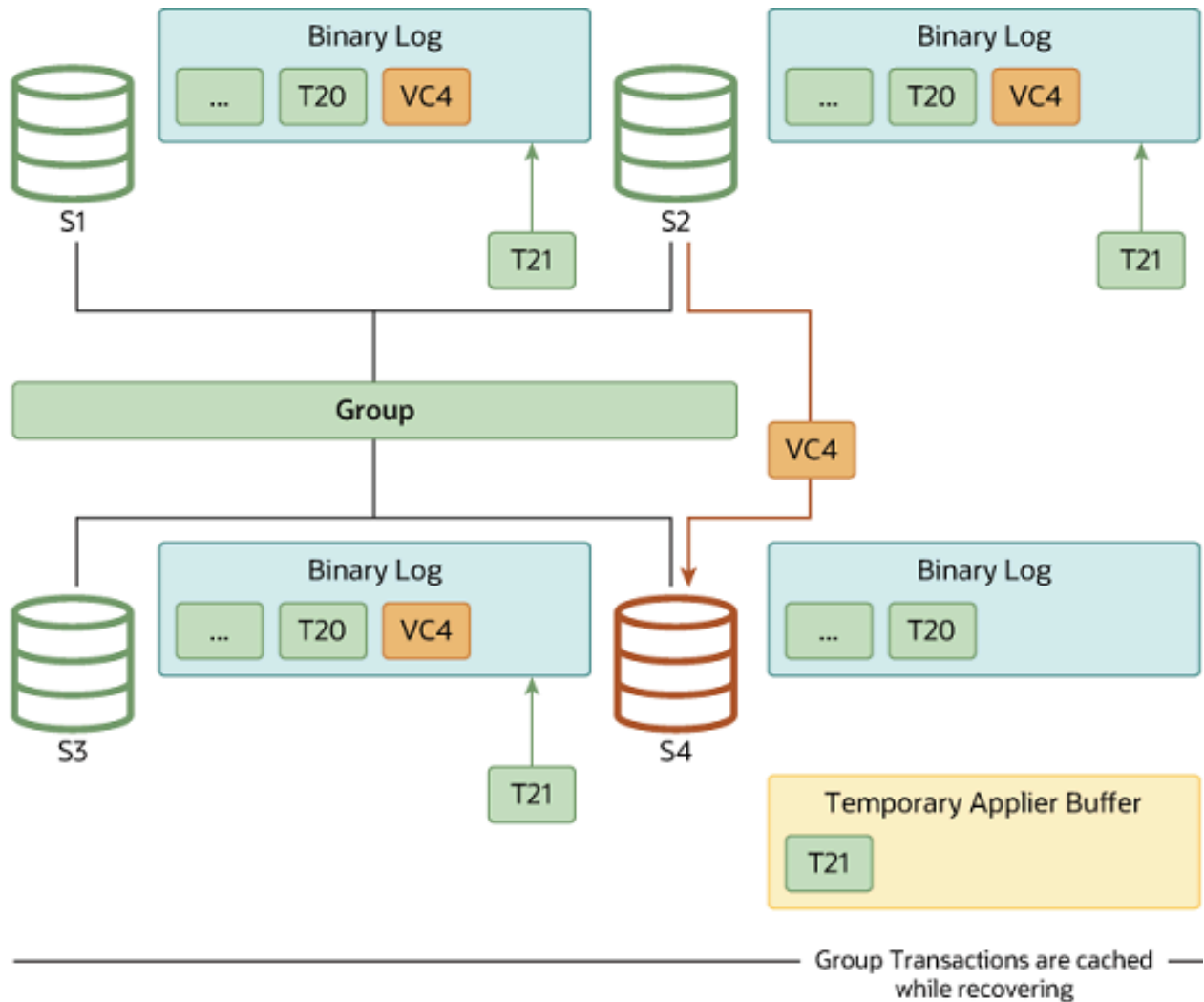
Figure 17.13 Queued Transactions
