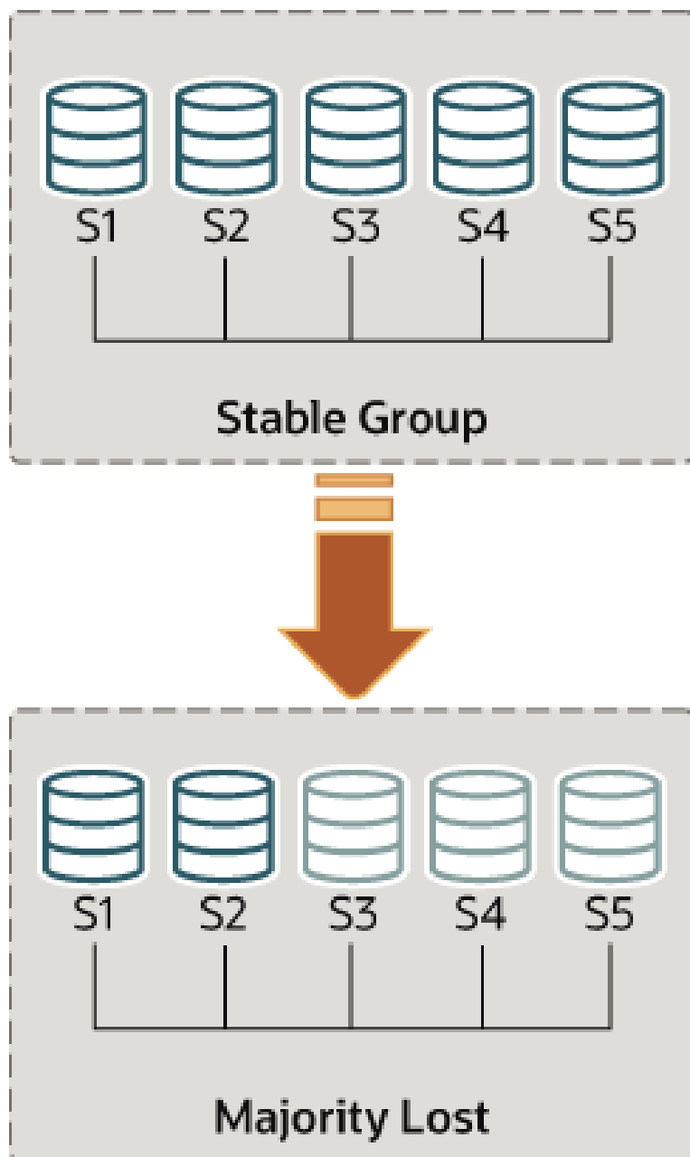
Figure 17.7 Losing Quorum
