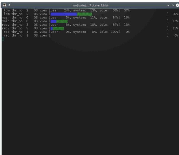
Figure 5.1 ndb_top Running in Terminal
