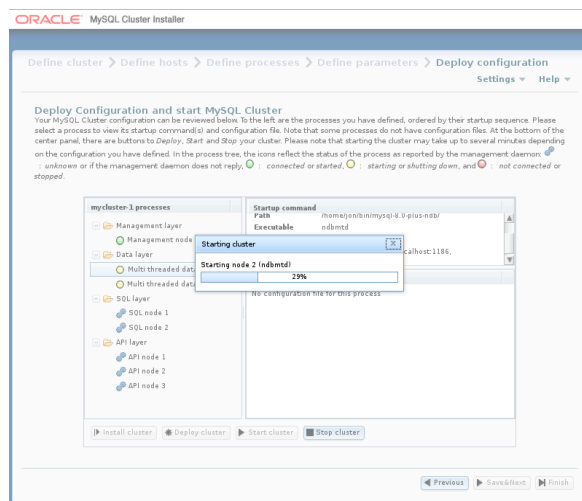
Figure 3.19 Cluster Startup Process with Progress Bar
