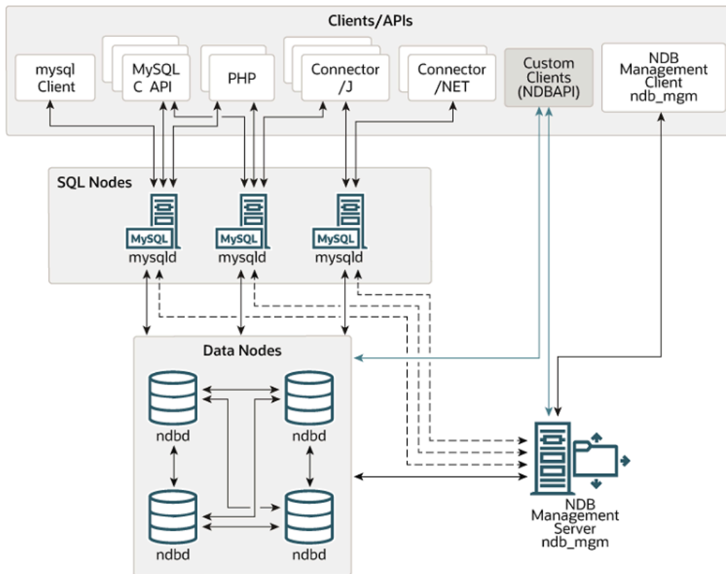
Figure 2.1 NDB Cluster Components
