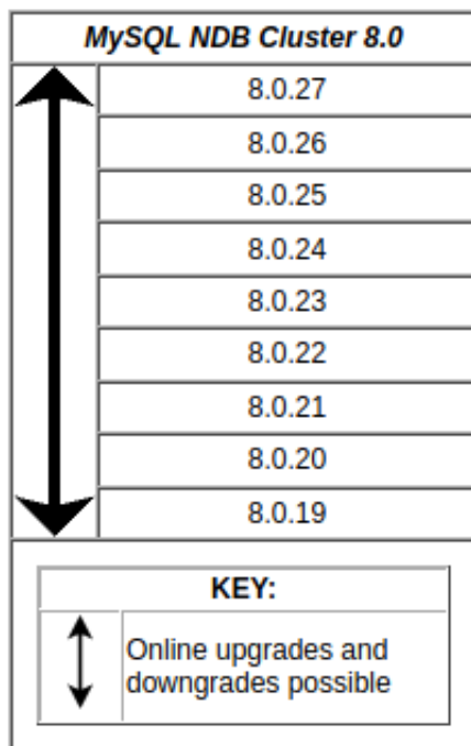
Figure 3.2 NDB Cluster Upgrade and Downgrade Compatibility, MySQL NDB Cluster 8.0
