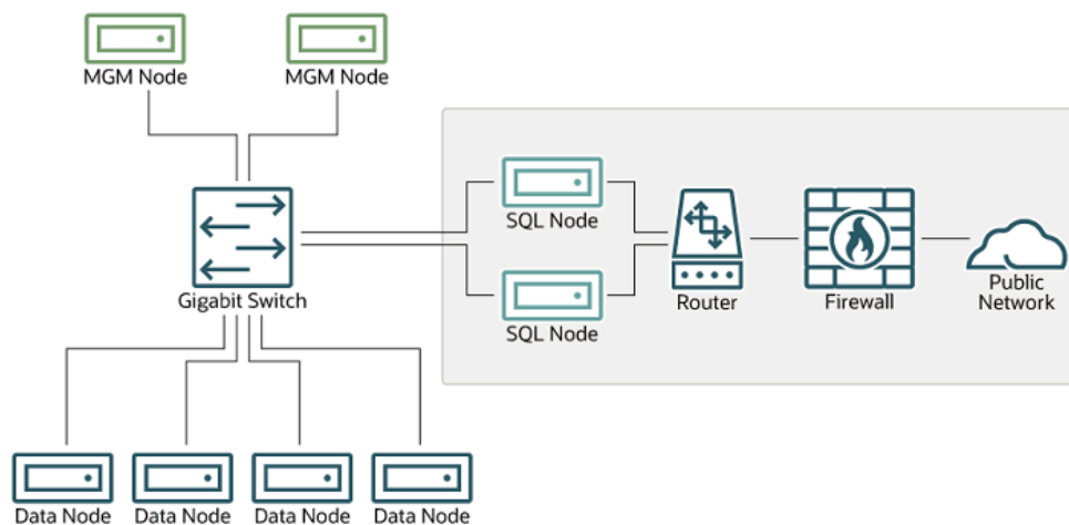
Figure 6.2 NDB Cluster with Hardware Firewall
