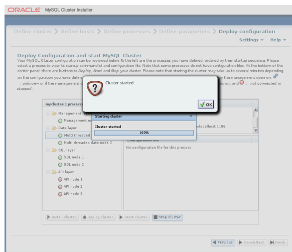
Figure 3.20 Cluster Startup, Process Completed Dialog
