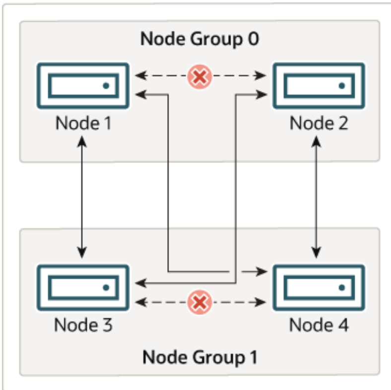
Figure 2.3 Nodes Required for a 2x2 NDB Cluster
