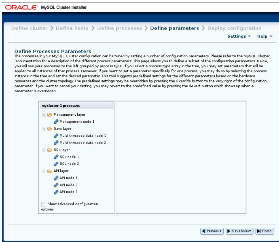
Figure 3.15 NDB Cluster Auto-Installer Define Parameters screen
