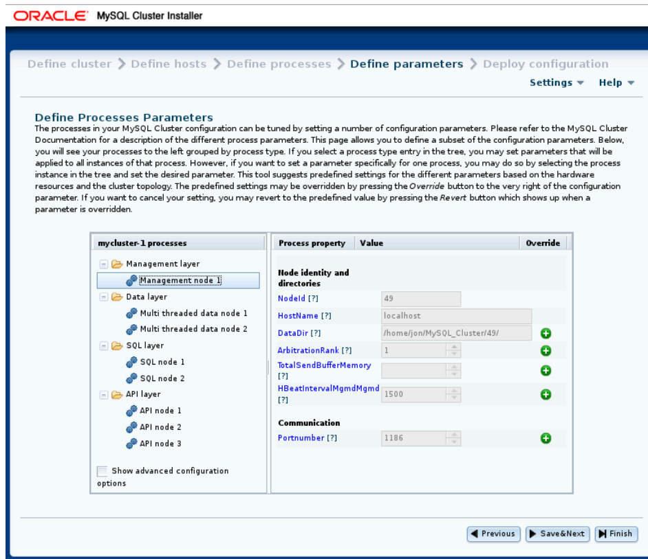
Figure 3.16 Define Parameters—Process Attributes
