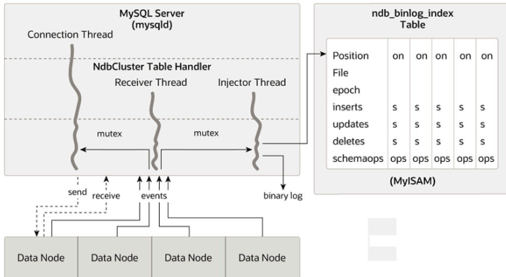
Figure 7.5 The Replication Source Cluster
