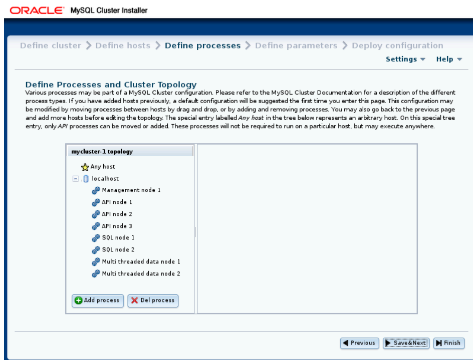
Figure 3.13 NDB Cluster Auto-Installer Define Processes dialog
