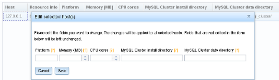
Figure 3.7 NDB Cluster Auto-Installer Edit Hosts dialog
