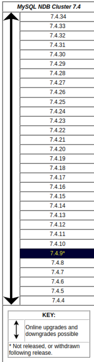
Figure 3.2 NDB Cluster Upgrade and Downgrade Compatibility, MySQL NDB Cluster 7.4
