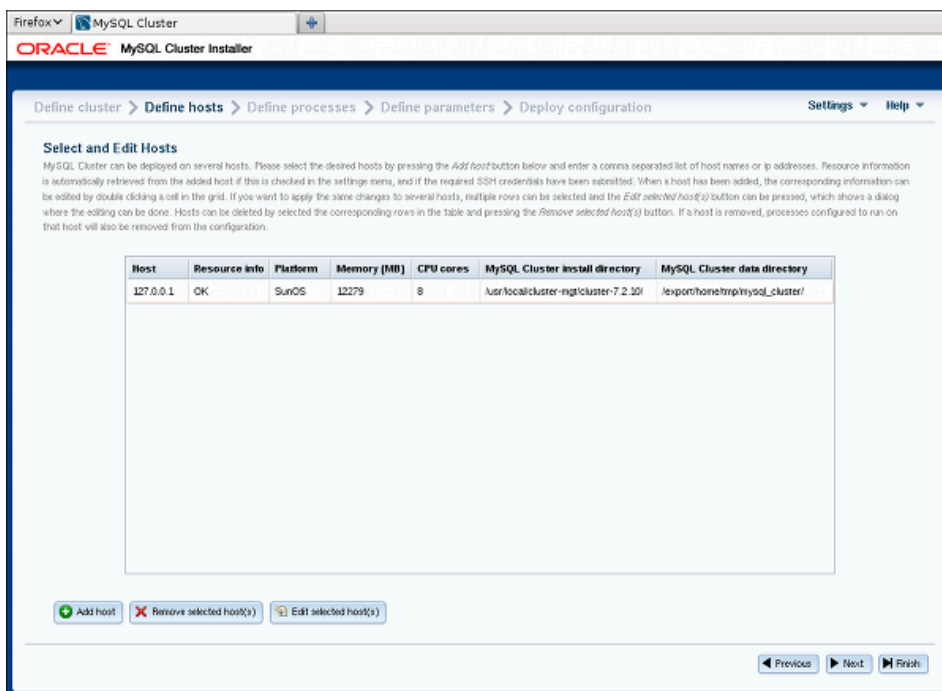
Figure 3.6 NDB Cluster Define Hosts screen
