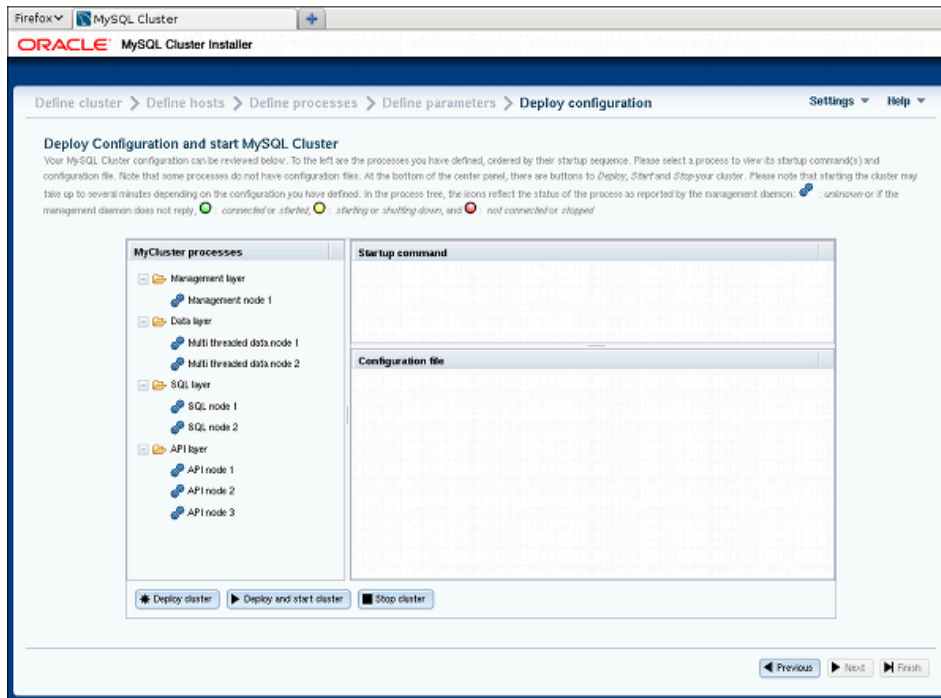
Figure 3.13 NDB Cluster Auto-Installer Deploy Cluster Configuration screen
