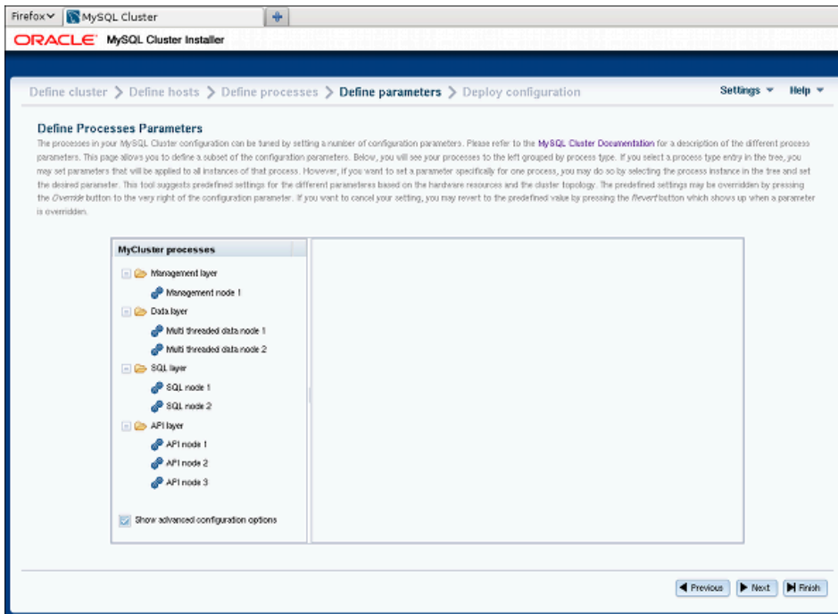
Figure 3.10 NDB Cluster Auto-Installer Define Attributes screen
