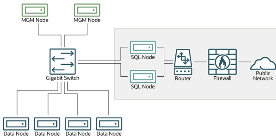
Figure 6.2 NDB Cluster with Hardware Firewall
