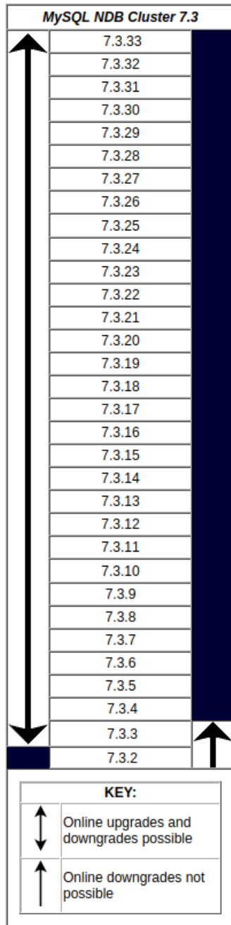
Figure 3.3 NDB Cluster Upgrade and Downgrade Compatibility, MySQL NDB Cluster 7.3
