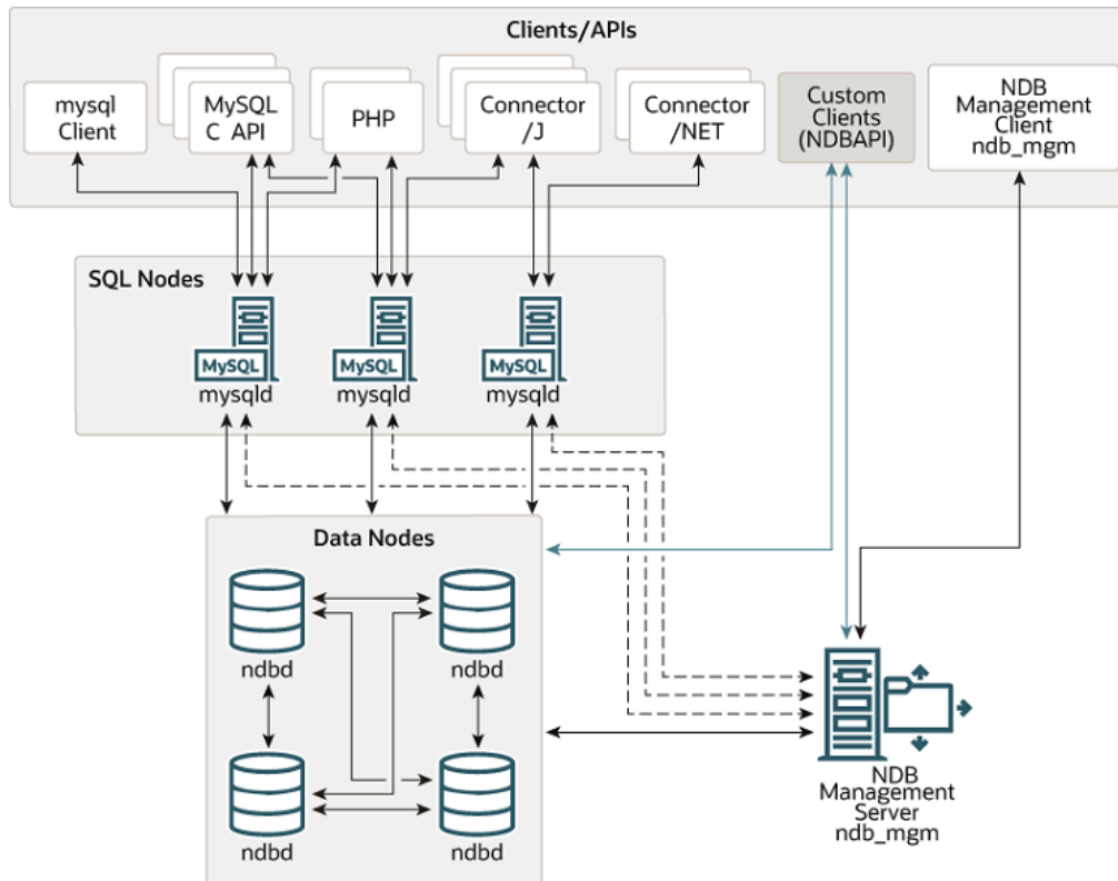
Figure 2.1 NDB Cluster Components
