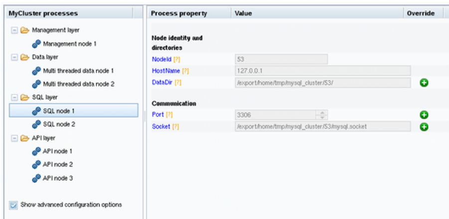
Figure 3.11 Define Attributes Detail With SQL Process Attributes
