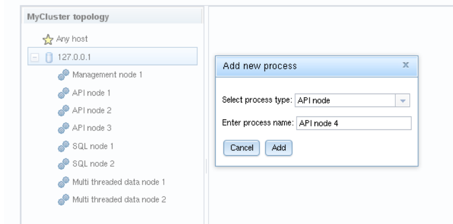
Figure 3.9 NDB Cluster Auto-Installer Add Process Dialog
