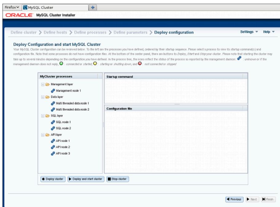
Figure 3.13 NDB Cluster Auto-Installer Deploy Cluster Configuration screen
