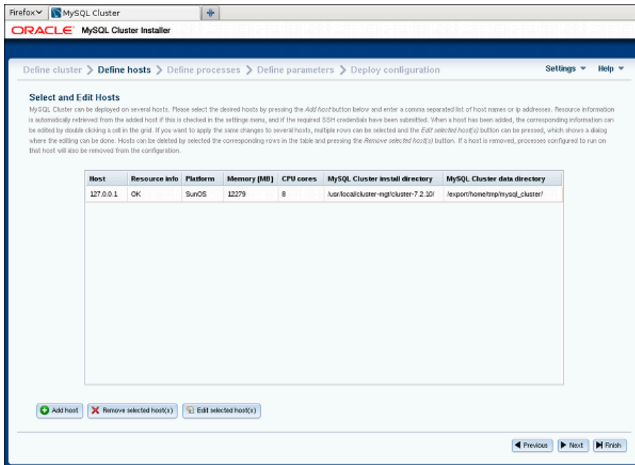
Figure 3.6 NDB Cluster Define Hosts screen
