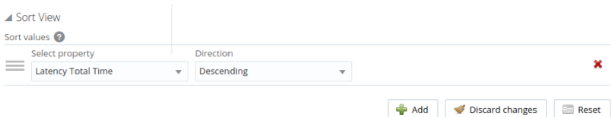
Figure 31.10 Sort View
