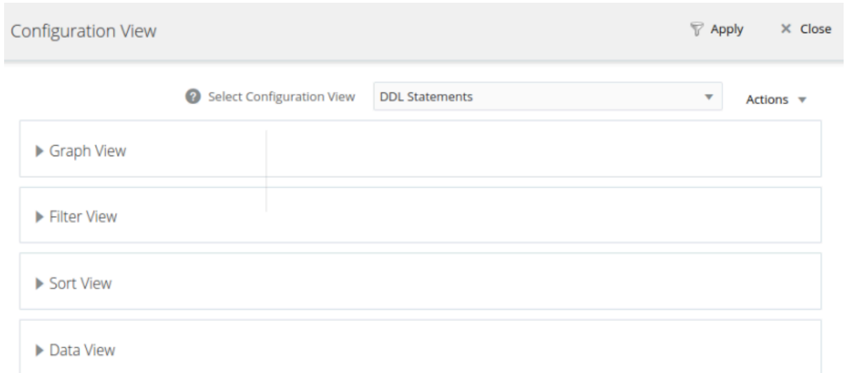
Figure 31.7 Configuration View
