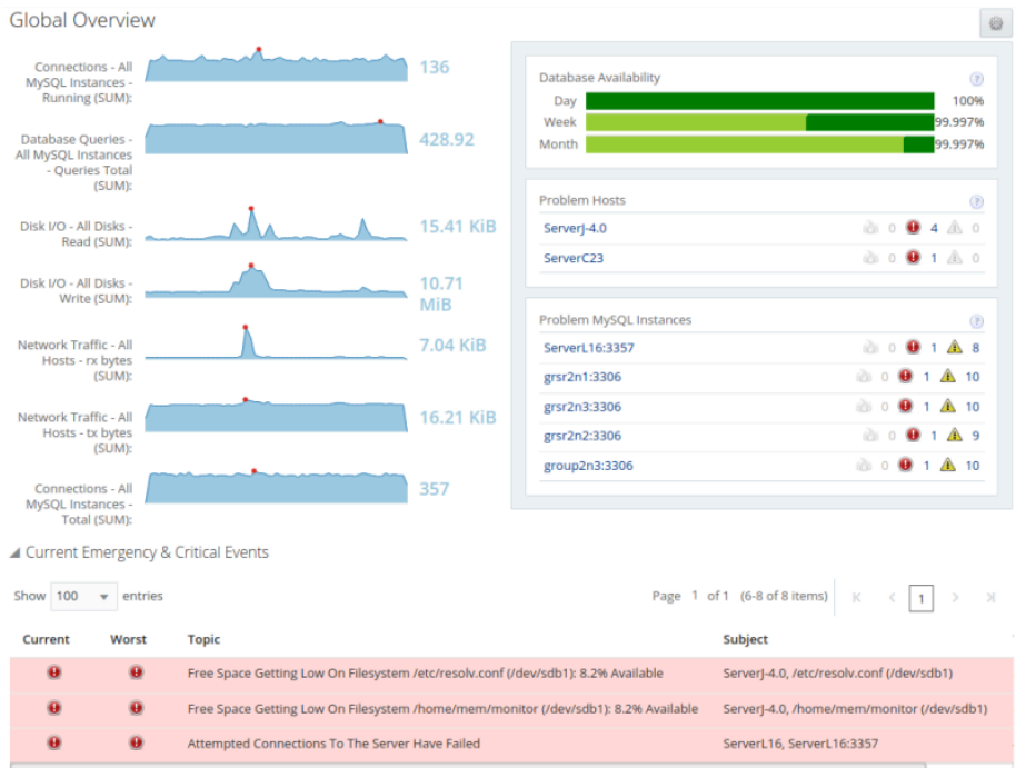
Figure 24.1 Global Overview
