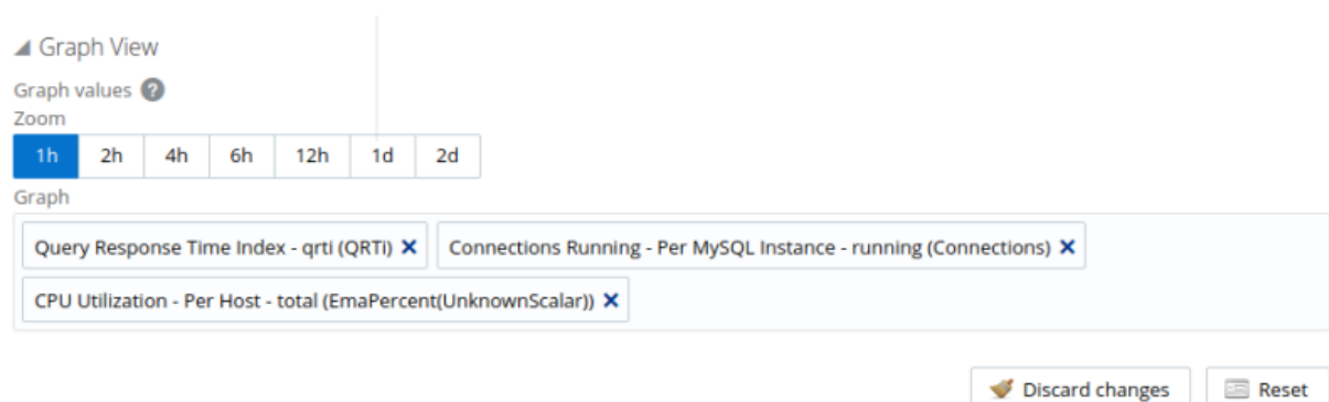
Figure 31.8 Graph View
