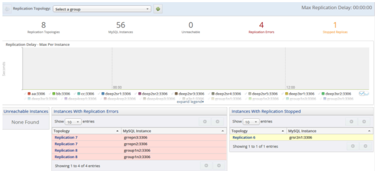
Figure 27.1 Replication Overview
