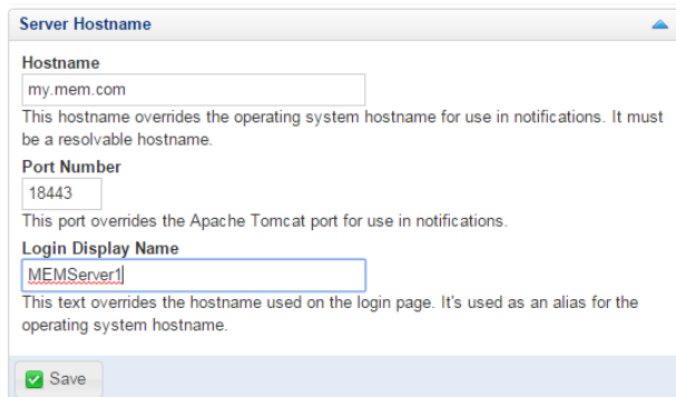
Figure 14.1 Server Hostname
