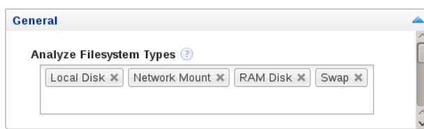
Figure 20.6 Filesystem - General
