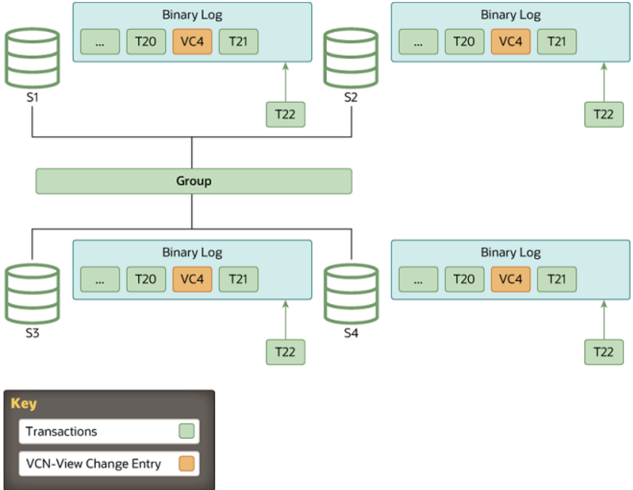
Figure 18.12 Instance Online
