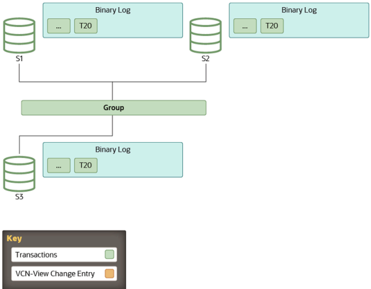
Figure 18.8 Stable Group
