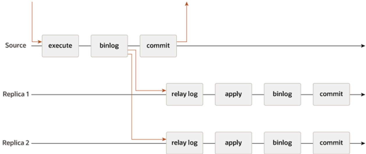
Figure 18.1 MySQL Asynchronous Replication
