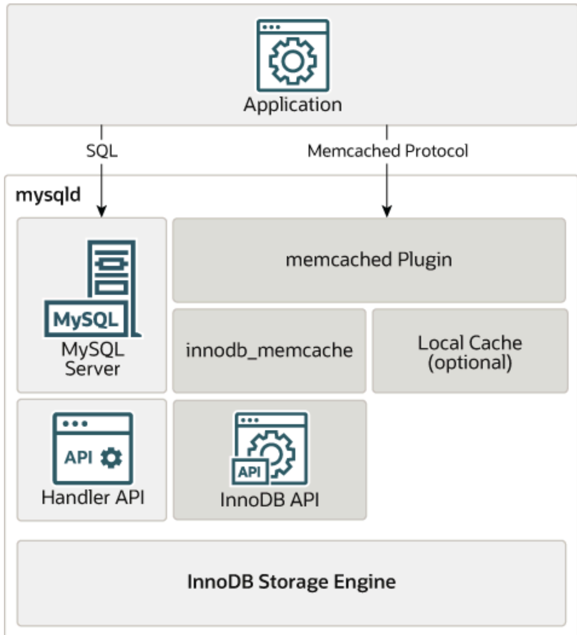
Figure 15.4 MySQL Server with Integrated memcached Server
