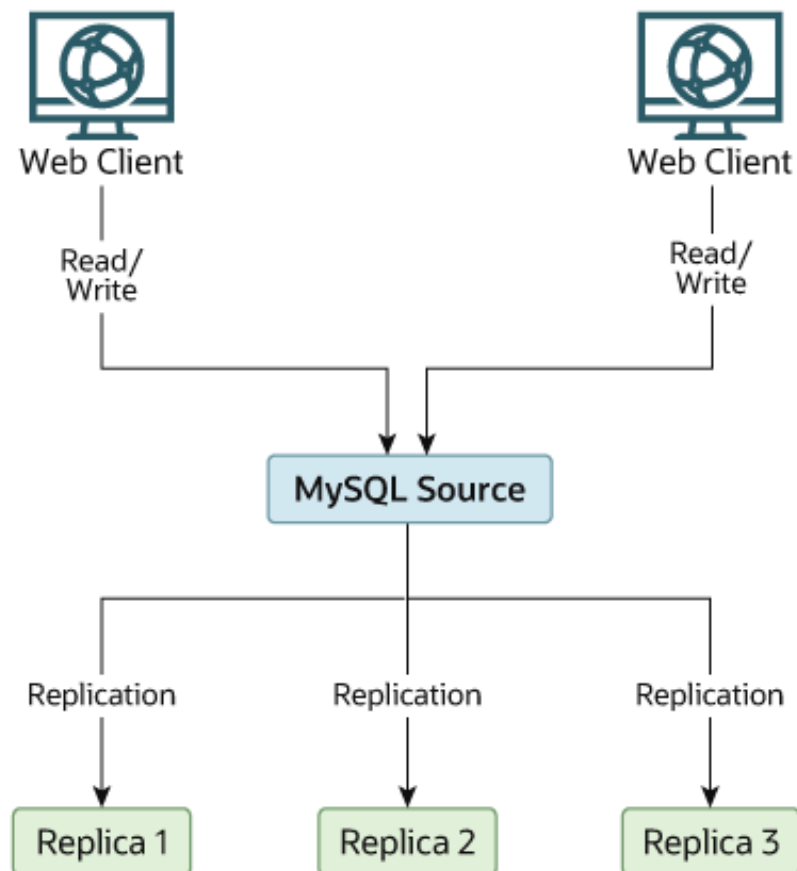
Figure 17.4 Redundancy Using Replication, Initial Structure
