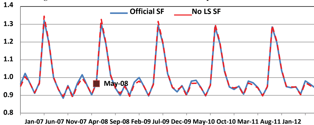
Figure 3: Level Shift Effect on UN Male Teen Multiplicative Seasonal Factors
