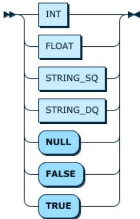
Figure 11.37 Literal
