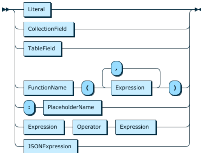
Figure 11.38 Expression
