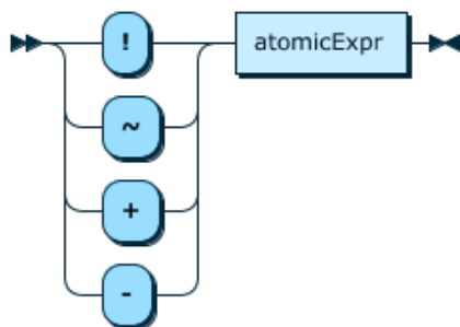
Figure 12.14 unaryOp
