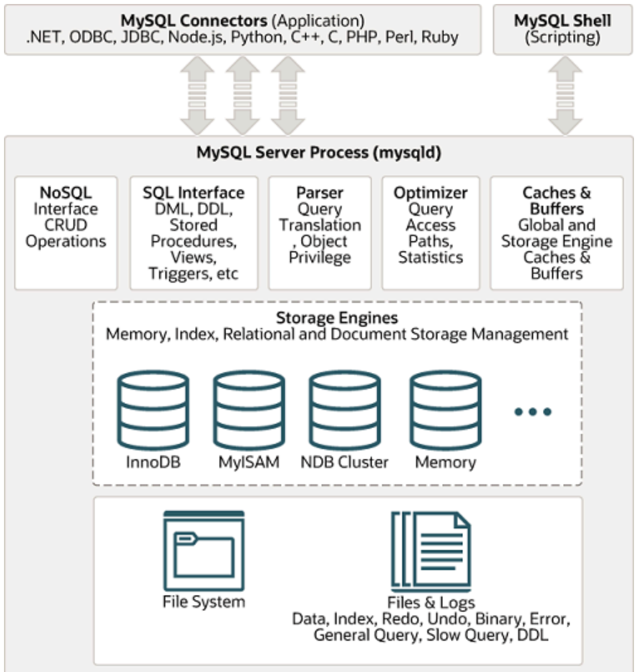
Figure 16.3 MySQL Architecture with Pluggable Storage Engines
