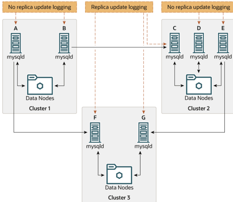
Figure 23.39 NDB Cluster Multi-Source Replication, With MySQL Servers
