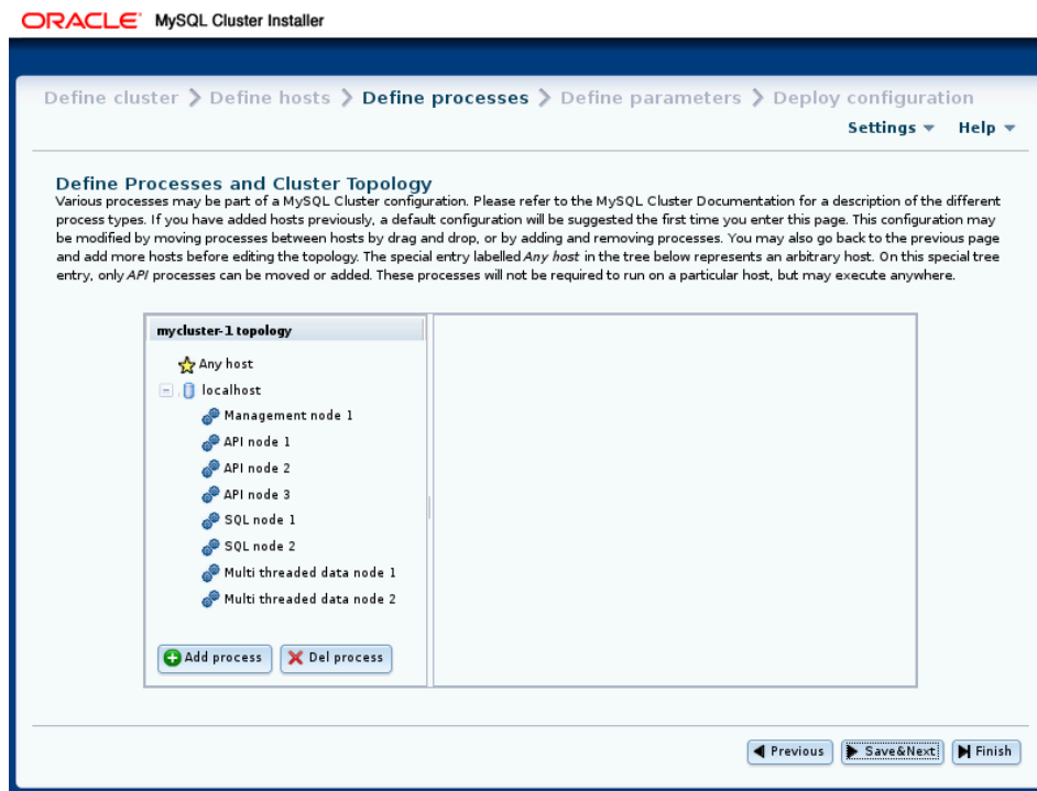
Figure 23.16 NDB Cluster Auto-Installer Define Processes dialog
