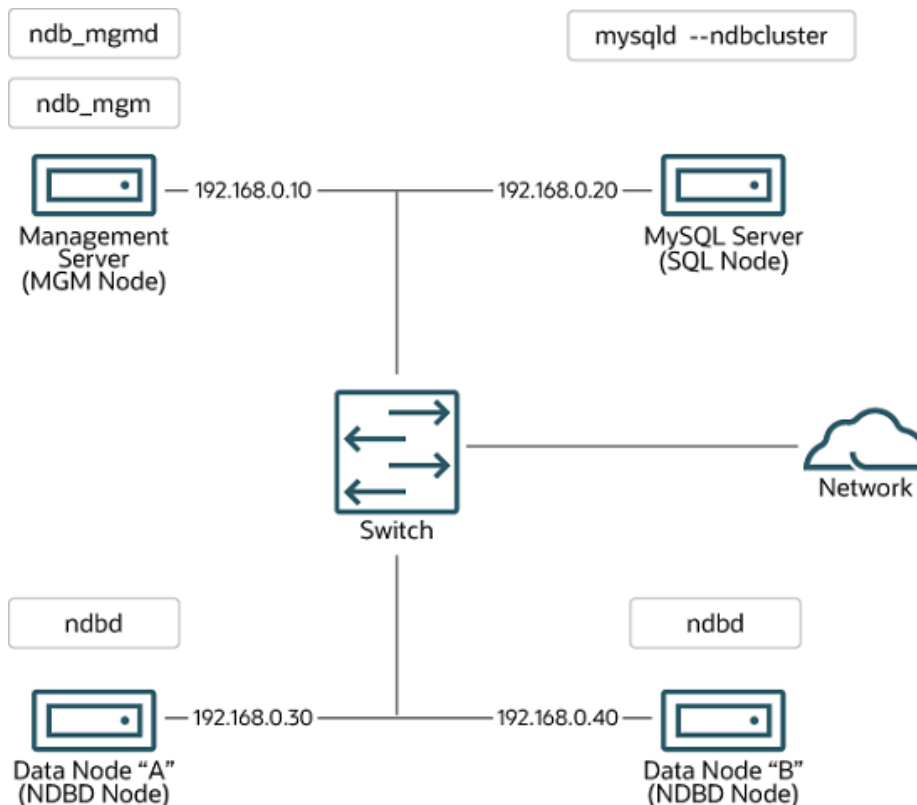
Figure 23.4 NDB Cluster Multi-Computer Setup
