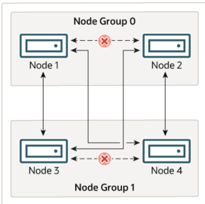
Figure 23.3 Nodes Required for a 2x2 NDB Cluster
