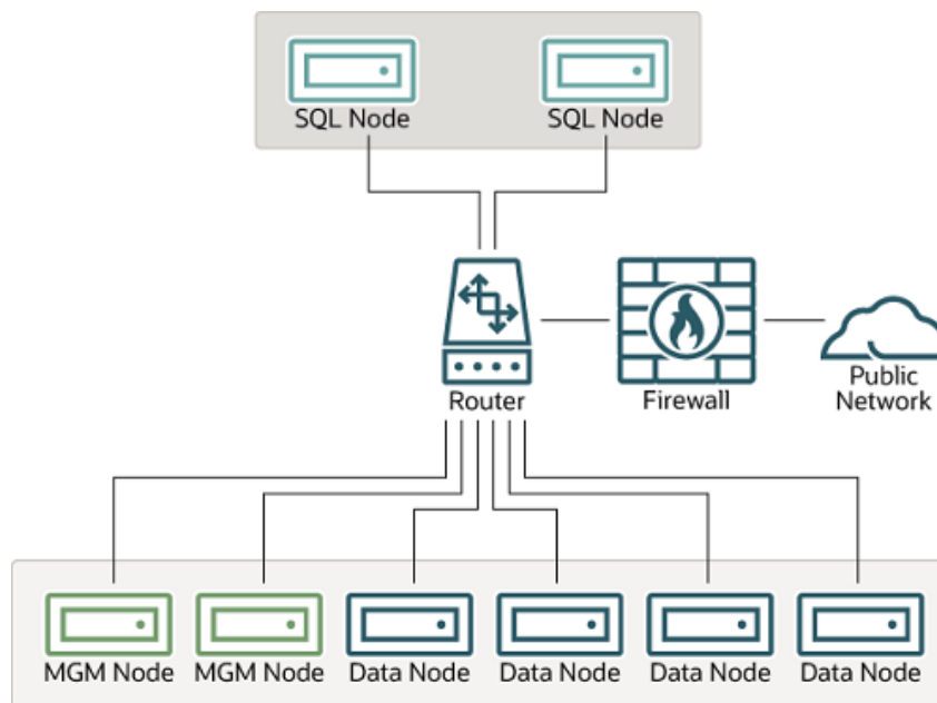
Figure 23.30 NDB Cluster with a Combination of Hardware and Software Firewalls
