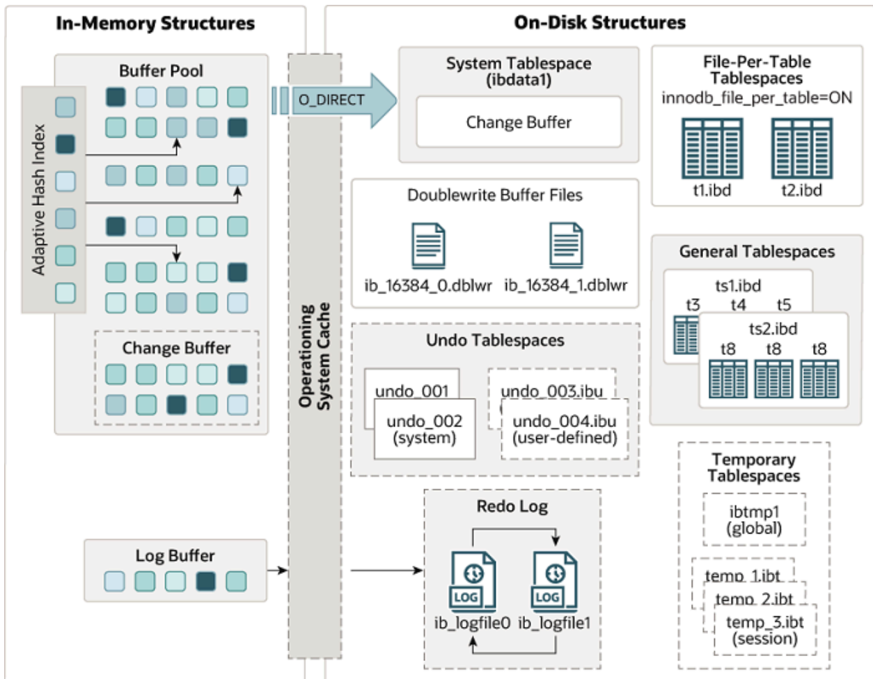
Figure 15.1 InnoDB Architecture
