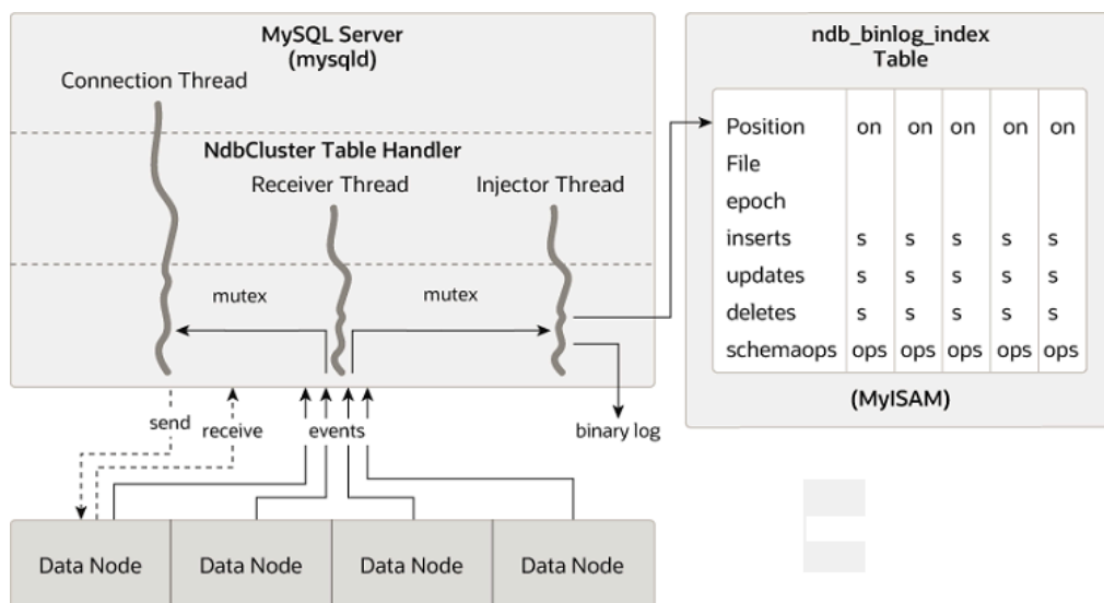
Figure 23.35 The Replication Source Cluster
