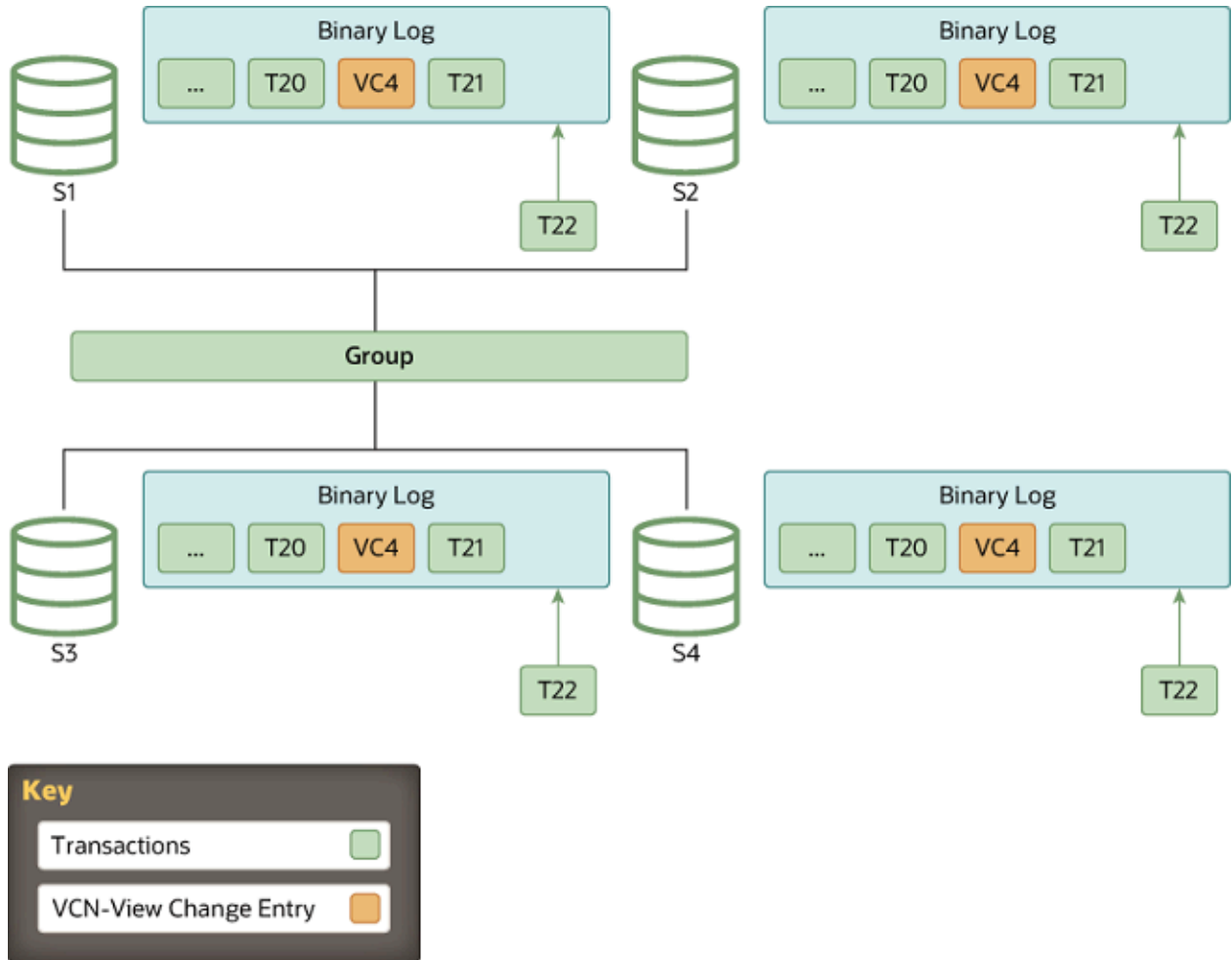
Figure 18.12 Instance Online
