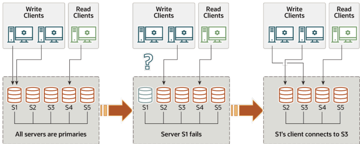
Figure 18.5 Client Failover
