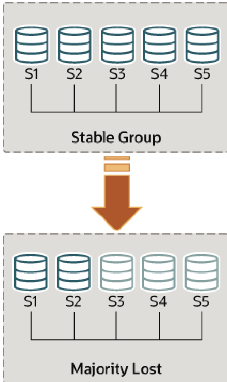
Figure 18.13 Losing Quorum
