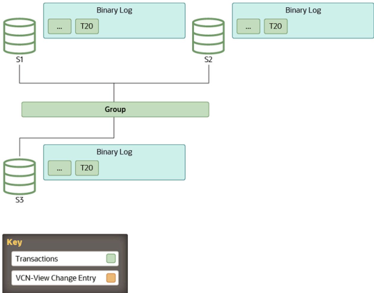
Figure 18.8 Stable Group
