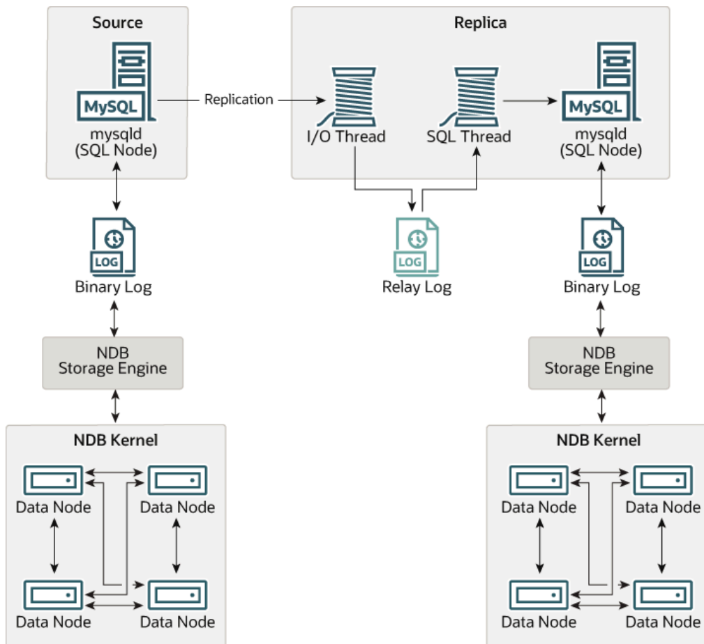
Figure 23.31 NDB Cluster-to-Cluster Replication Layout
