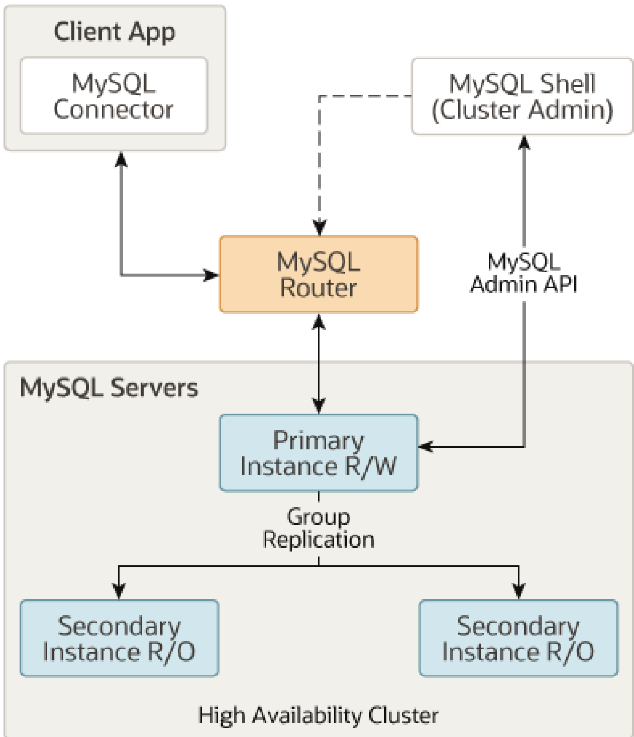
Figure 21.1 InnoDB Cluster overview
