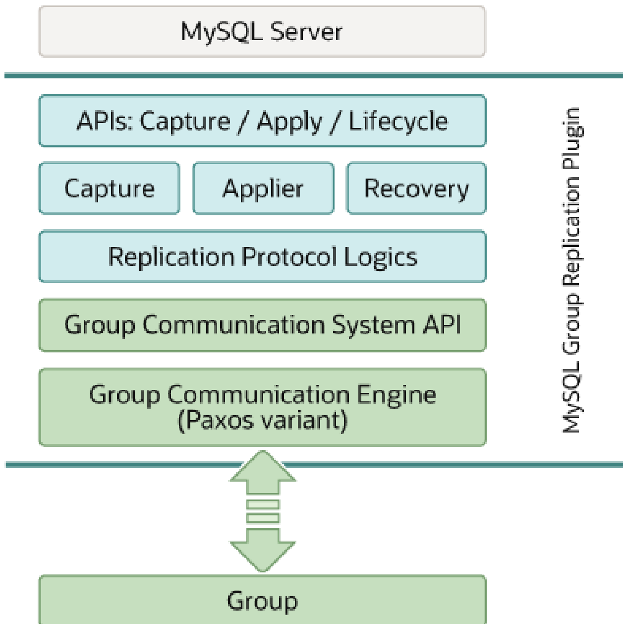
Figure 18.6 Group Replication Plugin Block Diagram
