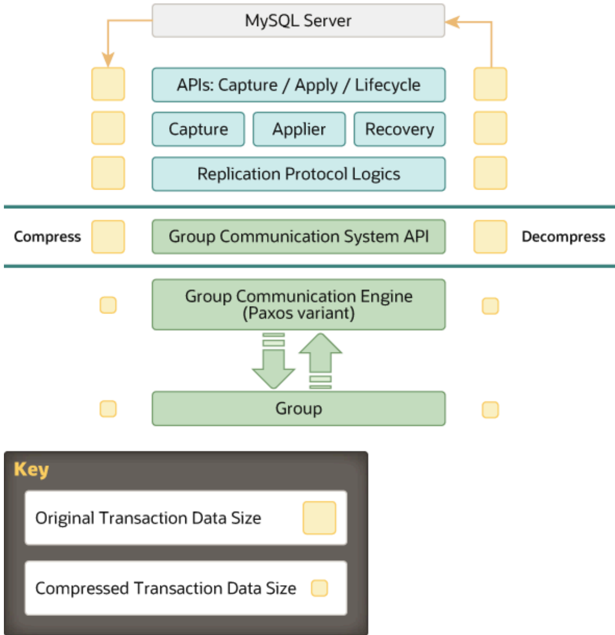
Figure 18.15 Compression Support
