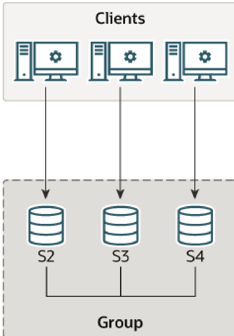
Figure 18.7 Group Architecture
