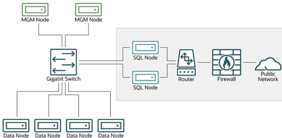
Figure 23.28 NDB Cluster with Hardware Firewall
