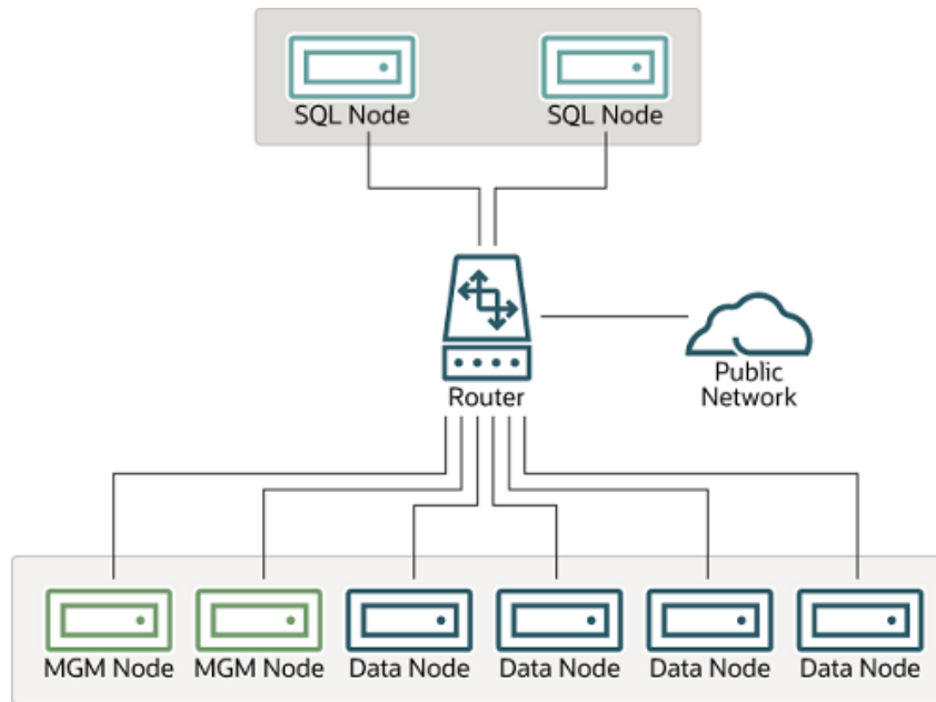
Figure 23.29 NDB Cluster with Software Firewalls
