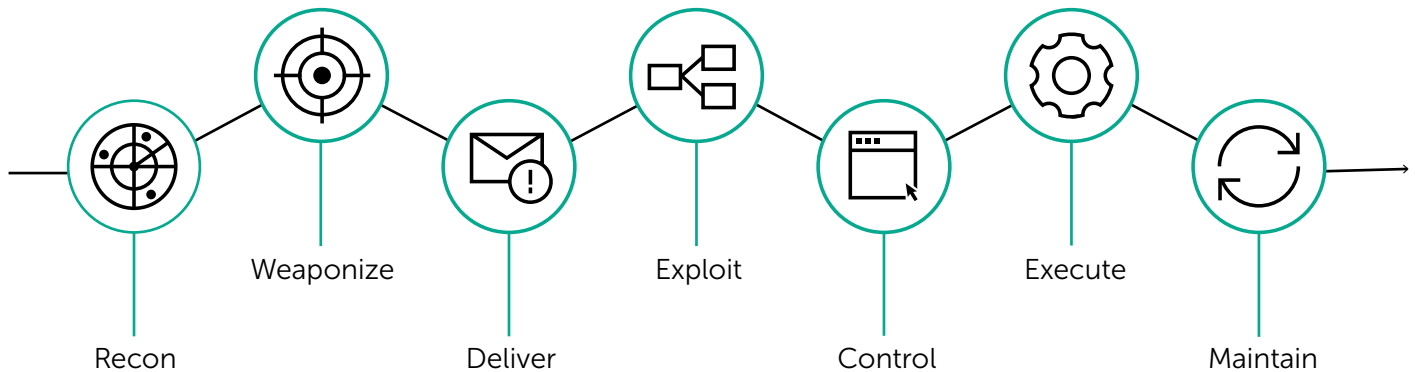
Figure 1: Adversary simulation
