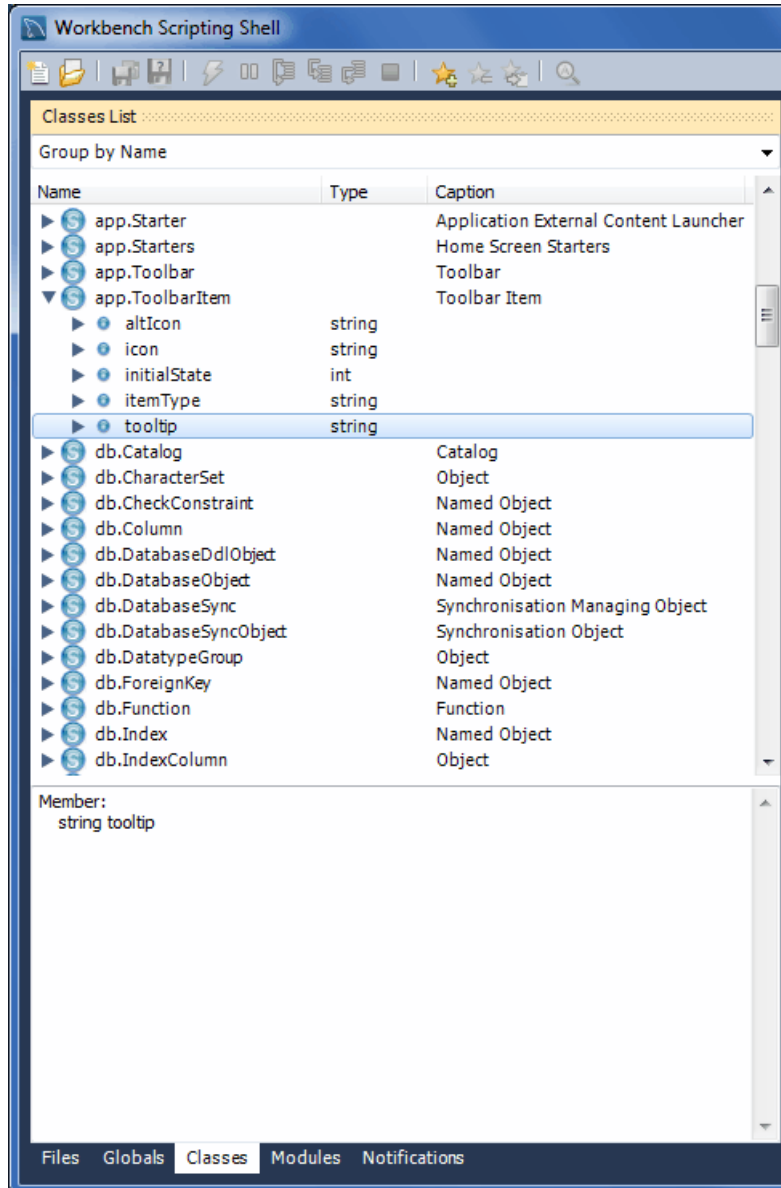
Figure C.5 The Workbench Scripting Shell Tab: Classes
