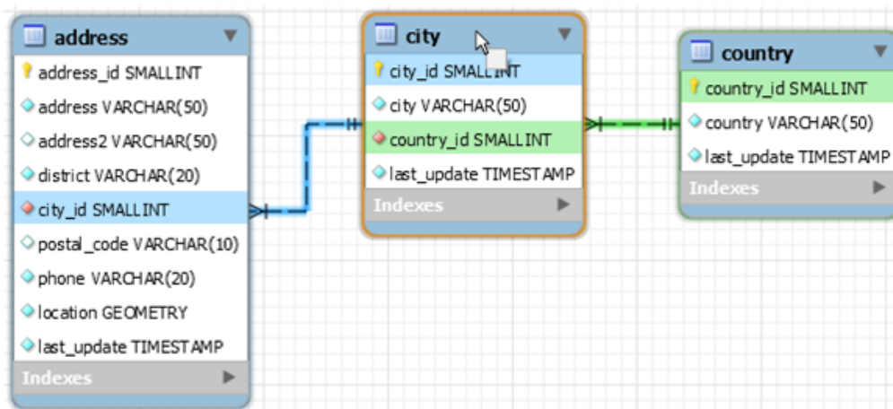
Figure 9.6 Enhanced Entity-Relationship Diagram
