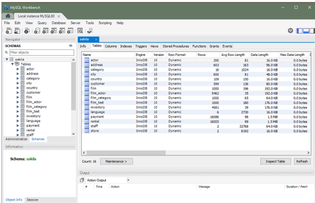
Figure 8.23 Schema Inspector
