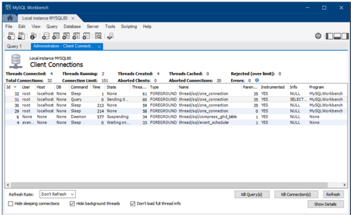
Figure 5.27 Client Connection Overview
