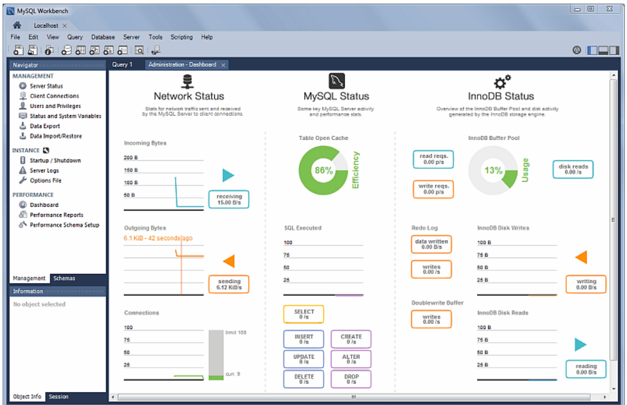
Figure 7.1 Performance: Dashboard
