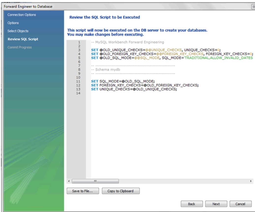
Figure 9.44 Review Script
