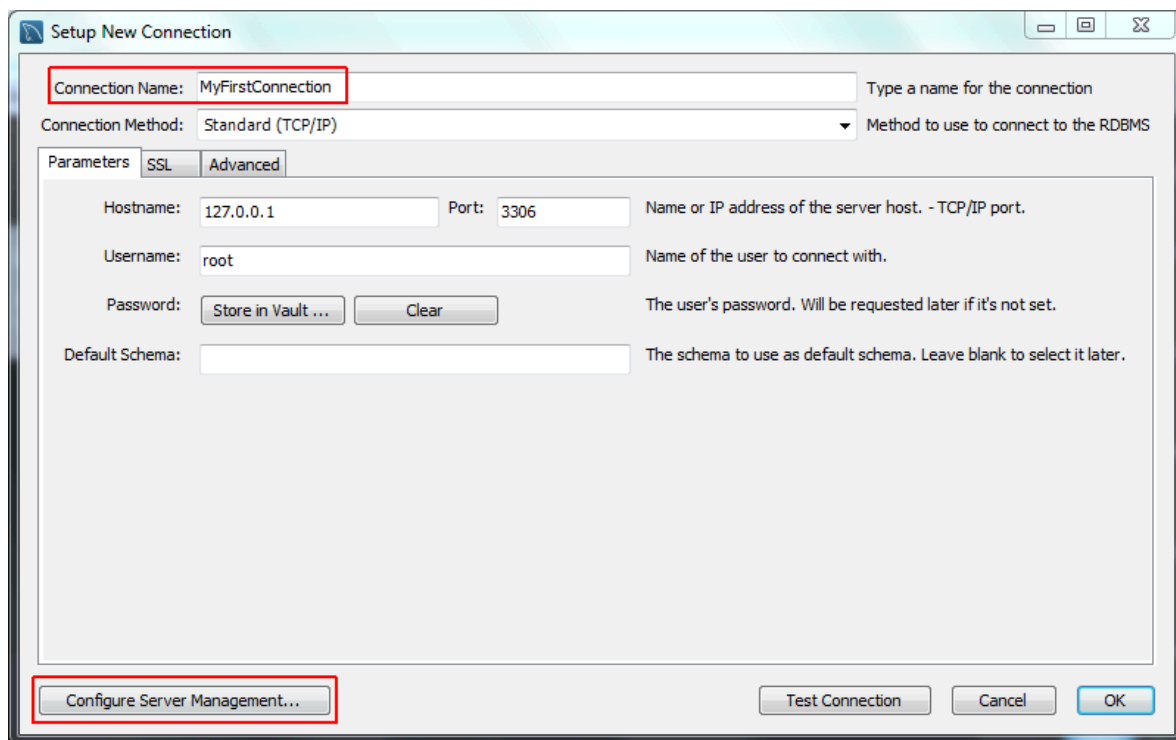
Figure 5.3 Getting Started Tutorial - Setup New Connection: MyFirstConnection
