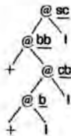
Annotated syntax tree
