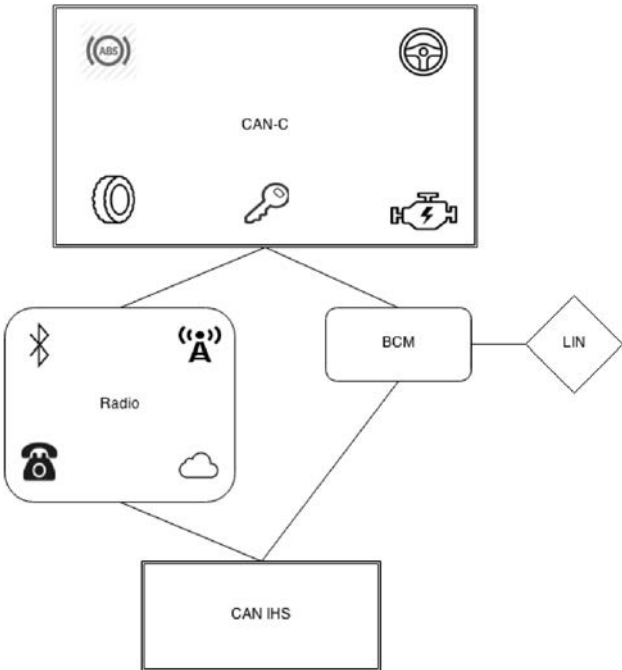
Figure 2. The Jeep Cherokee network architecture that the researchers Charlie Miller and Chris Valasek compromised in 2015
