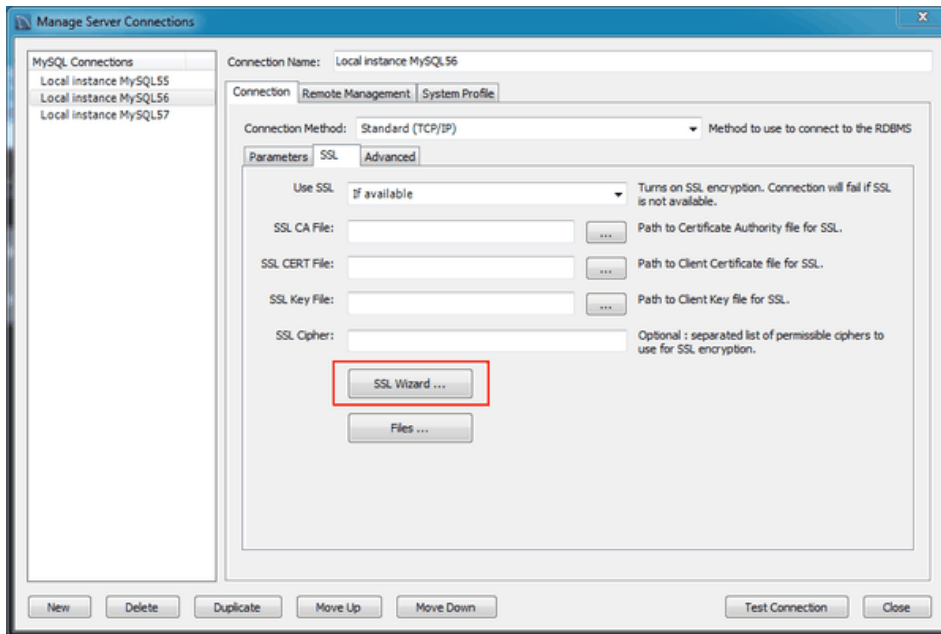
Figure 5.16 SSL Wizard: Start
