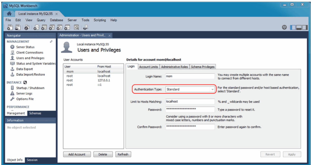
Figure 5.26 Upgraded Password: Standard (old) to Standard
