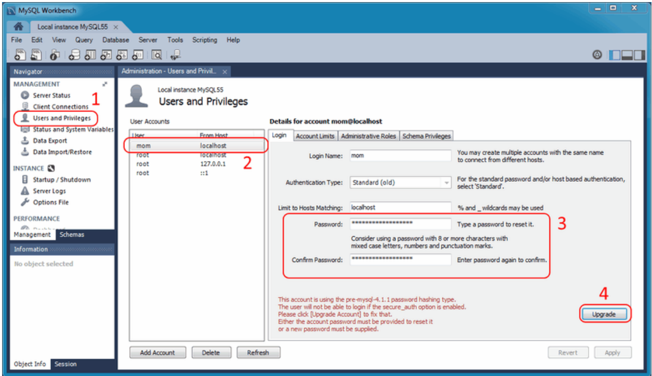
Figure 5.23 Upgrade Old Password: Setting a New Password
