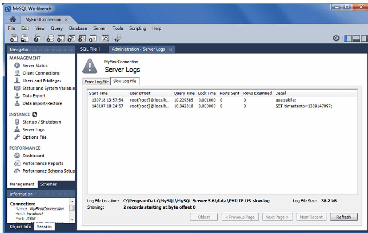
Figure 6.3 Navigator Management: Instance: Server Logs: Slow Log
