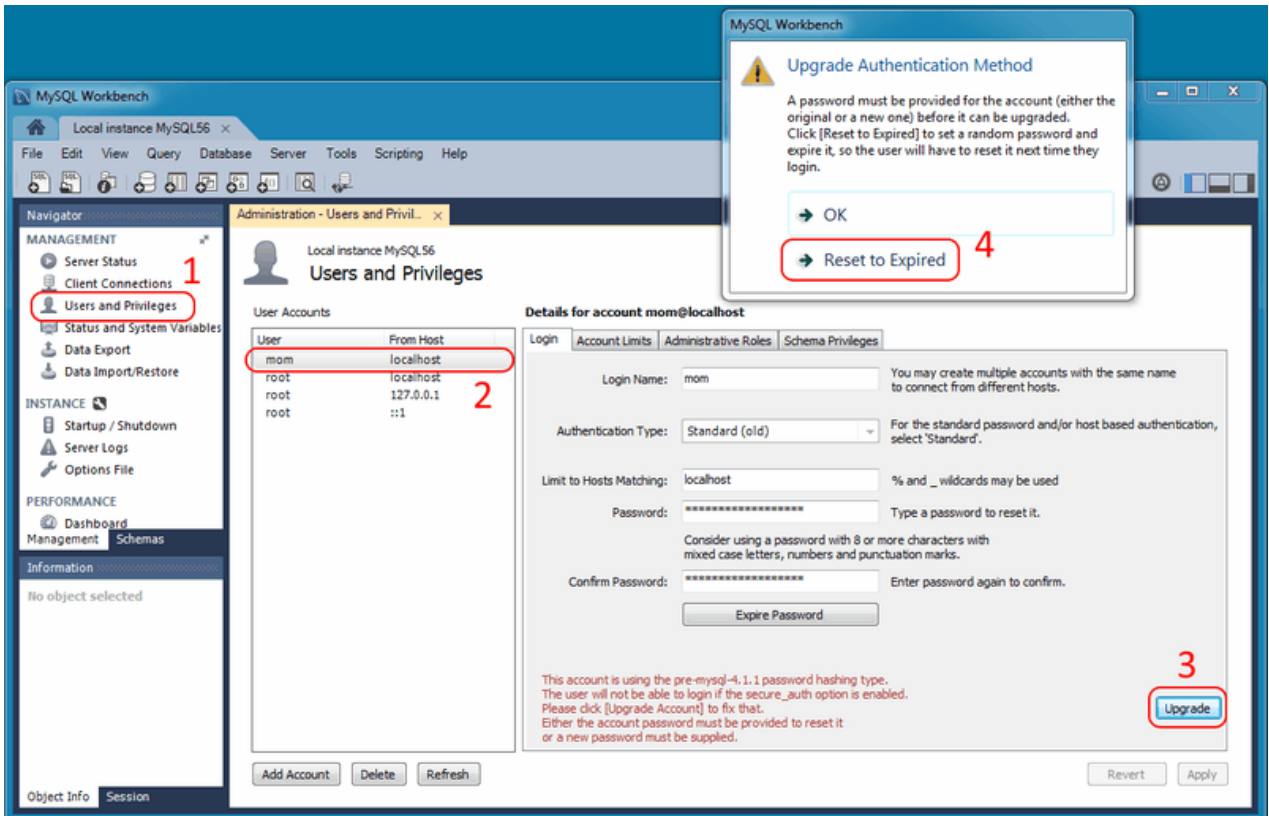
Figure 5.24 Upgrade Old Password: Reset to Random Expired Password
